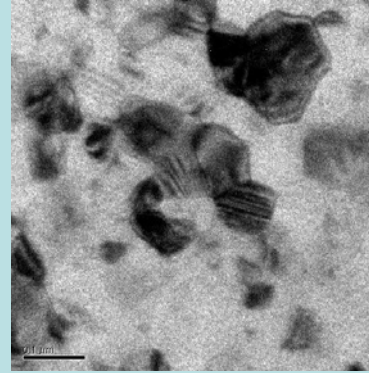
Twinned nc-Al grains (~50nm)
