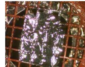
A specimen ready for in-situ straining in the TEM
