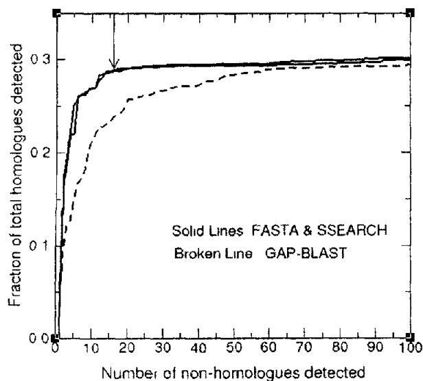
Figure 1 The performance of PDB_ISL with different pairwise search methods. The coverage is shown on the Y-axis as a fraction of the 6,964 SCOP evolutionary relationships in the PDB40D-1 database. The number of errors accumulated at increasing E-values is shown on the X-axis. The E-values at the arrow represent the coverage at 16 errors, a 1% error rate. The two solid lines are for FASTA and SSEARCH and the dotted line is for BLAST2.
