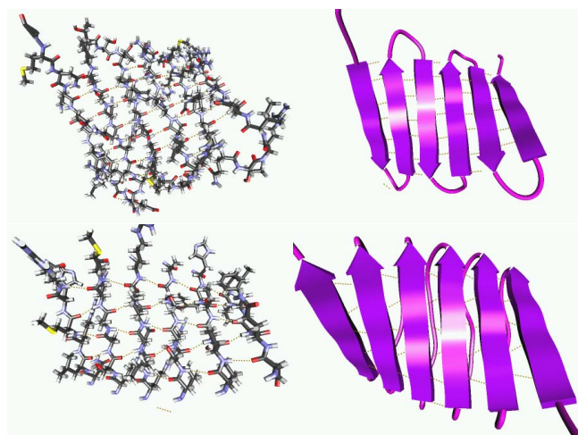
Figure 4: Two \beta -sheets. Hydrogen bonds stabilizing the sheets are shown as dashed yellow lines. Top row: anti-parallel sheet (left) and cartoon rendering (right). Bottom row: parallel sheet (left) and cartoon rendering (right).
