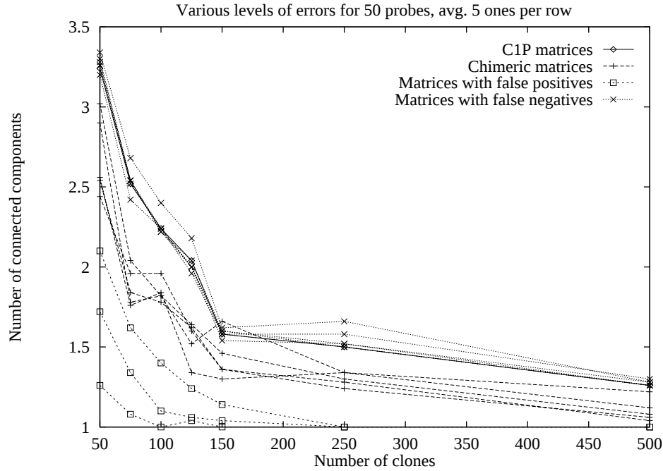
Figure 5: Number of connected components for varied data
