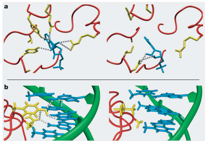
Figure 2 | Molecular structures in different evolutionary forms. Main chains are shown in red, key residues in yellow, the DNA backbone in green, key DNA bases or cofactor in blue, and hydrogen bonds as dashed lines. a , The left panel shows wild-type E. coli isocitrate dehydrogenase 34 (IDH), which is structurally similar to IMDH, with NADP as cofactor. The right panel shows an engineered IDH form with NAD as cofactor 35 . b , The left panel shows a wild-type E. coli lac repressor and operator 36 . The right panel shows a lac repressor and operator variant, with mutations mimicking the gal system 37 . Binding is tight and specific (despite the absence of hydrogen bonds): these variants bind wild-type partners poorly. Figures prepared with MOLMOL 38 .
