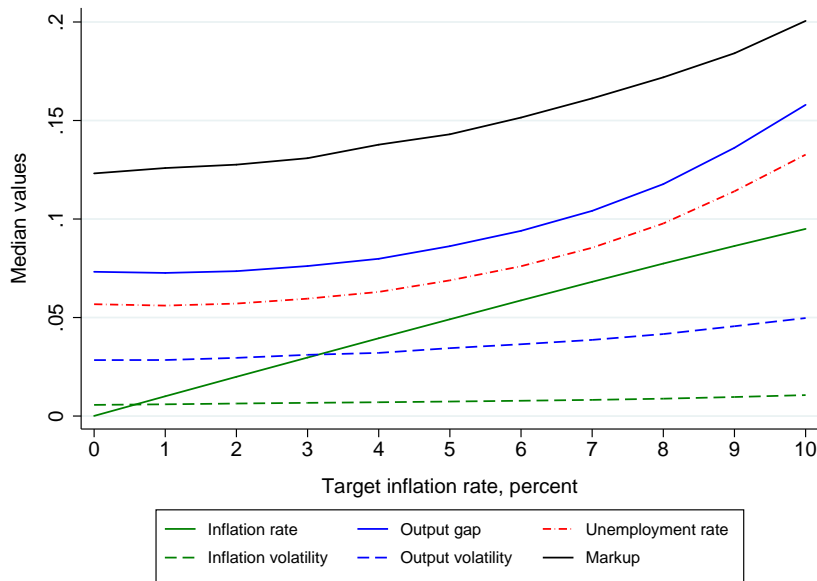
FIGURE 5: The main results under endogenous markups
