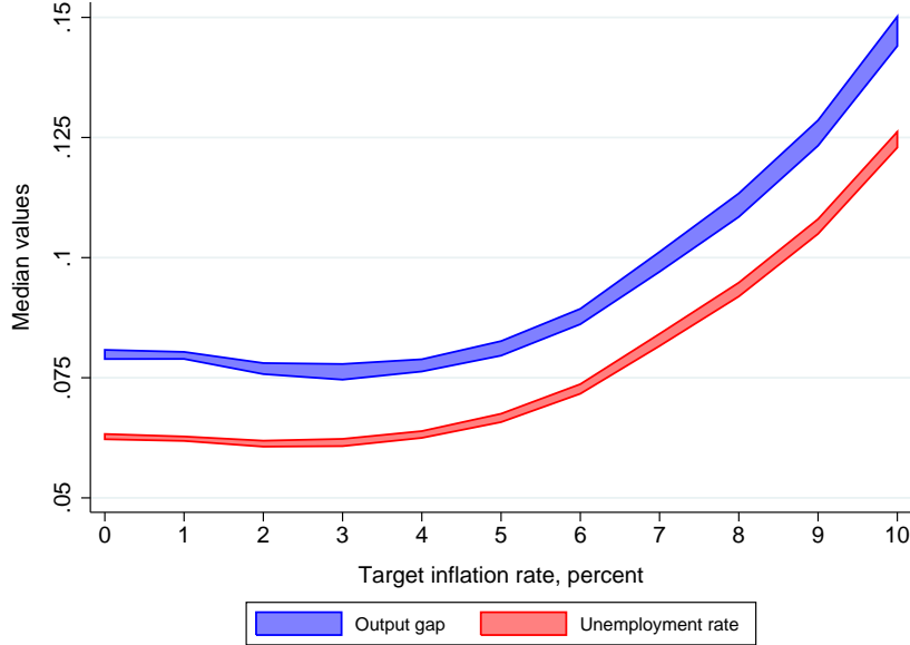
FIGURE 2: Statistical significance of the main results
