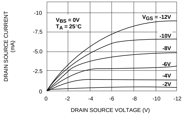
OUTPUT CHARACTERISTICS
