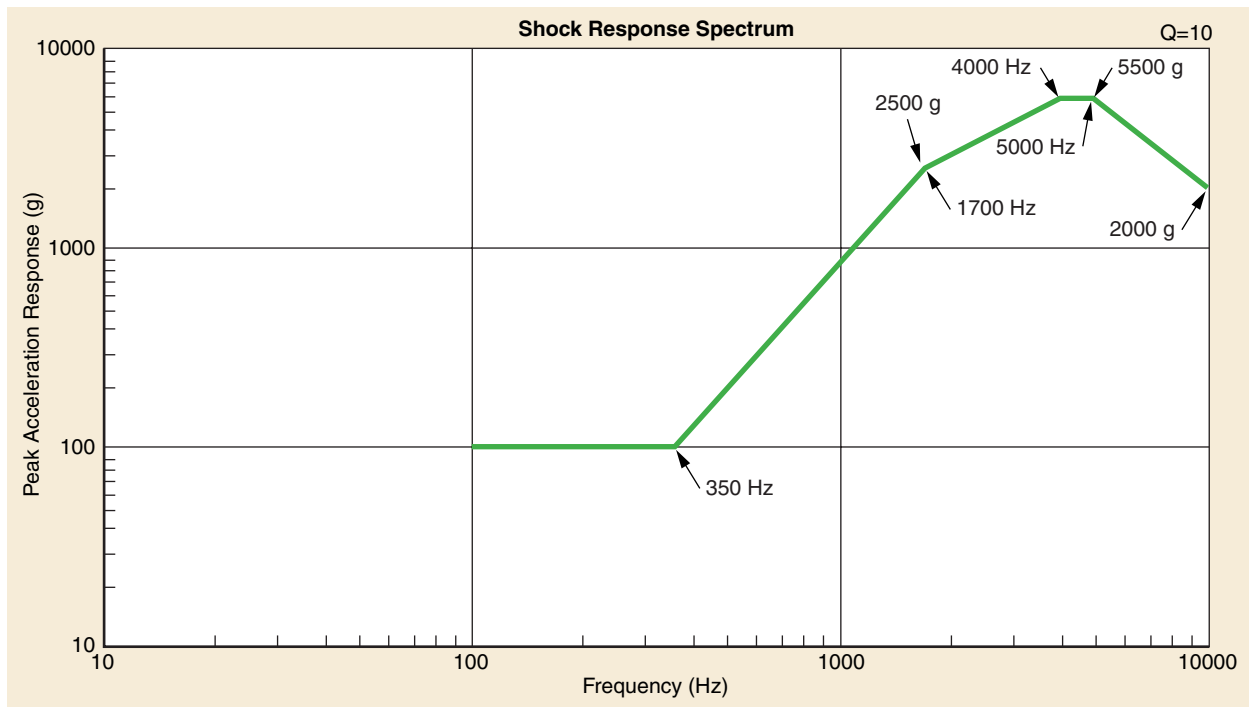
Figure 4-24. Maximum Flight Spacecraft Interface Shock Environment 6019 and 6915 Payload Attach Fitting
