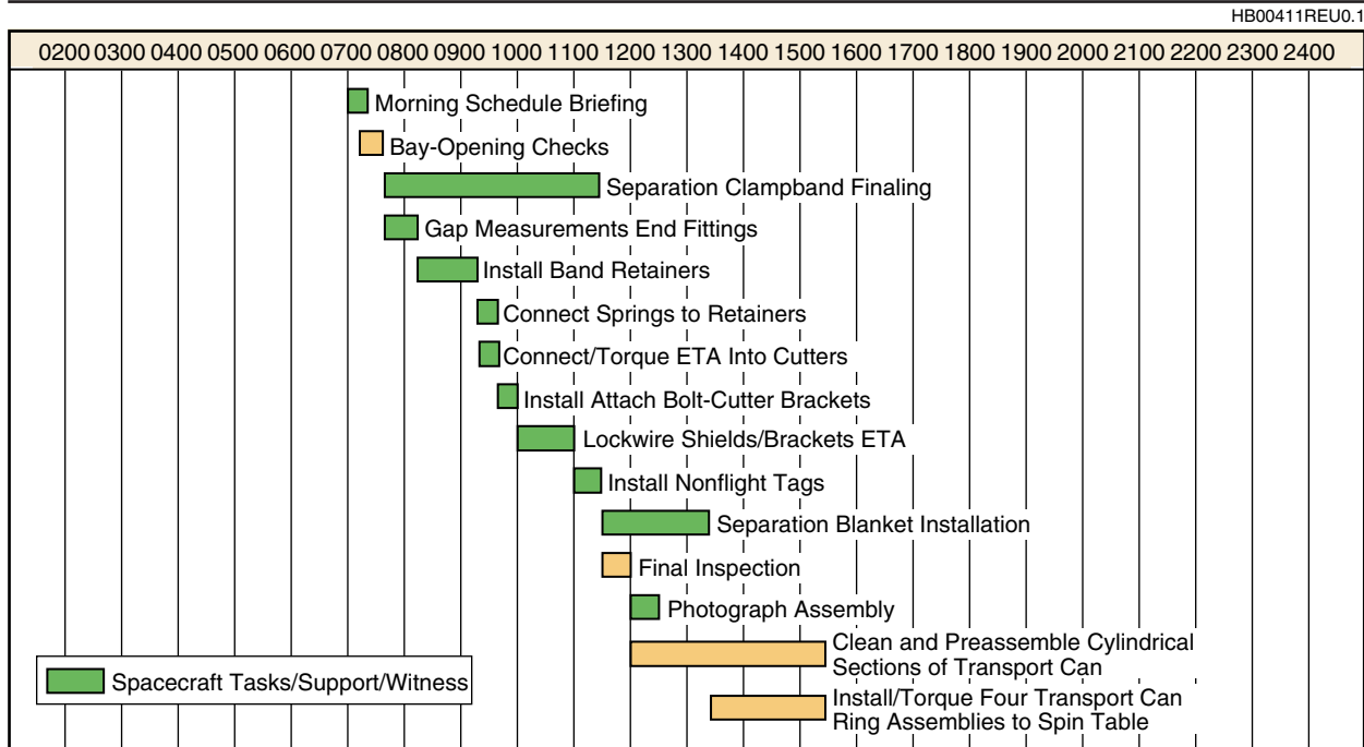
Figure 6-29. Typical Final Spacecraft Third-Stage Preparations (T-9 Day)
