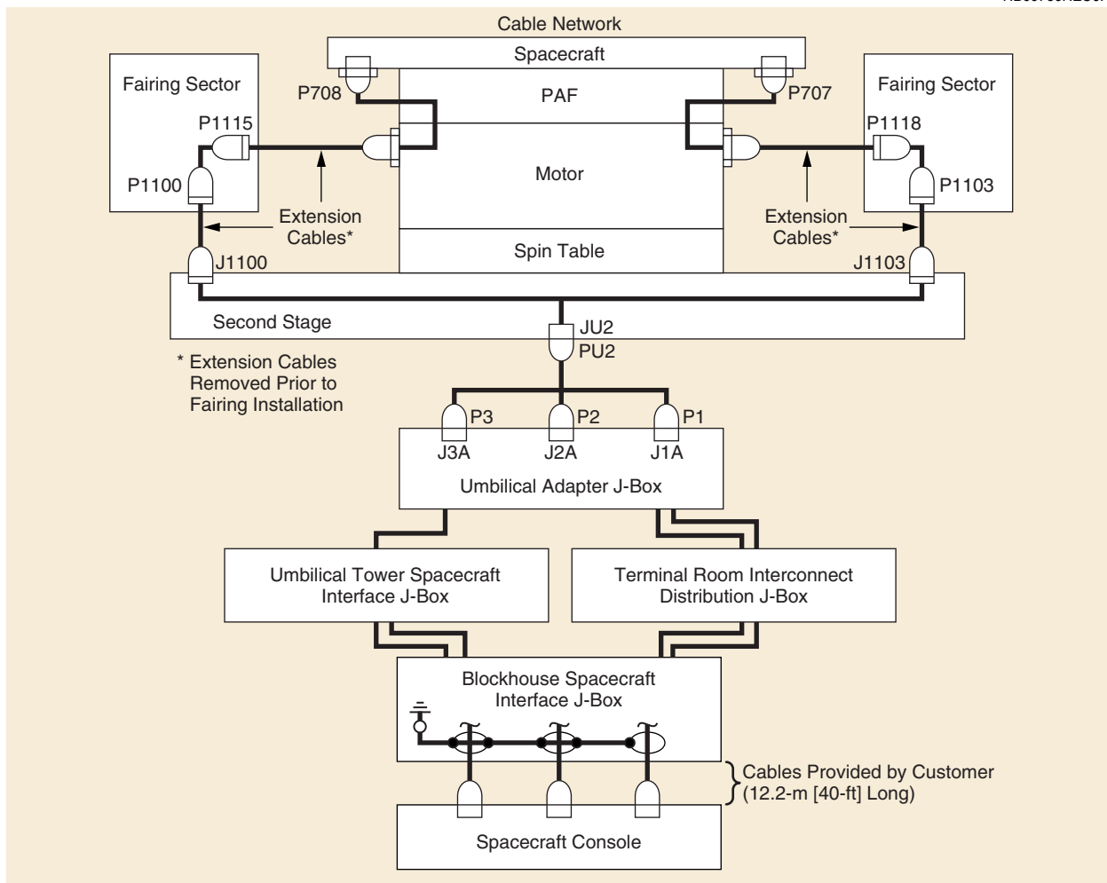
Figure 5-61. Typical Payload-to-Blockhouse Wiring Diagram for Three-Stage Missions at SLC-17
