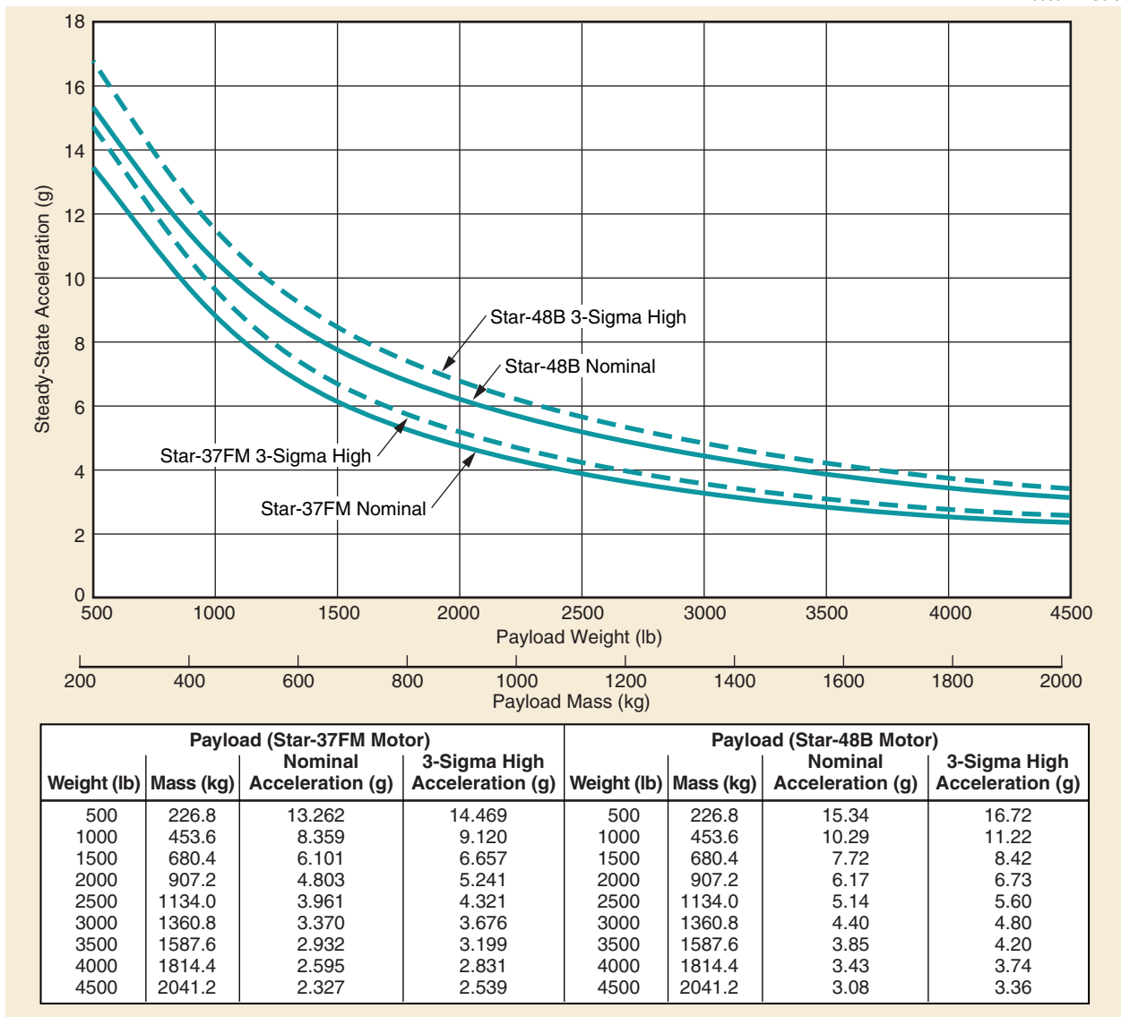
Figure 4-19. Axial Steady-State Acceleration vs. Payload Weight at Third-Stage Burnout
