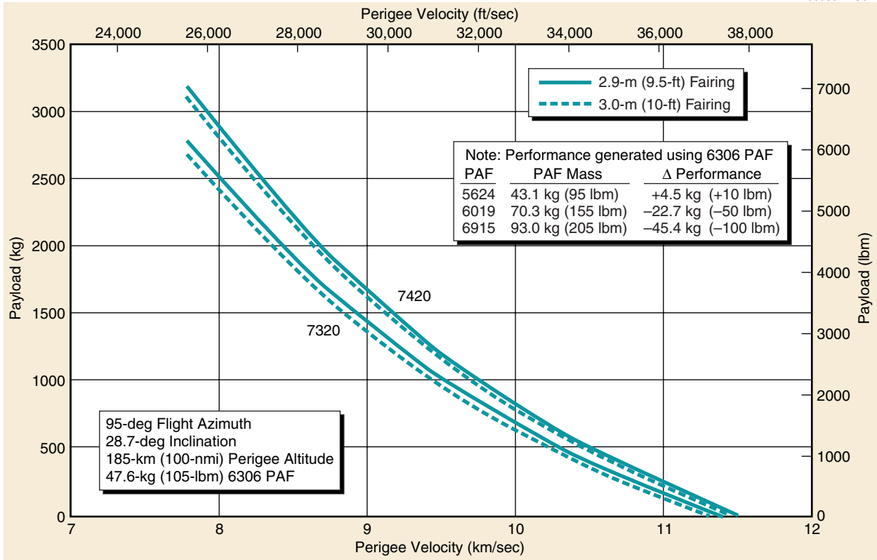
Figure 2-7. Delta II 7320/7420 Vehicle, Two-Stage Perigee Velocity Capability—ER Launch Site
