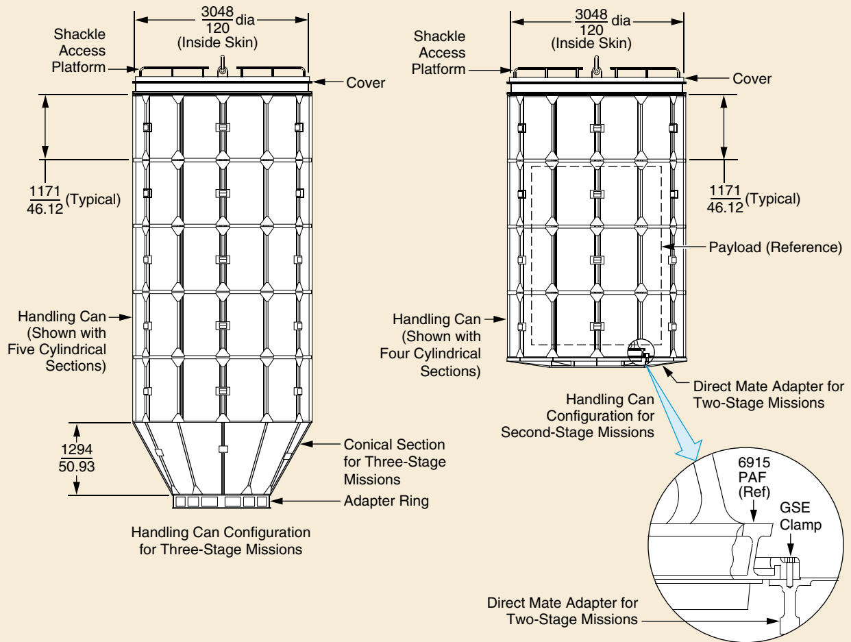
Figure 6-14. Delta II Upper-Stage Assembly Ground-Handling Can and Transporter
