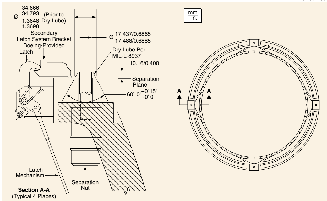
Figure 5-31. 6915 PAF Detailed Dimensions
