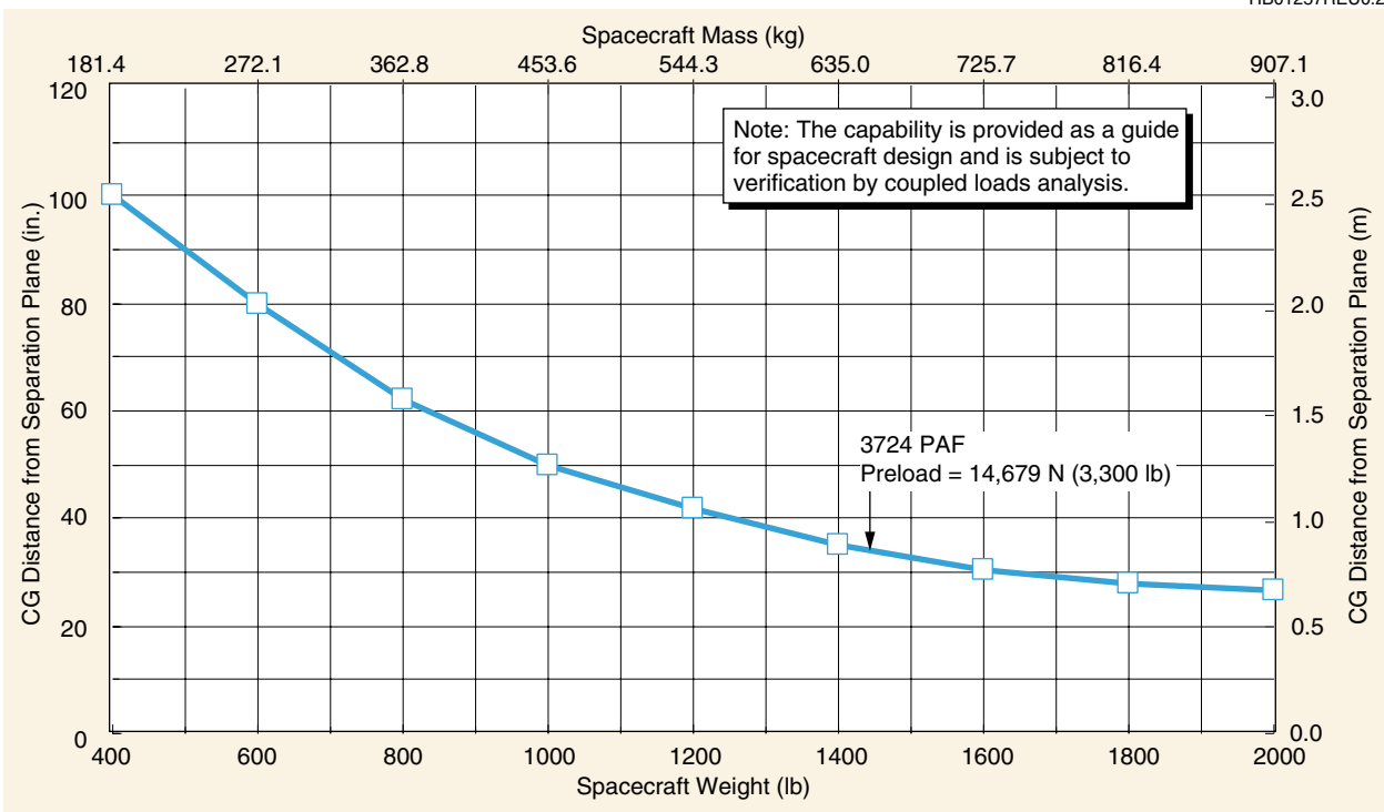
Figure 5-6. Capability of 3724 PAF
