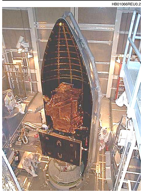
Figure 3-6. 3-m (10-ft) dia Composite Fairing
