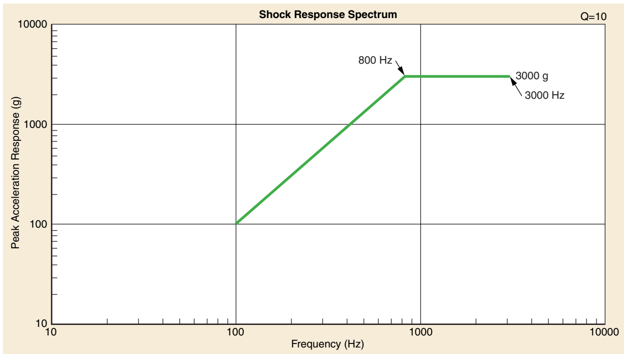
Figure 4-23. Maximum Flight Spacecraft Interface Shock Environment 6306 Payload Attach Fitting
