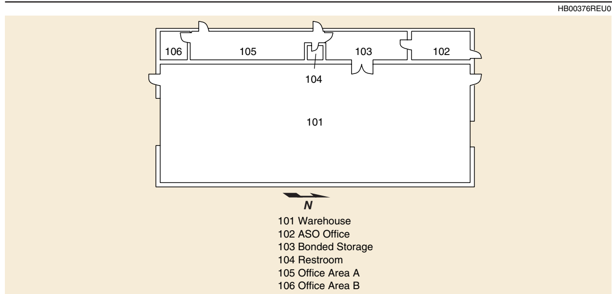
Figure 6-9. Building 4 Detailed Floor Plan, Astrotech
