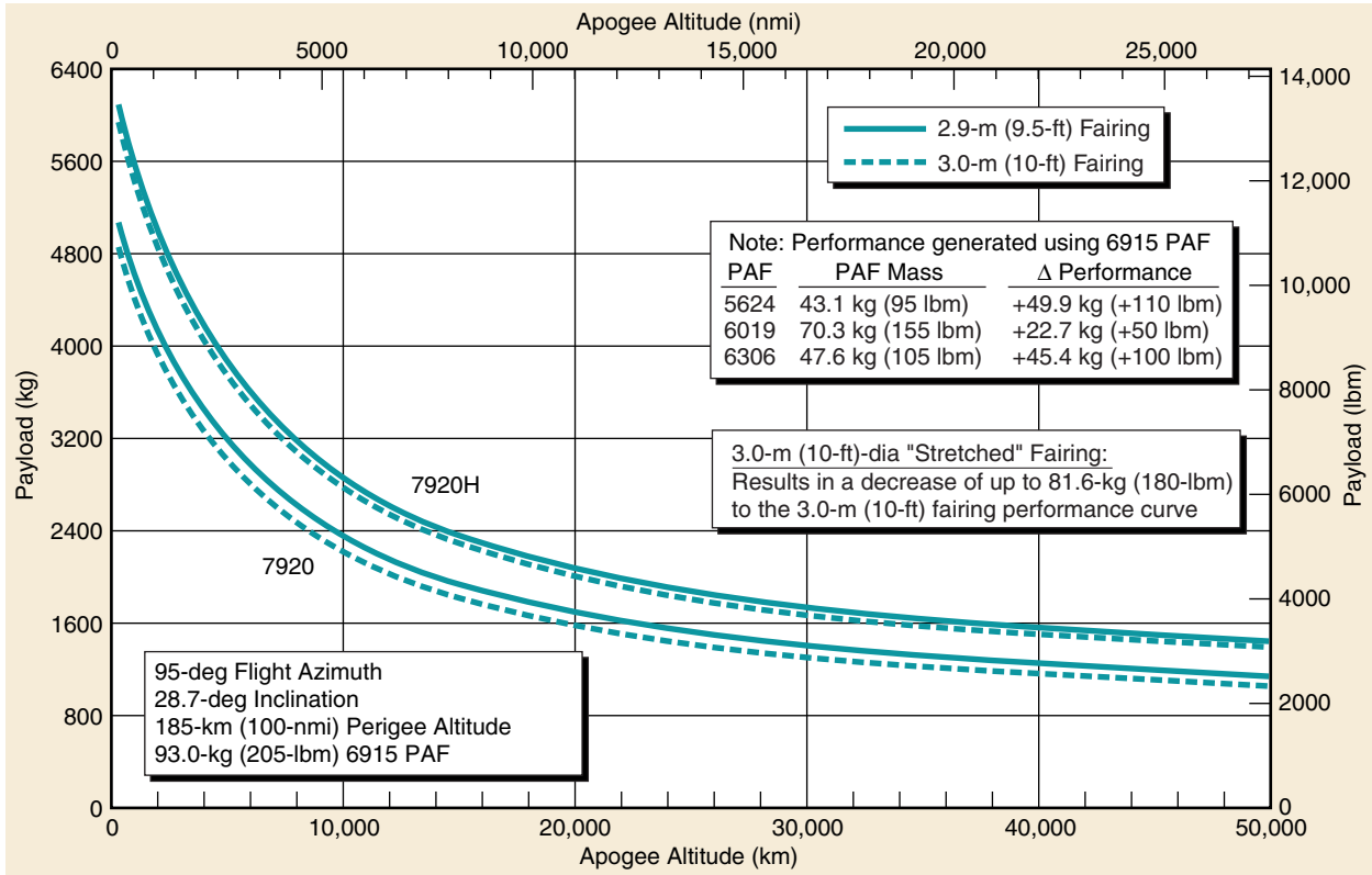
Figure 2-21. Delta II 7920/7920H Vehicle, Two-Stage Apogee Altitude Capability—Eastern Launch Site
