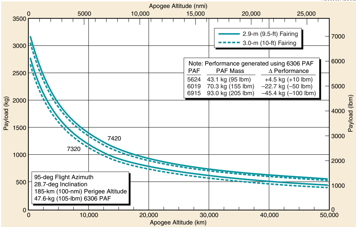
Figure 2-8. Delta II 7320/7420 Vehicle, Two-Stage Apogee Altitude Capability—ER Launch Site
