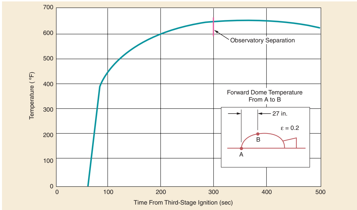
Figure 4-17. Star-37FM Motor Case Temperature
