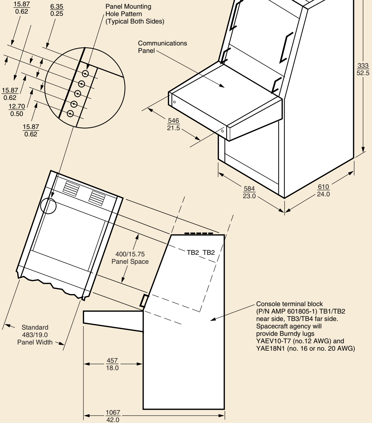
Figure 7-32. Spacecraft Blockhouse Console—Western Range
