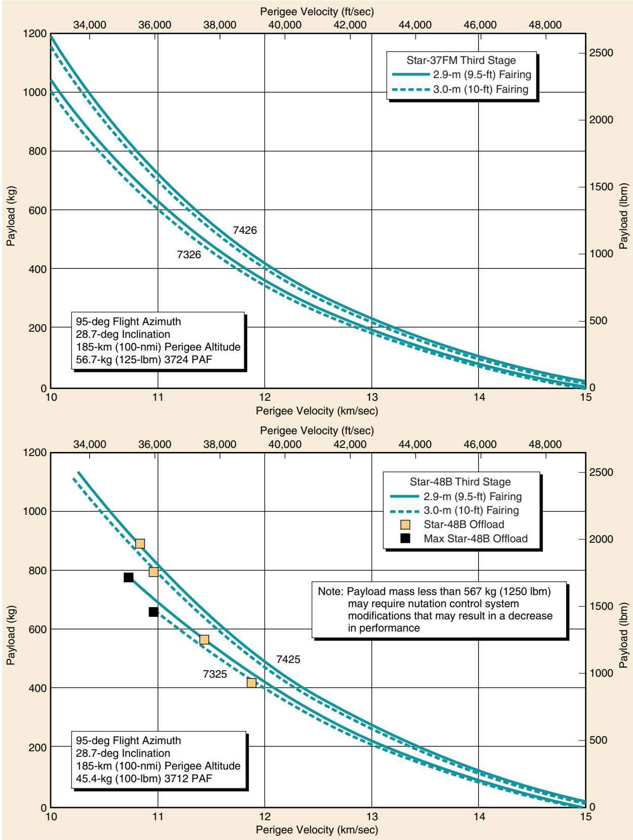
Figure 2-10. Delta II 732X/742X Vehicle, Three-Stage Perigee Velocity Capability—Eastern Launch Range
