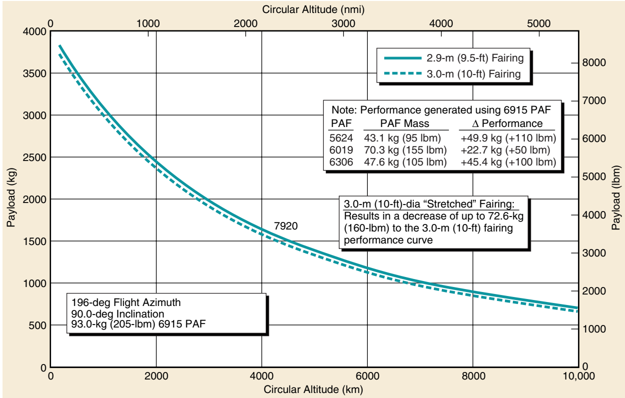
Figure 2-29. Delta II 7920 Vehicle, Two-Stage Circular Orbit Altitude Capability—Western Launch Site
