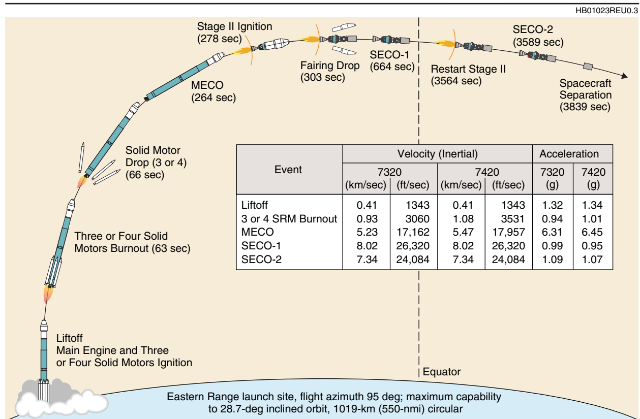
Figure 2-3. Typical Delta II 7320/7420 Mission Profile—Circular Orbit Mission (ER Launch Site)
