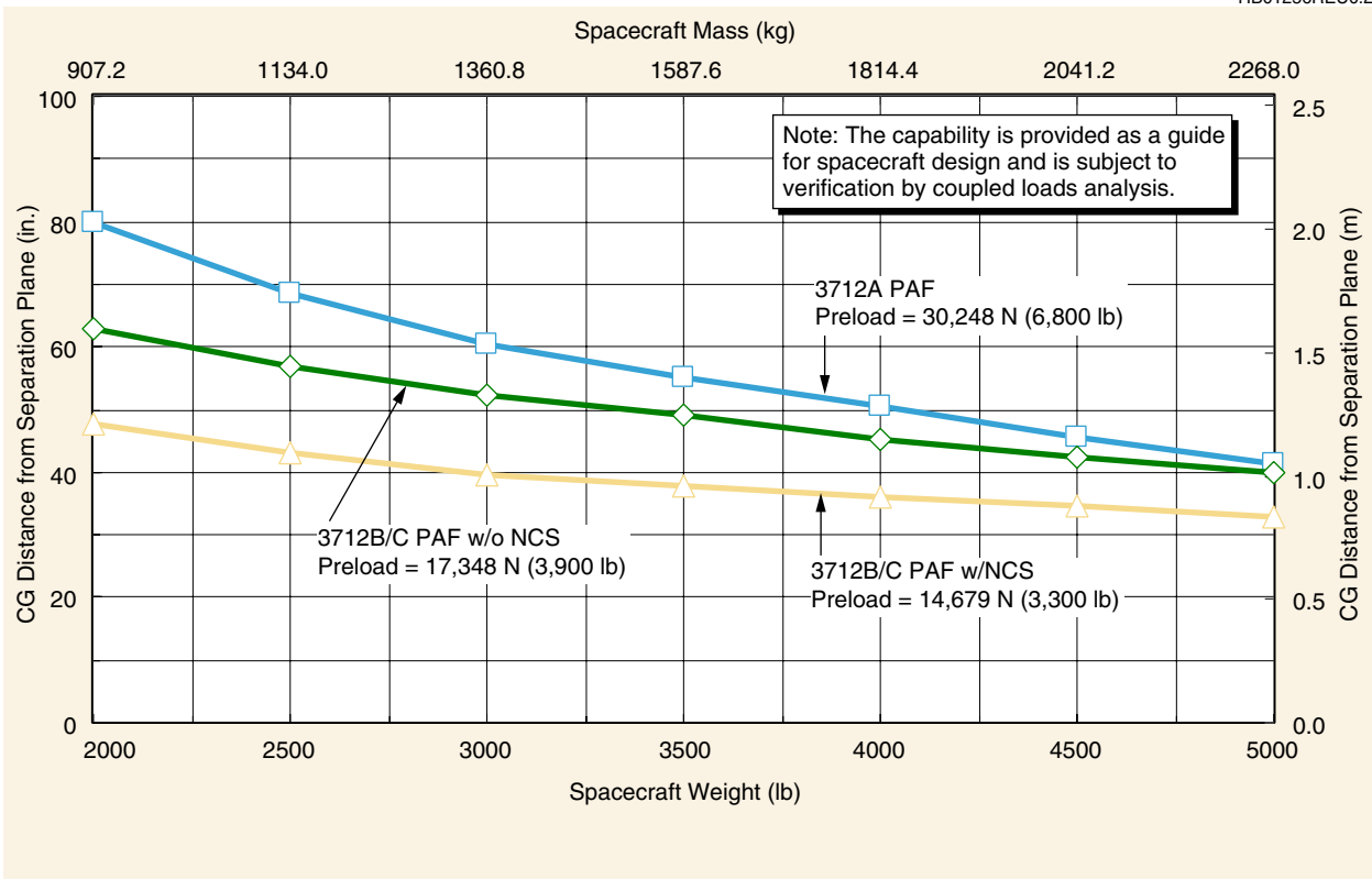
Figure 5-5. Capability of 3712 PAF
