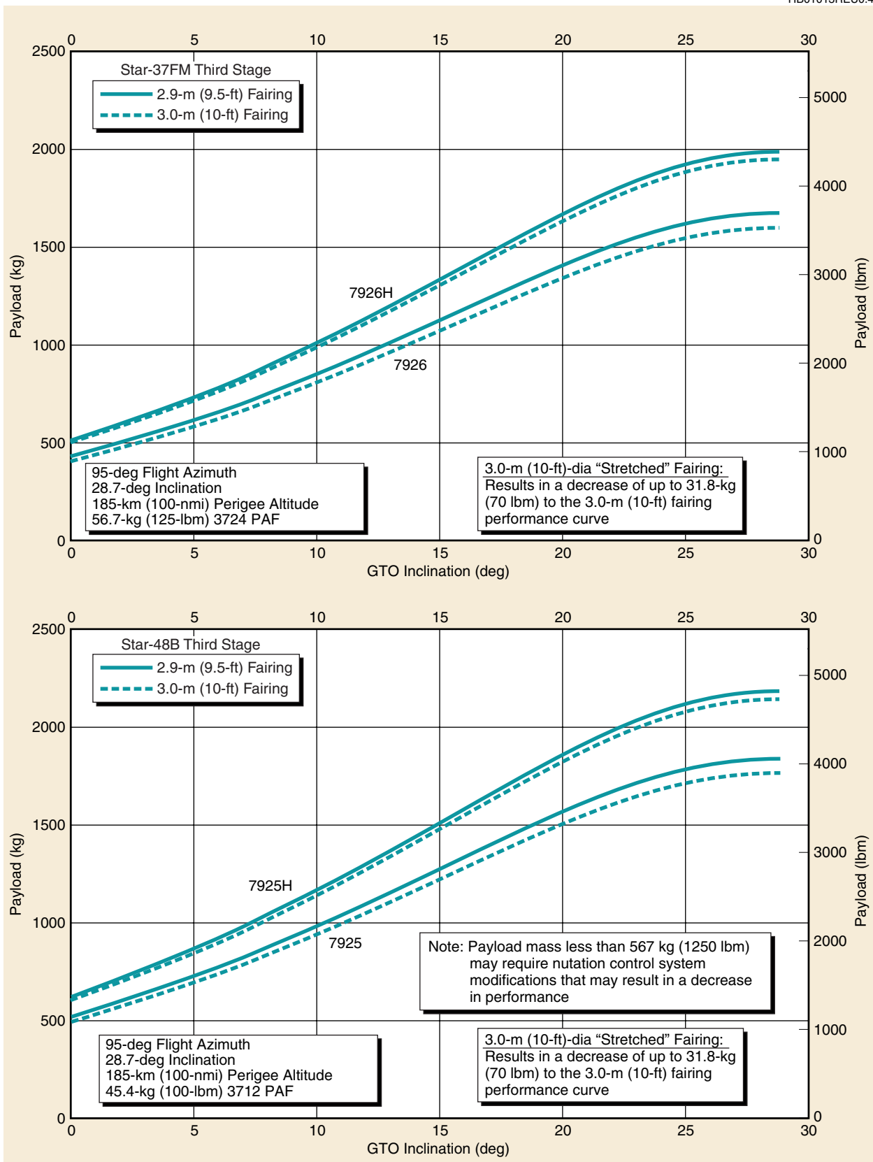
Figure 2-25. Delta II 792X/792XH Vehicle, Three-Stage GTO Inclination Capability—Eastern Launch Site
