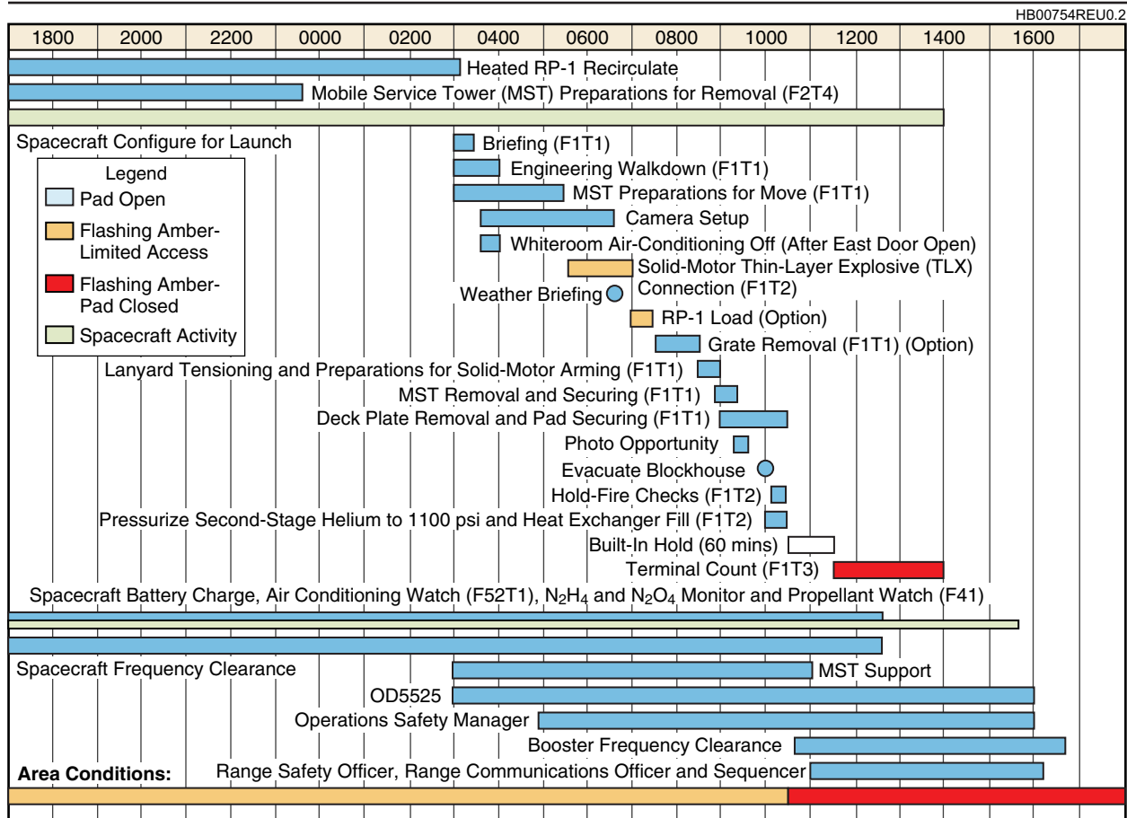
Figure 6-38. Typical Delta Countdown (T-0 Day)
