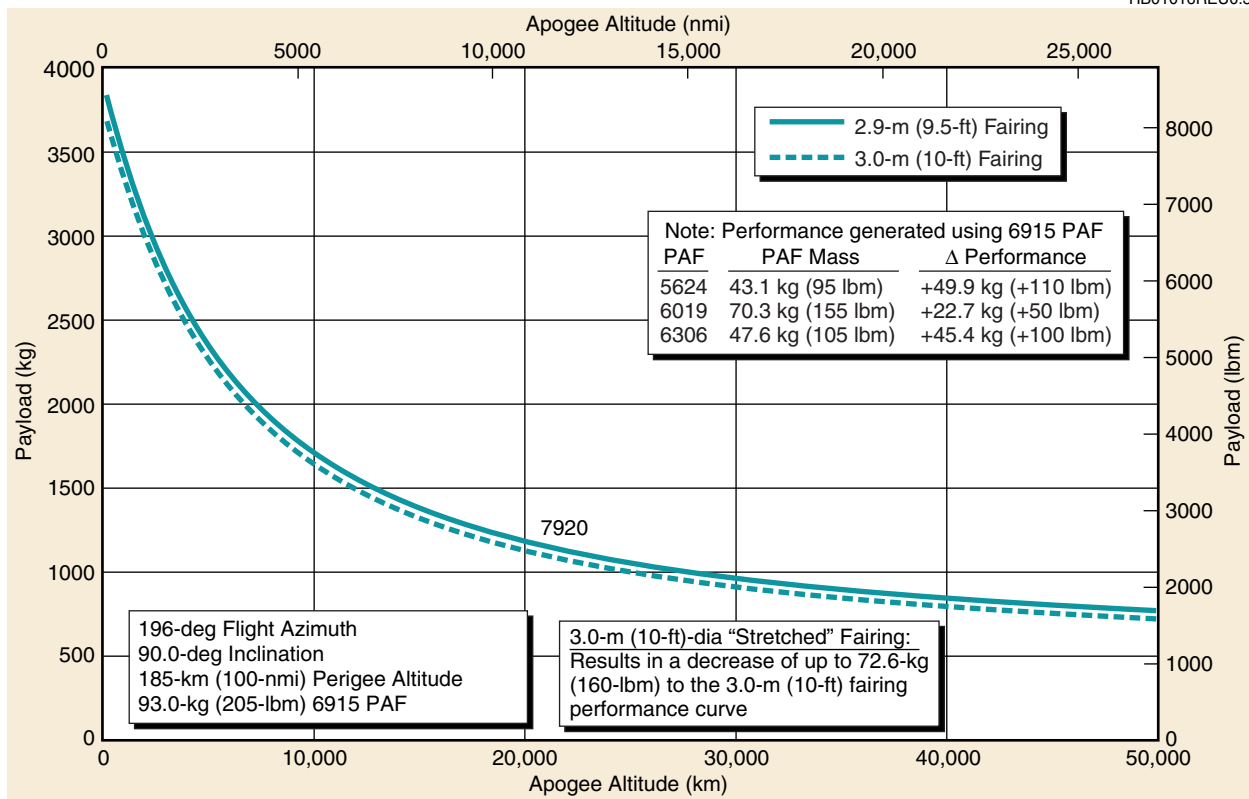
Figure 2-28. Delta II 7920 Vehicle, Two-Stage Apogee Altitude Capability—Western Launch Site
