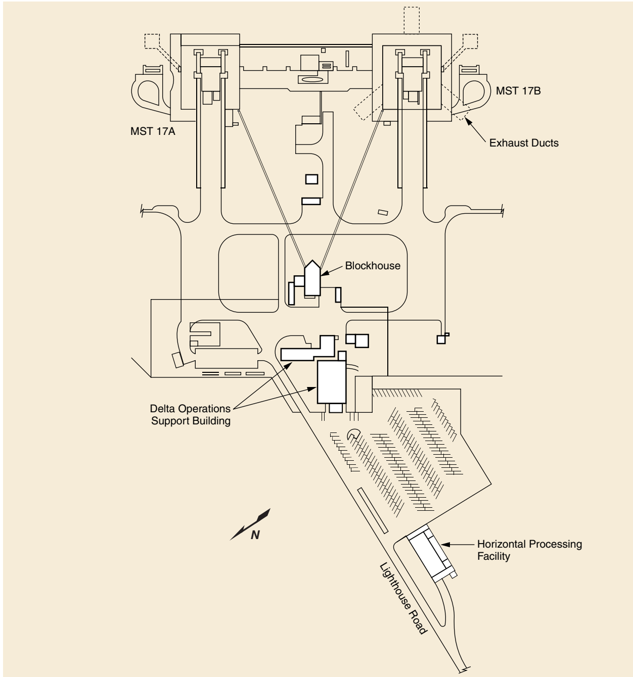
Figure 6-16. Space Launch Complex-17, Cape Canaveral Air Force Station
