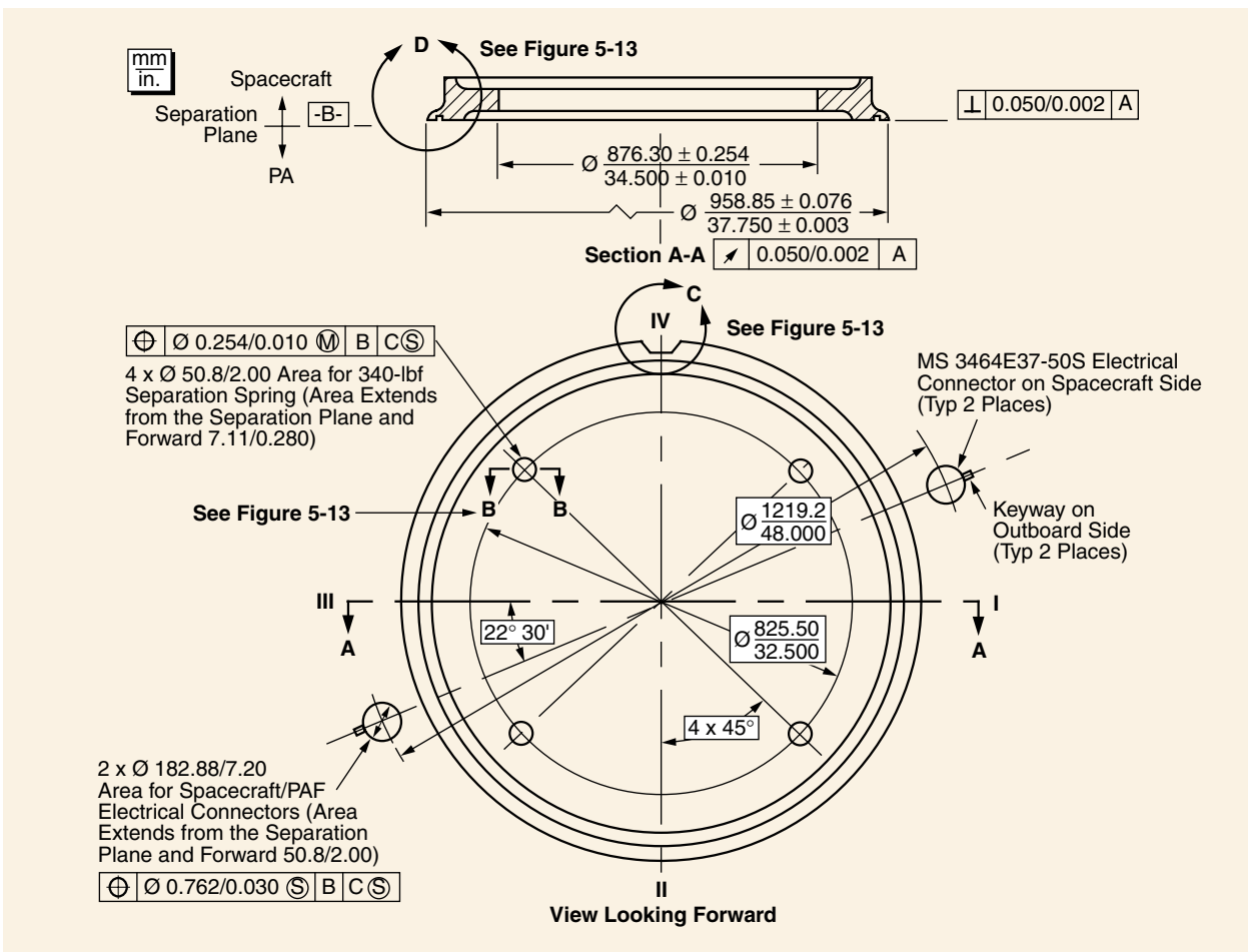
Figure 5-12. Dimensional Constraints on Spacecraft Interface to 3712B PAF
