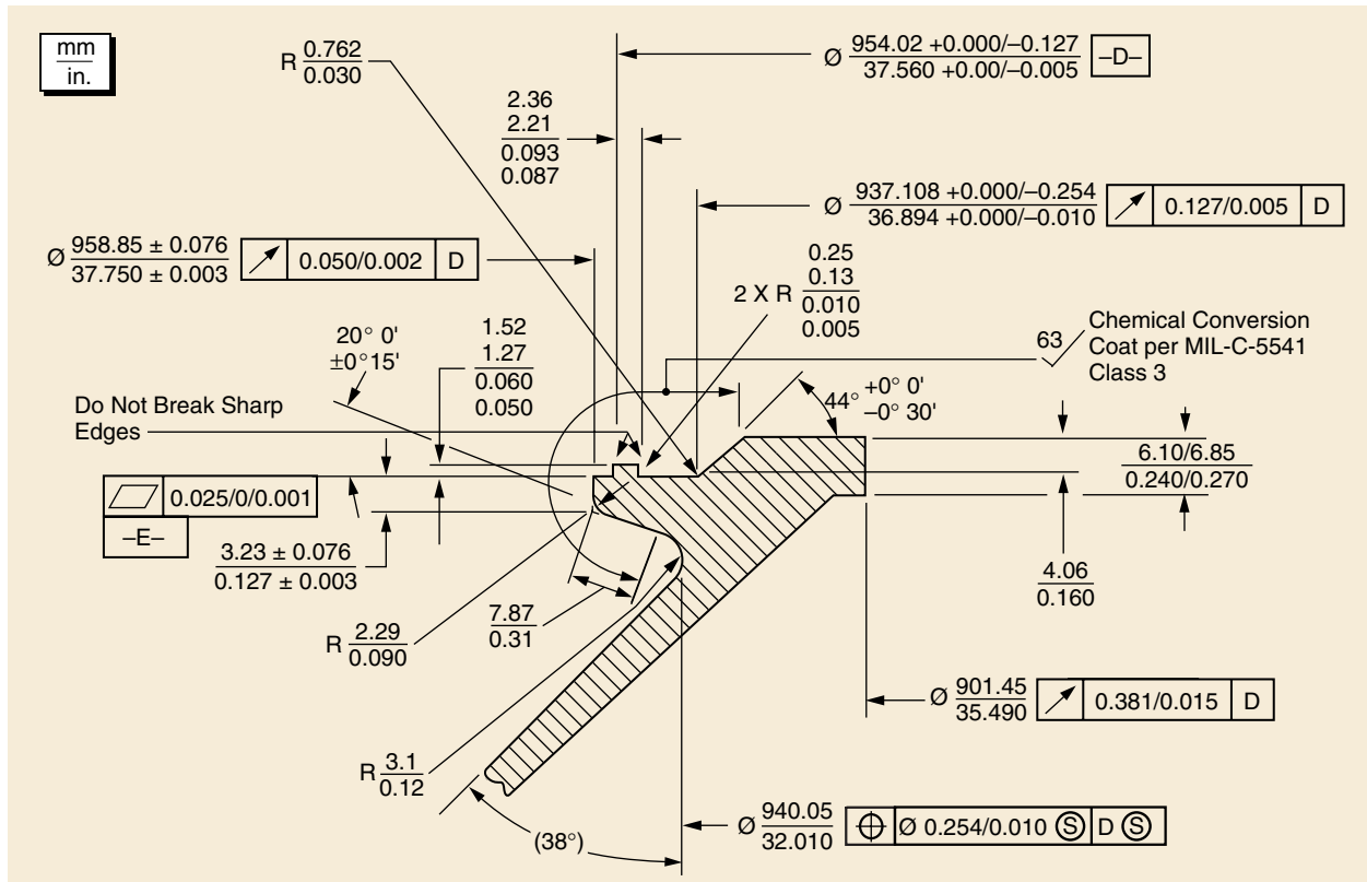
Figure 5-53. Dual-Payload Attach Fitting 37C PAF Detailed Dimensions
