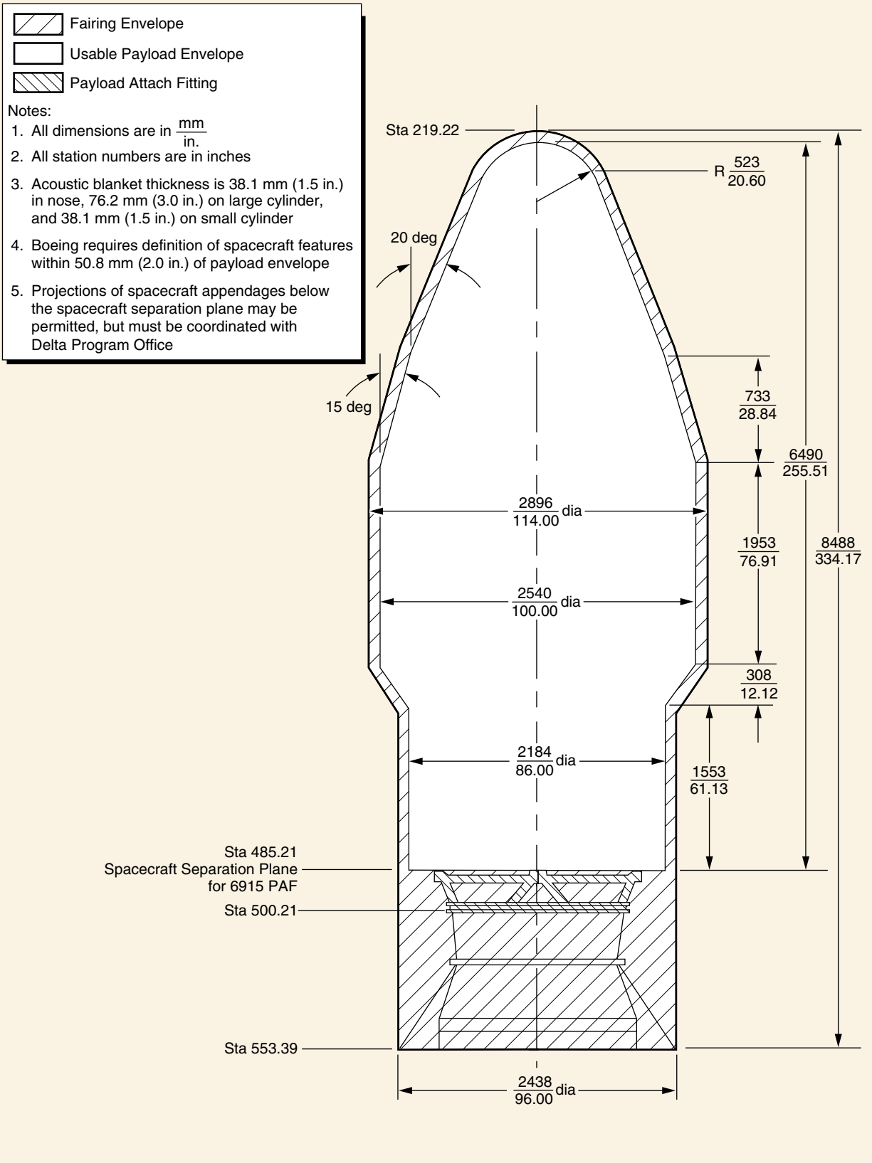
Figure 3-4. Payload Static Envelope, 2.9-m (9.5-ft)-dia Fairing, Two-Stage Configuration (6915 PAF)
