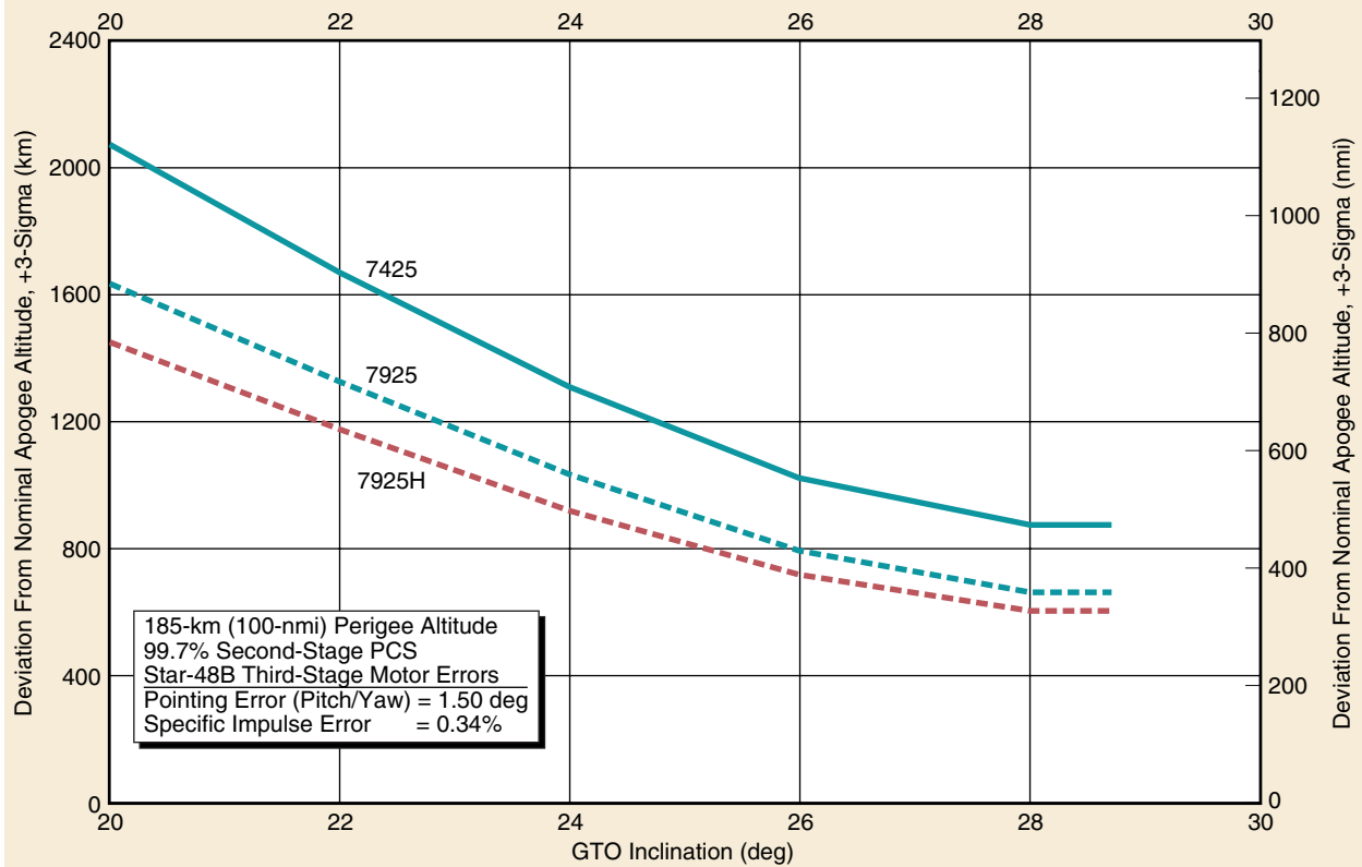
Figure 2-33. Delta II Vehicle, GTO Deviations Capability—Eastern Launch Site
