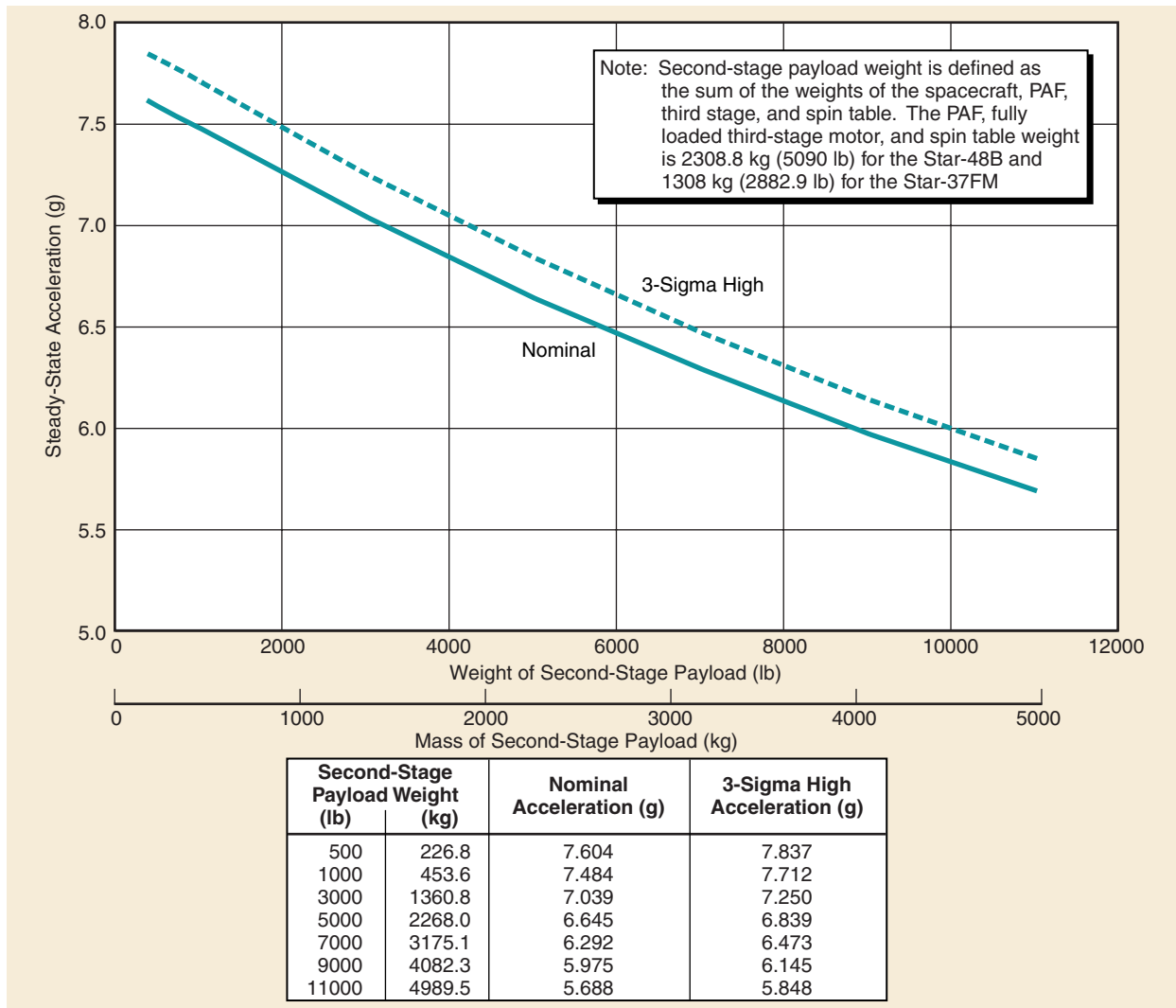
Figure 4-18. Axial Steady-State Acceleration at MECO vs. Payload Weight
