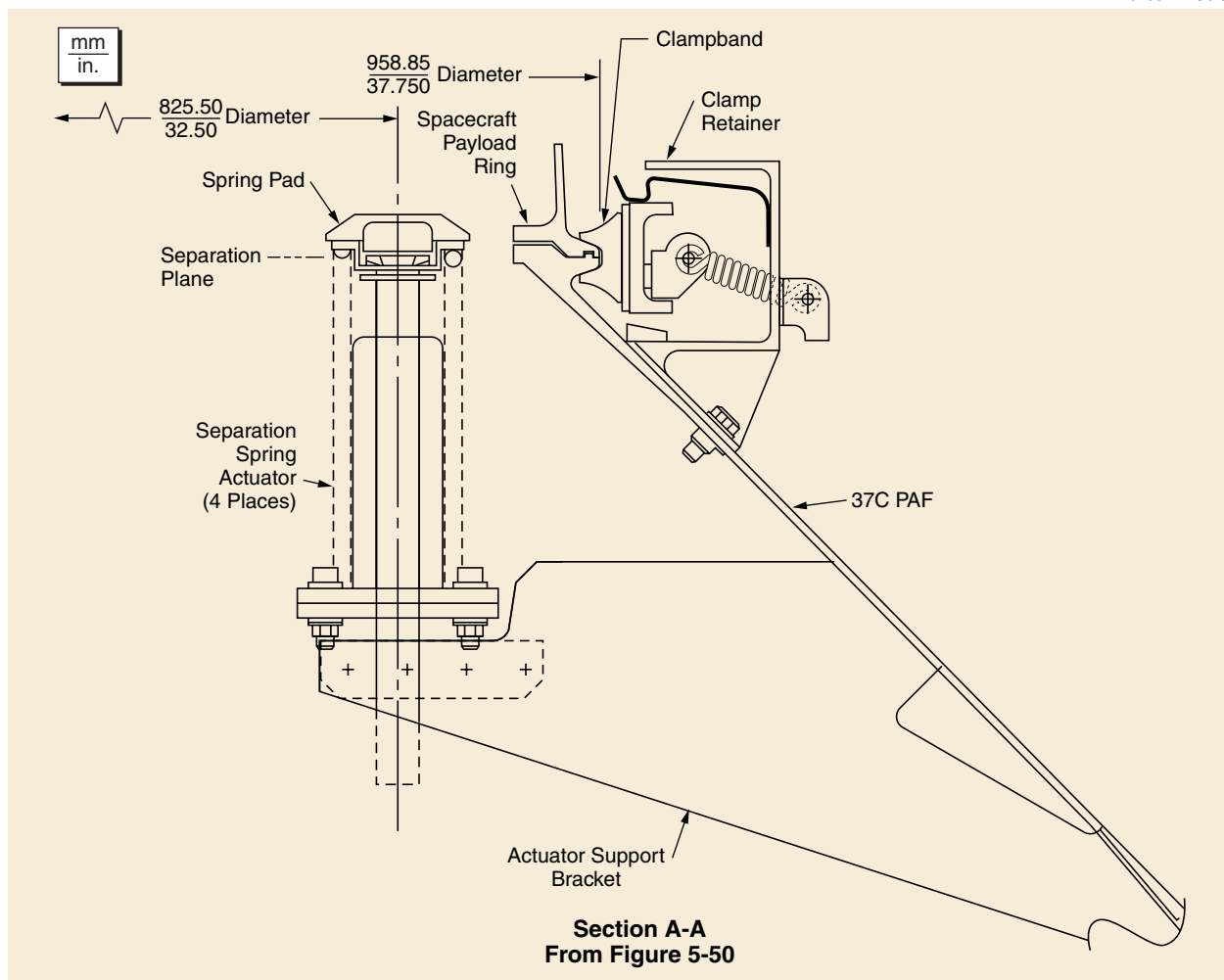
Figure 5-51. Dual-Payload Attach Fitting 37C PAF Separation System Interface
