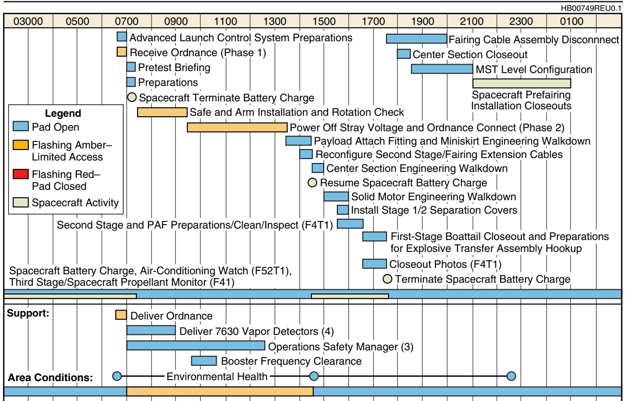
Figure 6-33. Typical Ordnance Installation and Hookup (T-5 Day)
