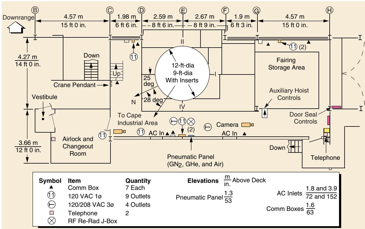
Figure 6-20B. Level 9B Floor Plan, Pad 17B
