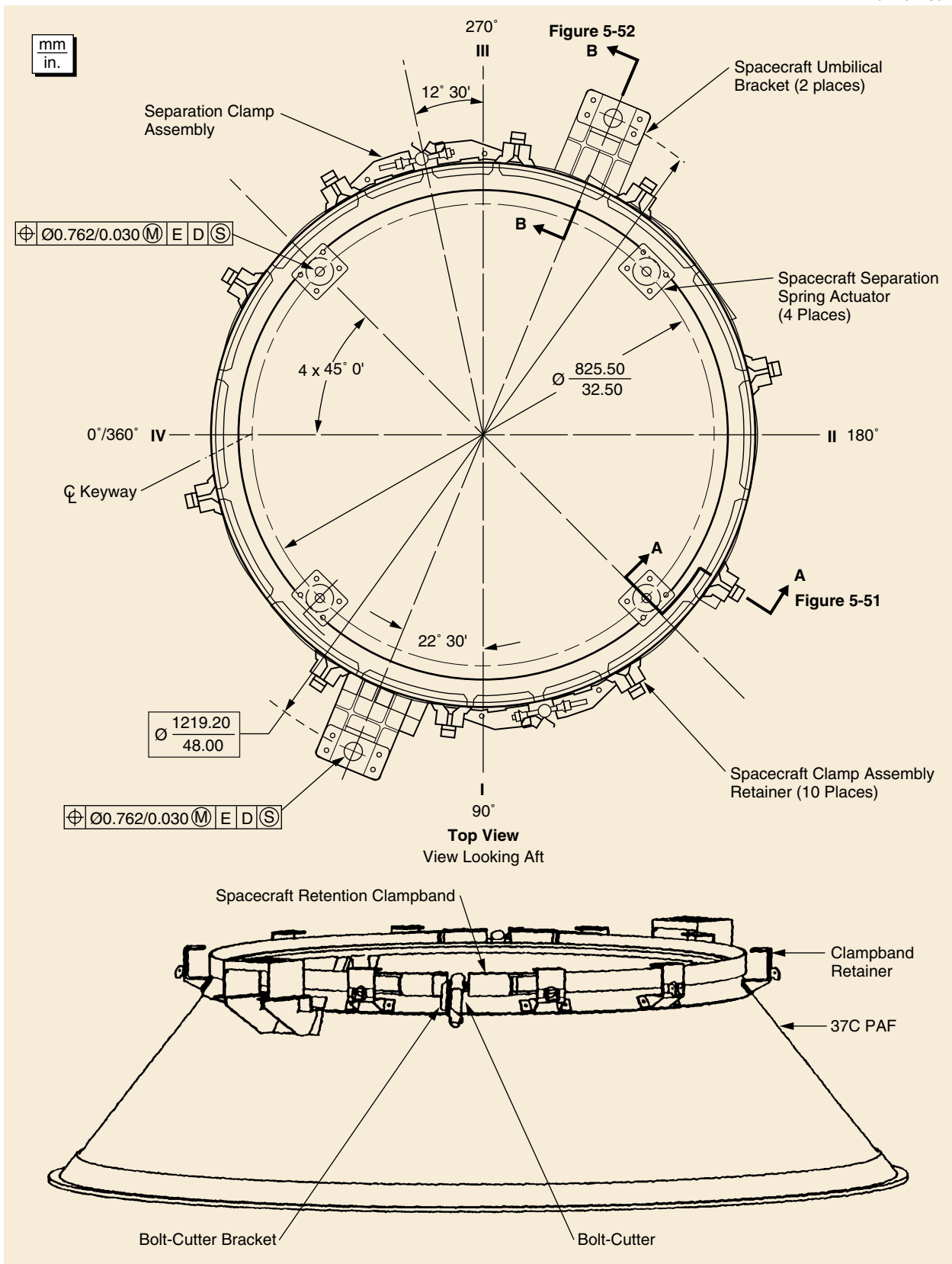
Figure 5-50. Dual-Payload Attach Fitting 37C PAF Interface
