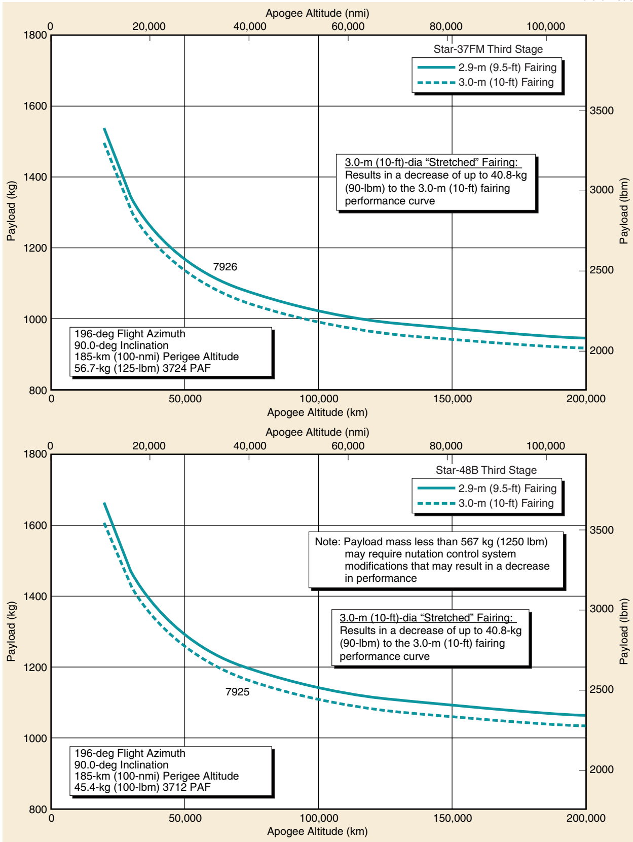
Figure 2-32. Delta II 792X Vehicle, Three-Stage Apogee Altitude Capability—Western Launch Site
