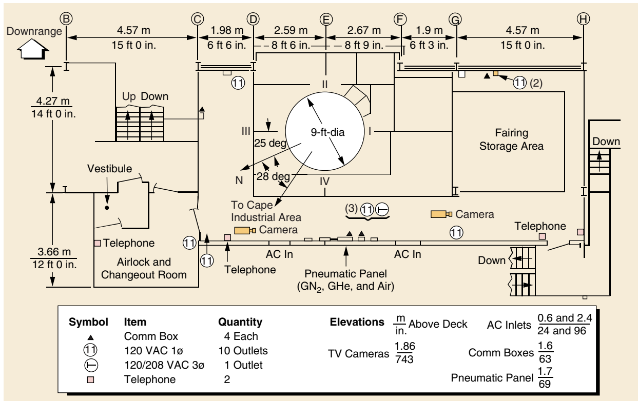
Figure 6-19B. Level 9A Floor Plan, Pad 17B
