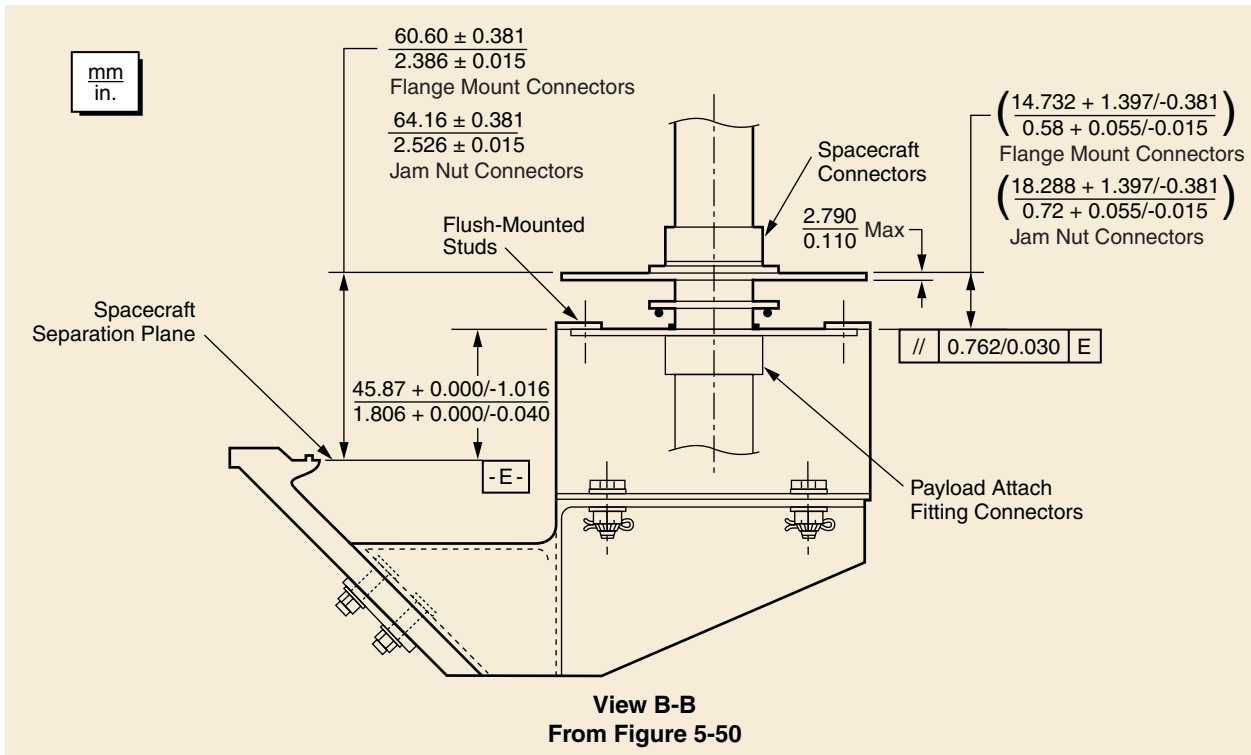
Figure 5-52. Dual-Payload Attach Fitting 37C PAF Spacecraft Separation Interface—Electrical Connector Bracket
