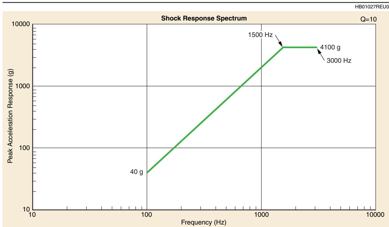
Figure 4-22. Maximum Flight Spacecraft Interface Shock Environment 3712A, 3712B, 3712C Payload Attach Fitting
