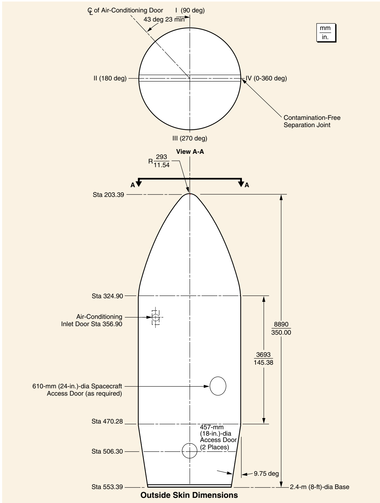
Figure 3-5. Profile, 3-m (10-ft)-dia Composite Fairing
