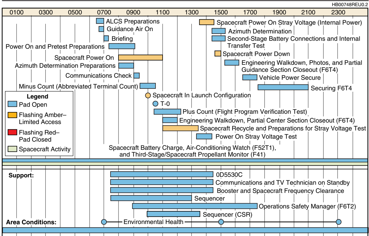
Figure 6-32. Typical Flight Program Verification and Stray-Voltage Checks (T-6 Day)
