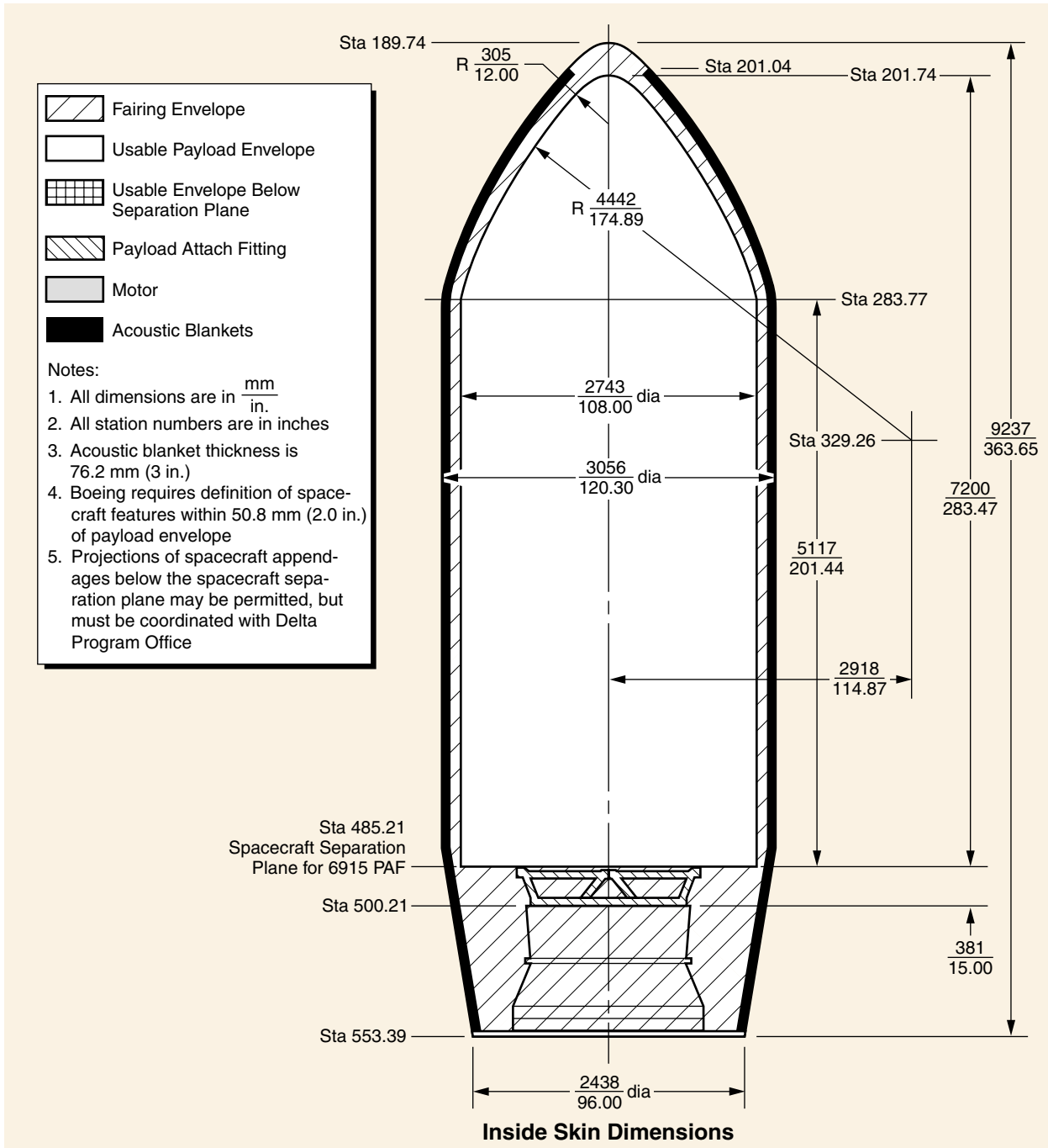
Figure 3-12. Payload Static Envelope, 3-m (10-ft)-dia Stretched Composite Fairing (-10L), Two-Stage Configuration (6915 PAF)
