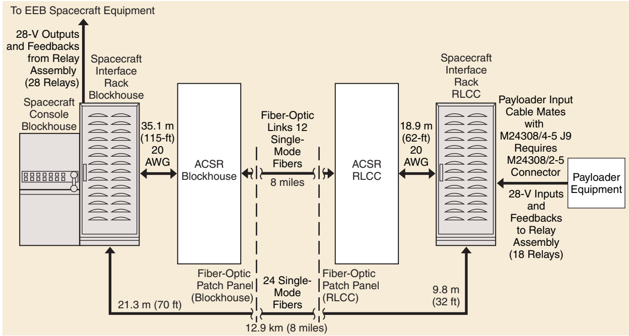
Figure 7-33. ACSR Blockhouse-to-RLCC Block Diagram
