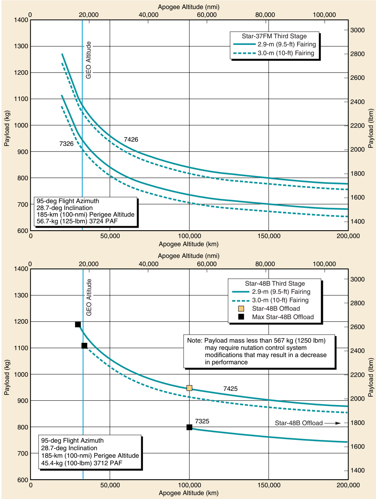
Figure 2-11. Delta II 732X/742X Vehicle, Three-Stage Apogee Altitude Capability—Eastern Launch Site
