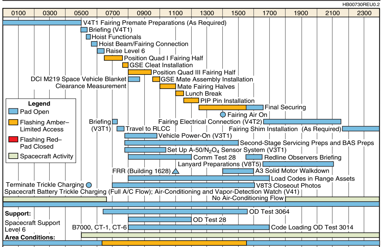
Figure 7-44. Typical Fairing Installation (T-4 Day)
