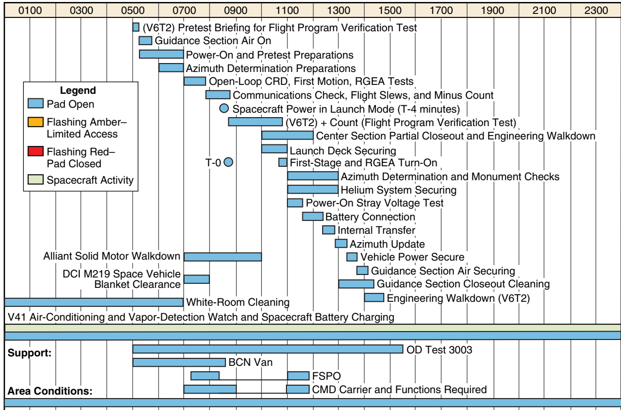
Figure 7-42. Typical Flight Program Verification and Stray Voltage Checks (T-6 Day)
