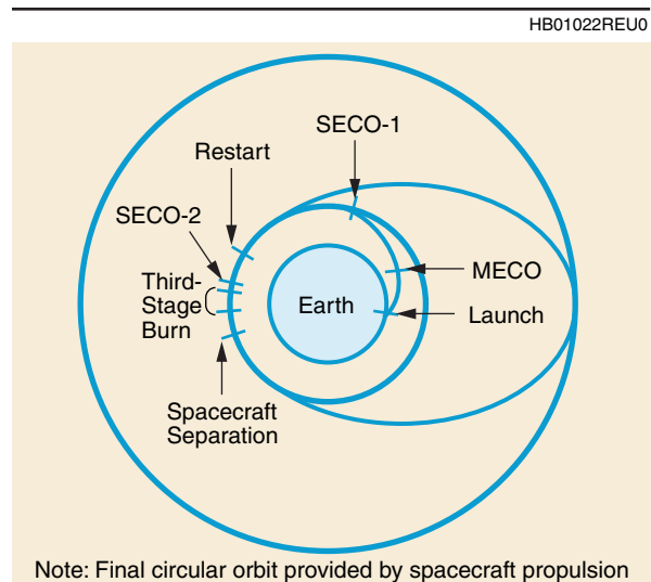
Figure 2-2. Typical Three-Stage Mission Profile
