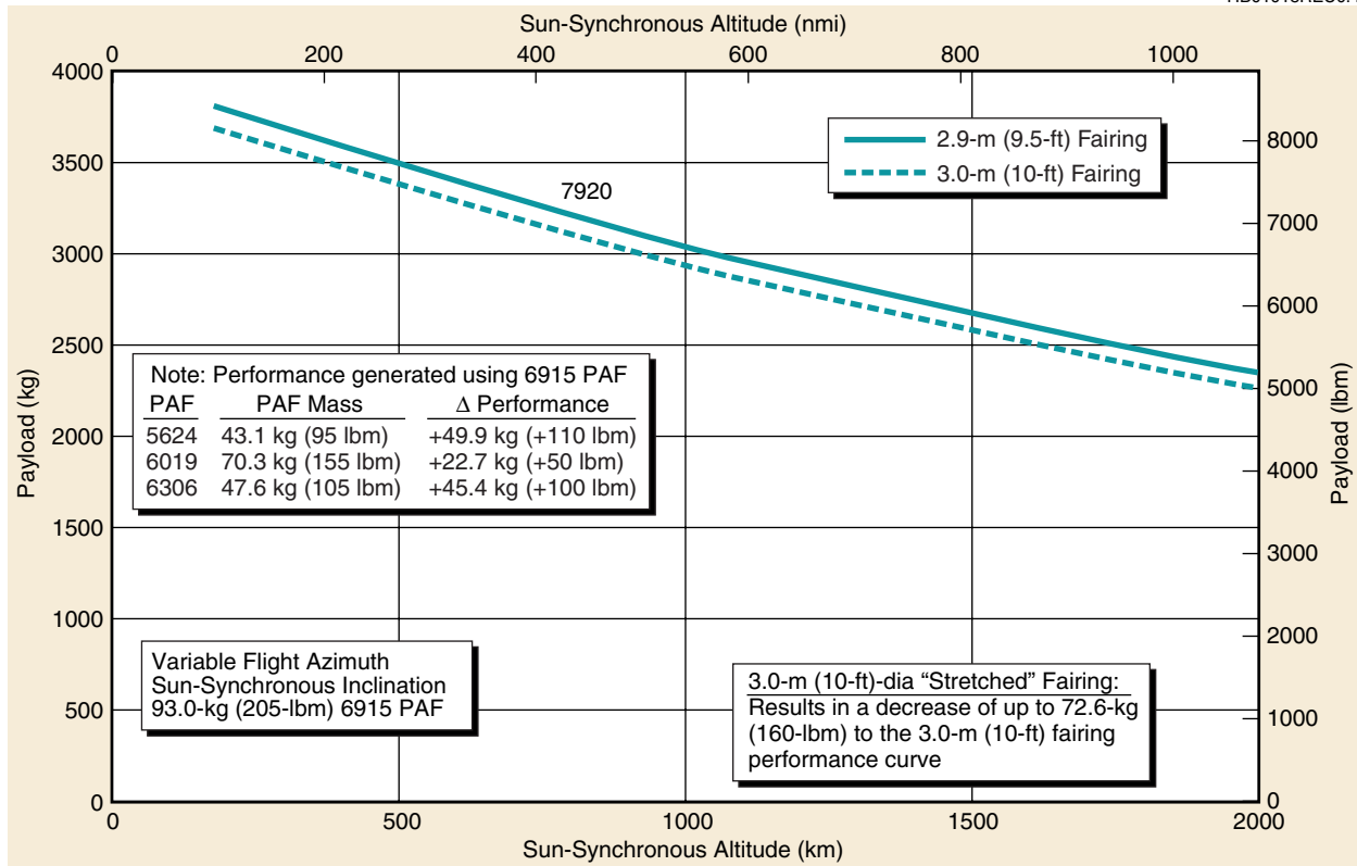
Figure 2-30. Delta II 7920 Vehicle, Two-Stage Sun-Synchronous Capability—Western Launch Site
