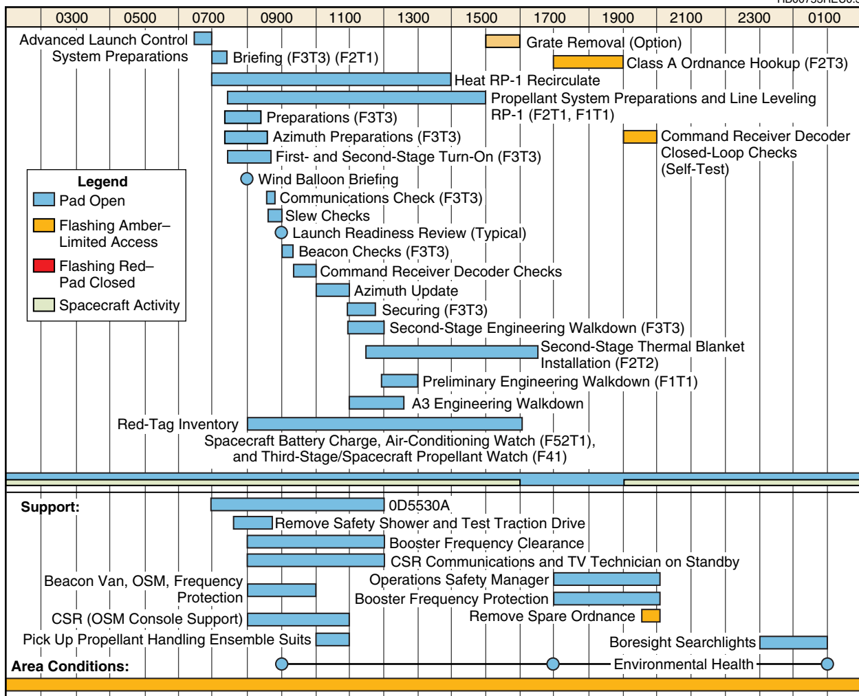
Figure 6-37. Typical Beacon, Range Safety, and Class A Ordnance (T-1 Day)
