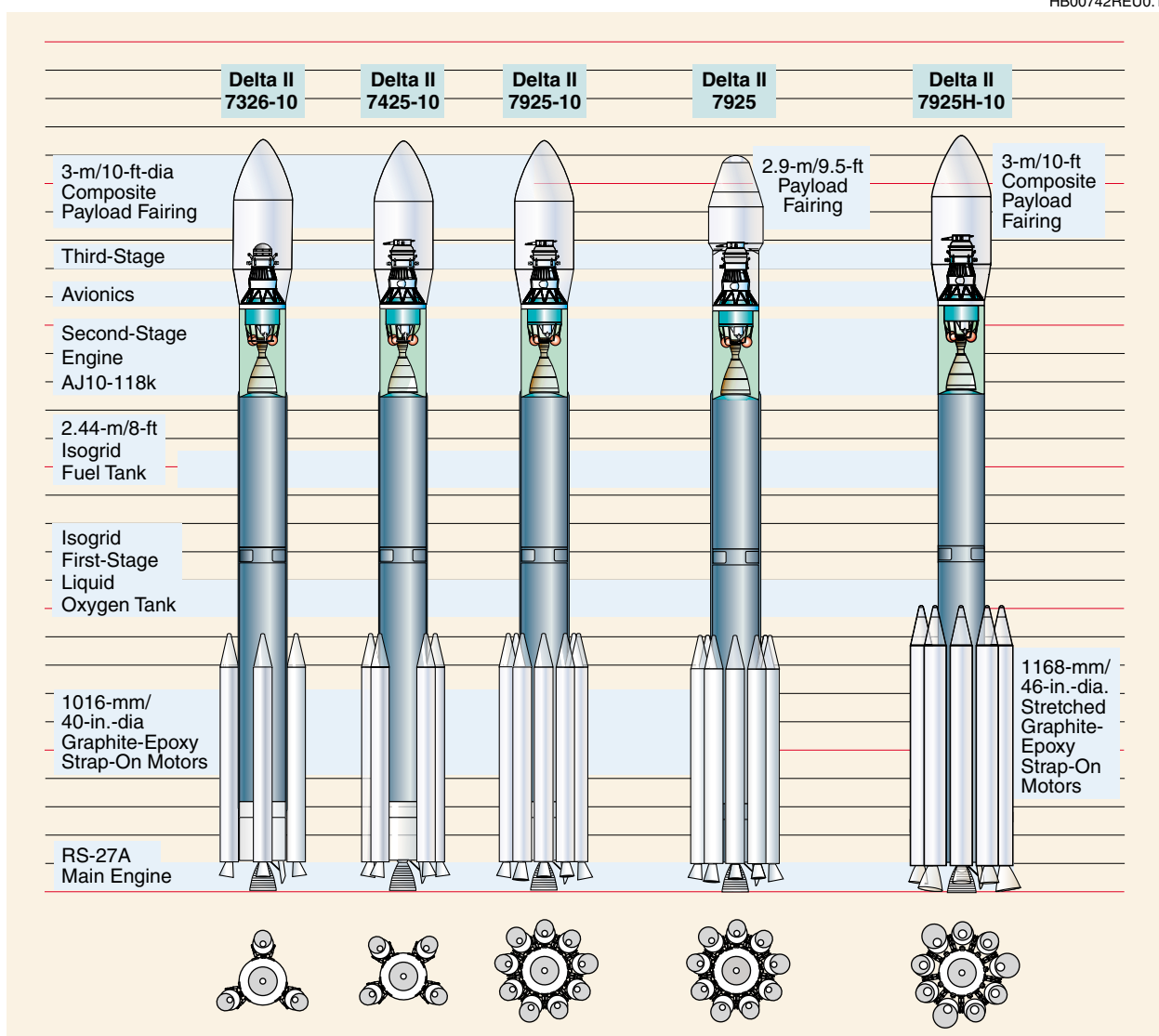
Figure 1-3. Some Typical Configurations of the Delta II Launch Vehicle with Optional Third Stage
