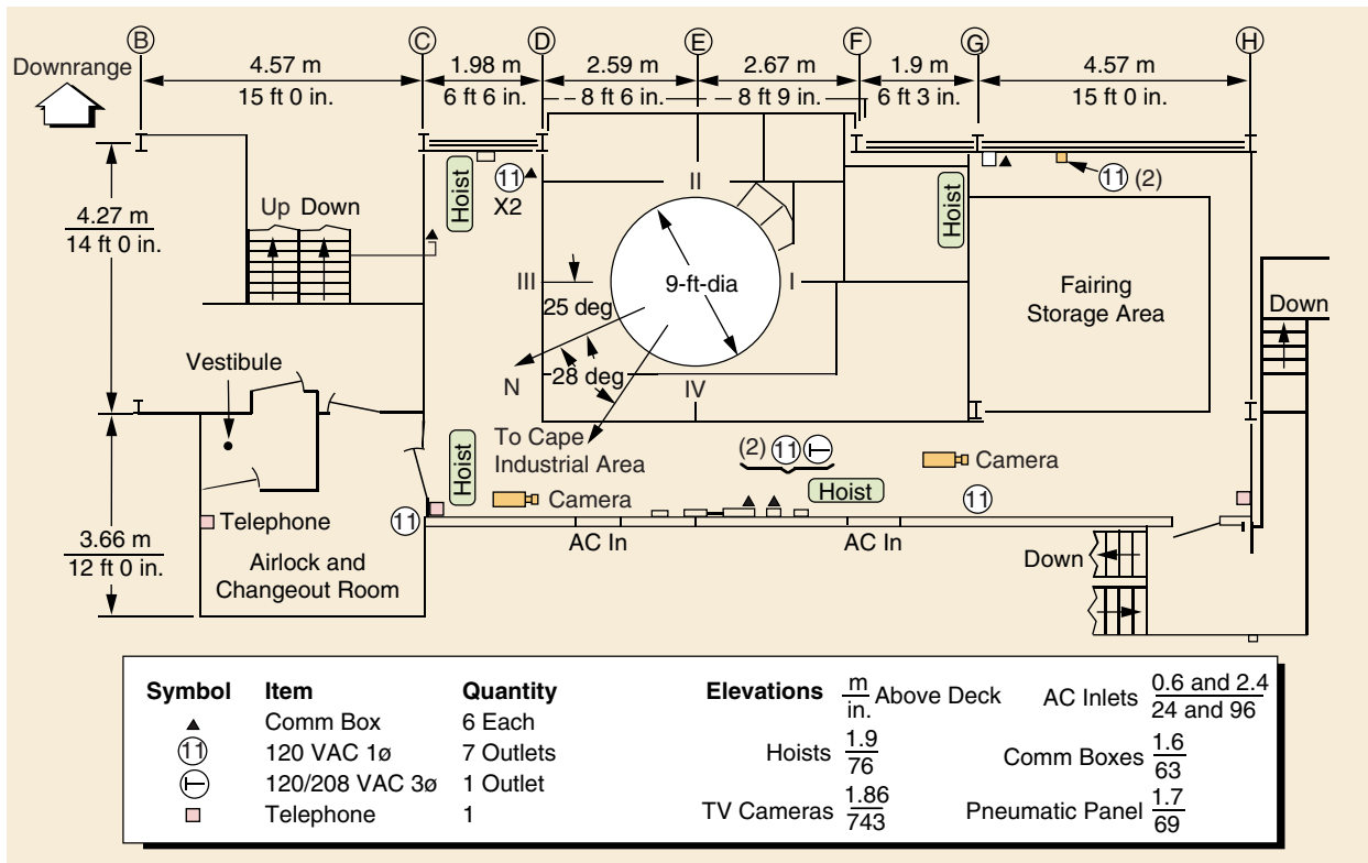
Figure 6-19A. Level 9A Floor Plan, Pad 17A
