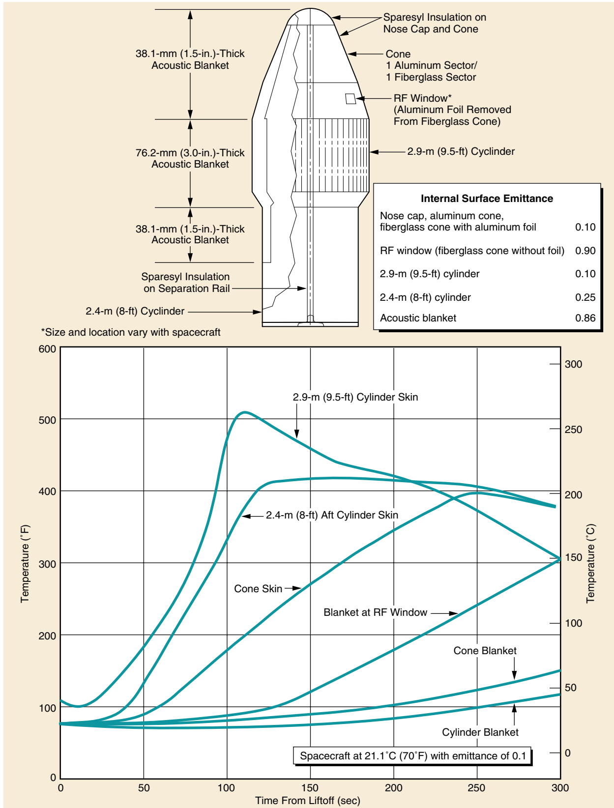
Figure 4-7. Predicted Maximum Internal Wall Temperature and Internal Surface Emittance (9.5-ft Fairing)
