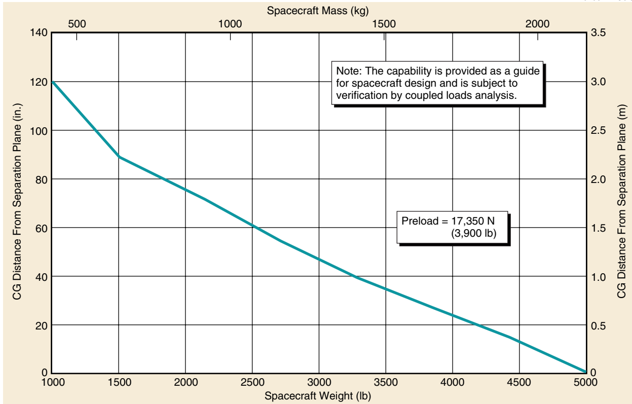
Figure 5-42. Capability of the 5624 PAF
