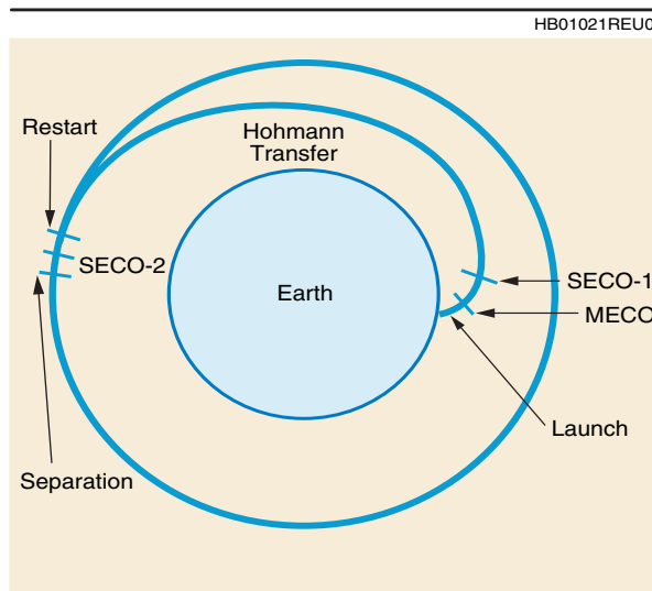
Figure 2-1. Typical Two-Stage Mission Profile
