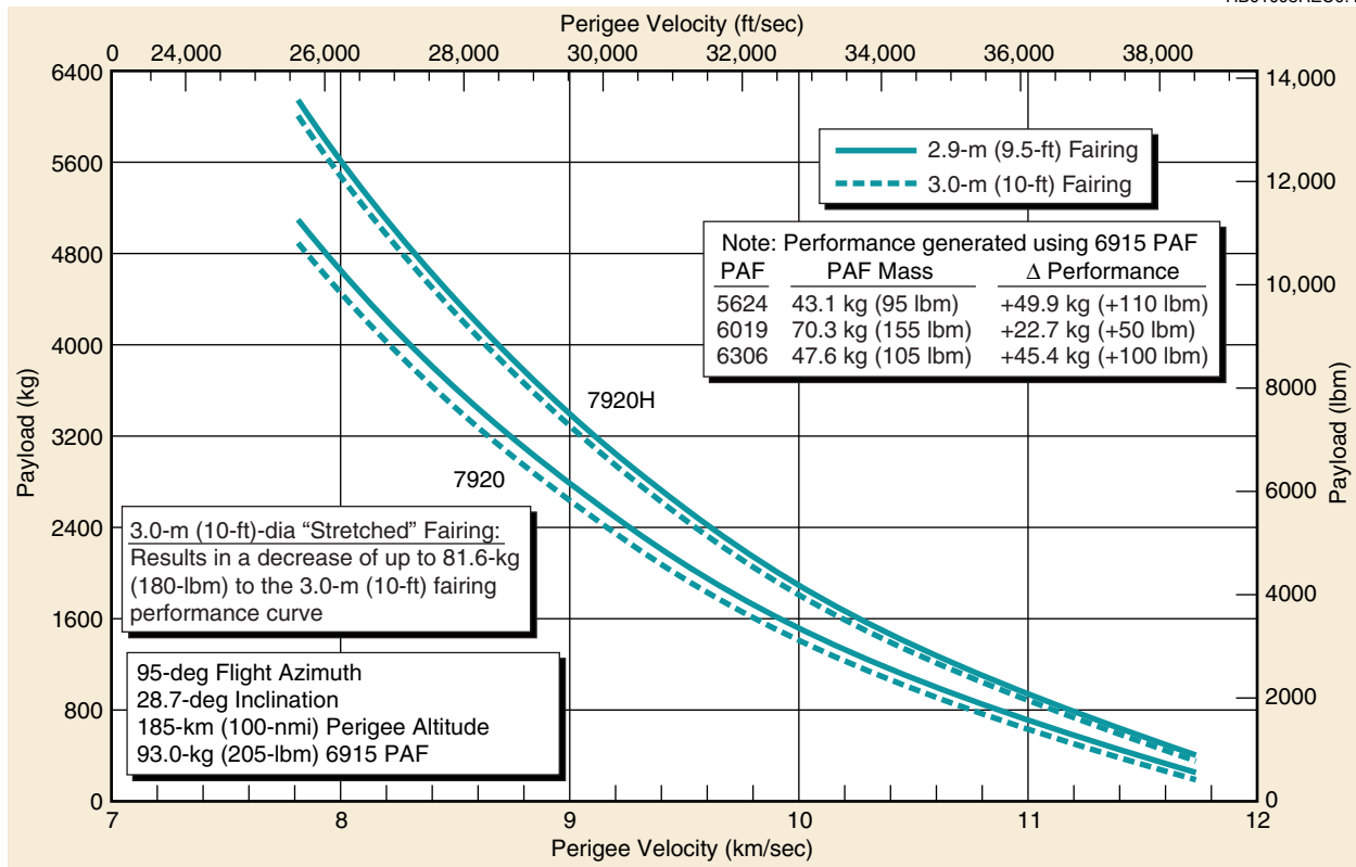
Figure 2-20. Delta II 7920/7920H Vehicle, Two-Stage Perigee Velocity Capability—Eastern Launch Site
