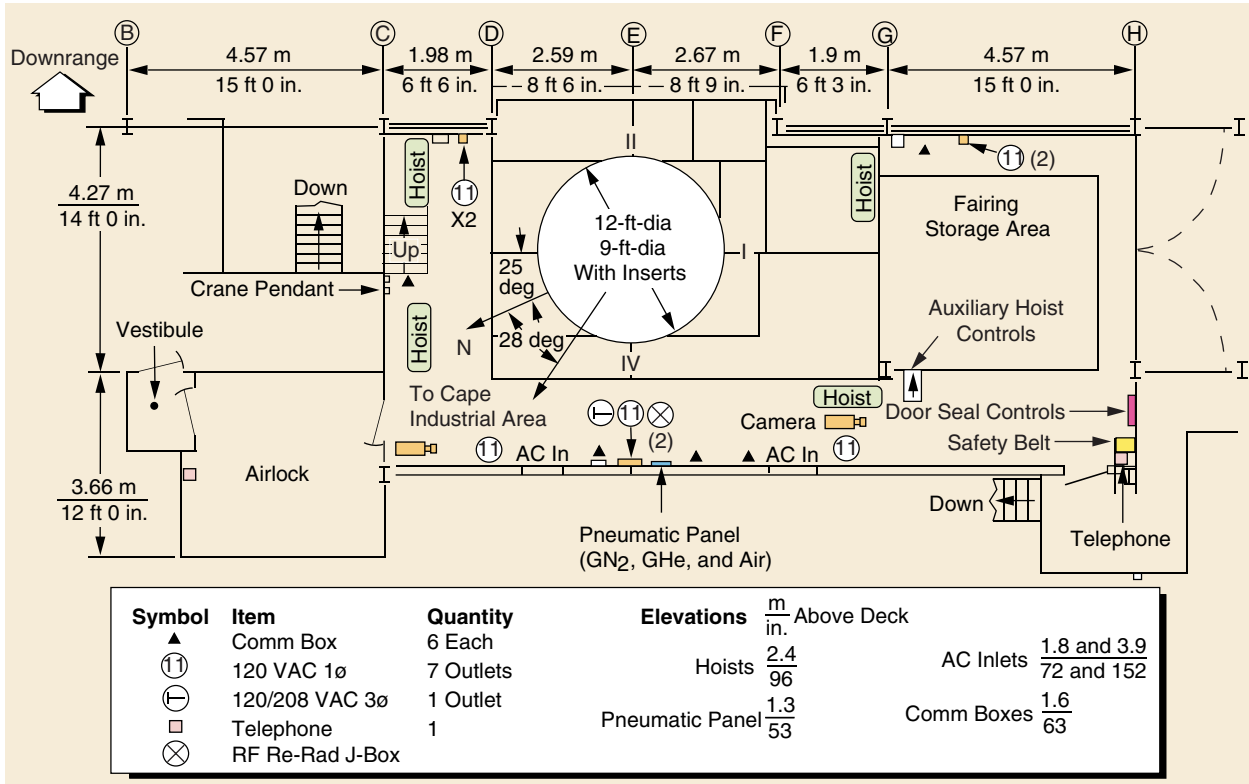
Figure 6-20A. Level 9B Floor Plan, Pad 17A
