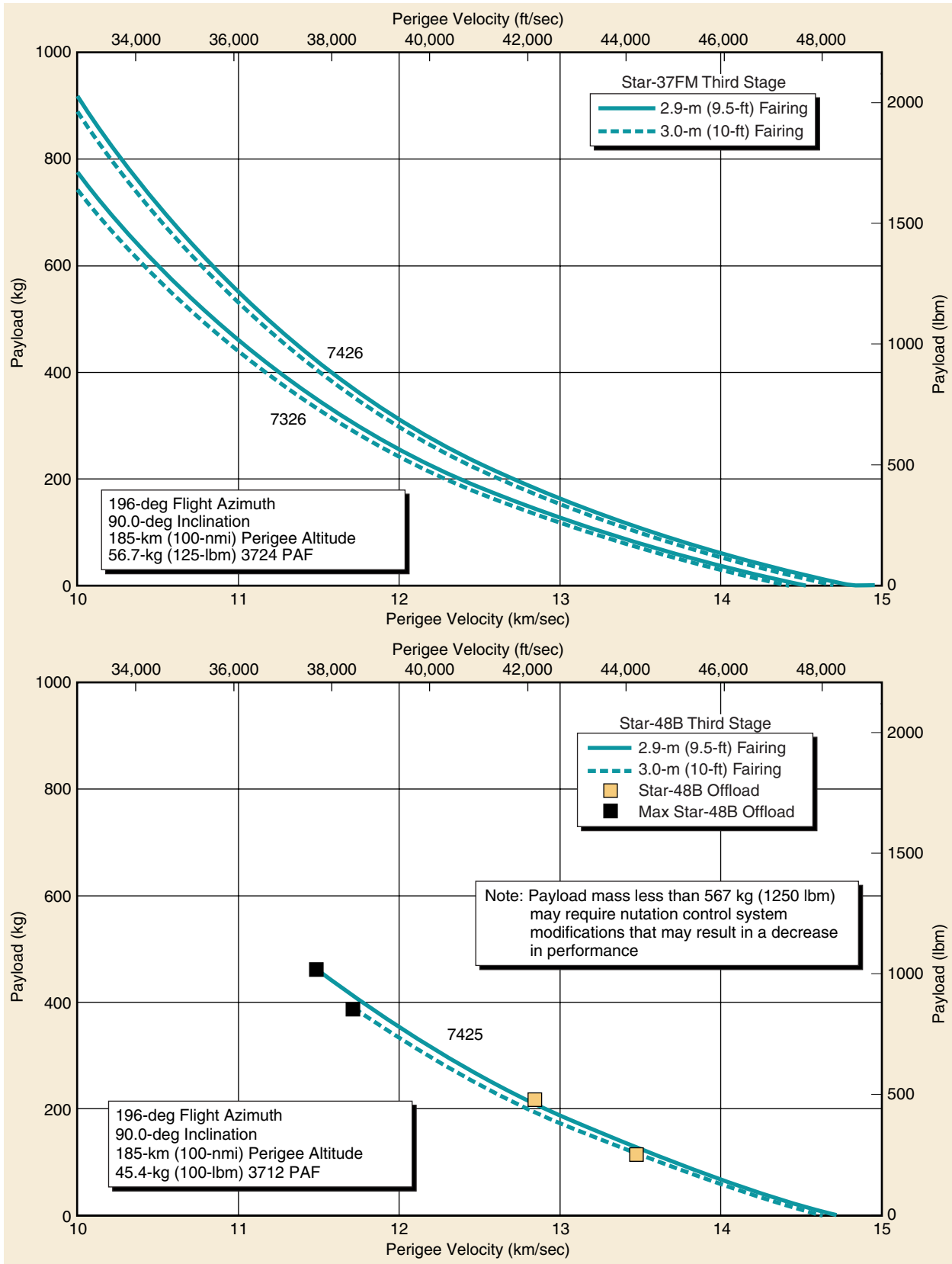
Figure 2-18. Delta II 732X/742X Vehicle, Three-Stage Perigee Velocity Capability—Western Launch Site
