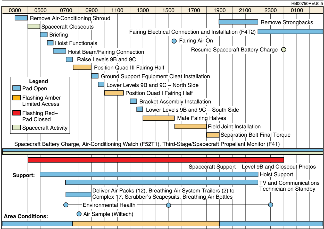
Figure 6-34. Typical Fairing Installation (T-4 Day)
