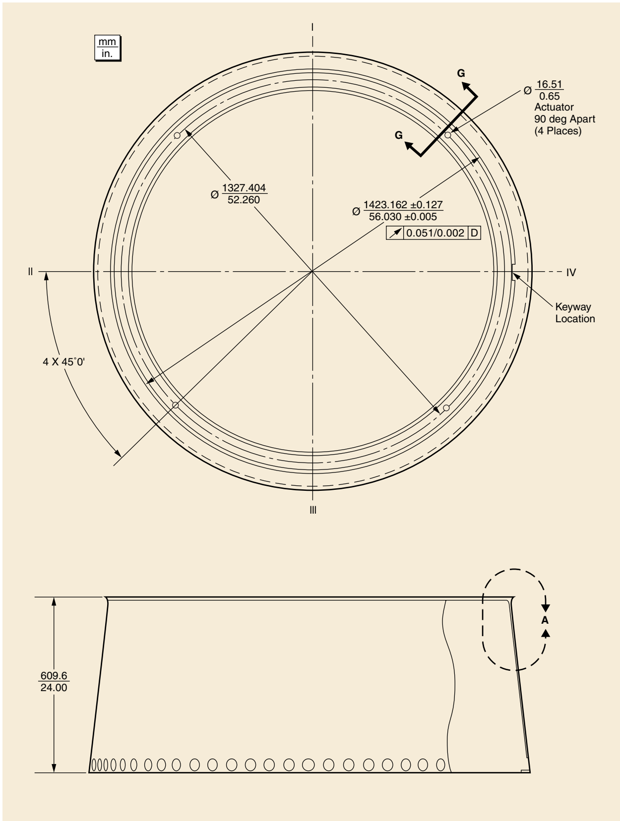
Figure 5-41. 5624 PAF Detailed Assembly
