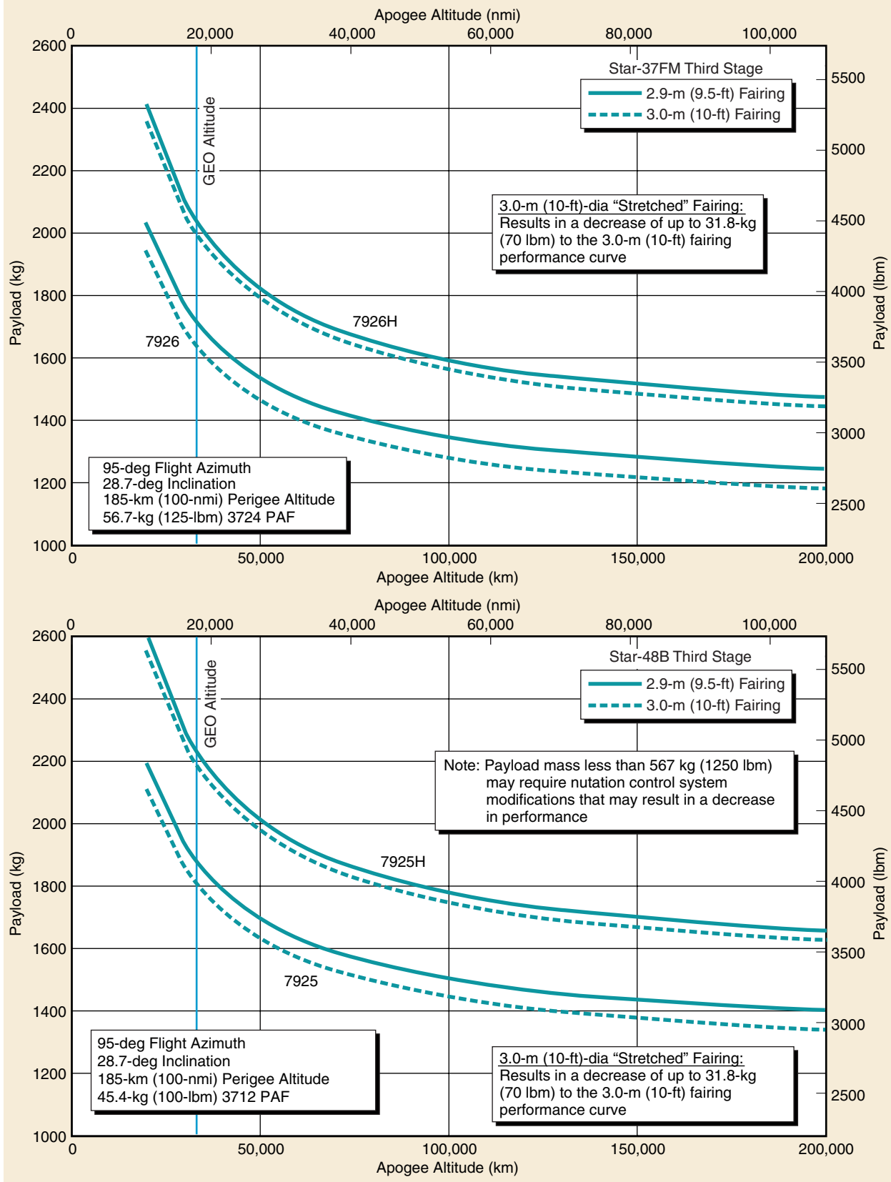
Figure 2-24. Delta II 792X/792XH Vehicle, Three-Stage Apogee Altitude Capability—Eastern Launch Site
