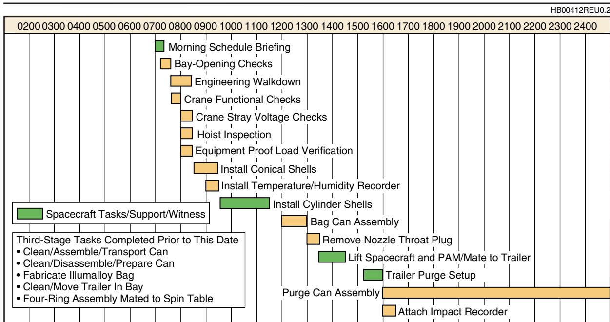
Figure 6-30. Typical Installation of Transportation Can (T-8 Day)
