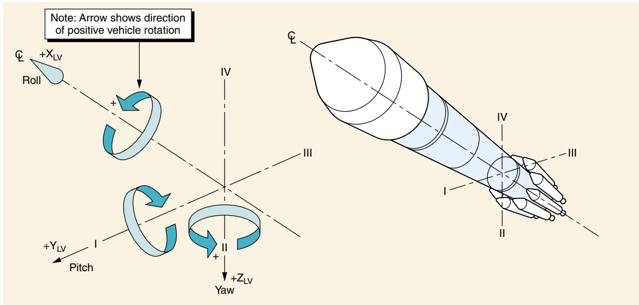
Figure 1-7. Vehicle Axes
