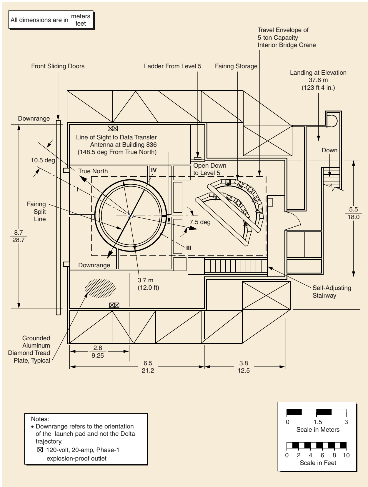
Figure 7-28. Level 6 of SLC-6 Mobile Service Tower—Plan View
