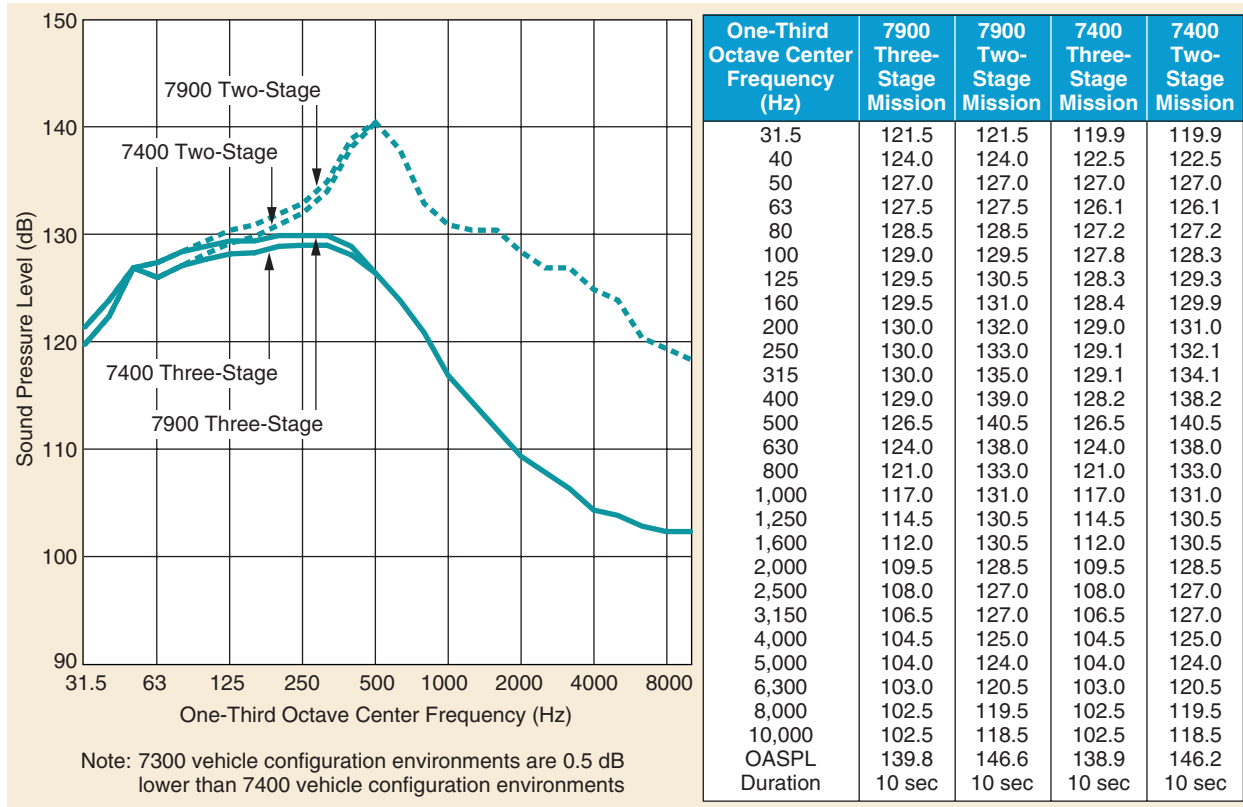
Figure 4-20. Predicted Delta II Acoustic Environments for 9.5-ft Fairing Missions
