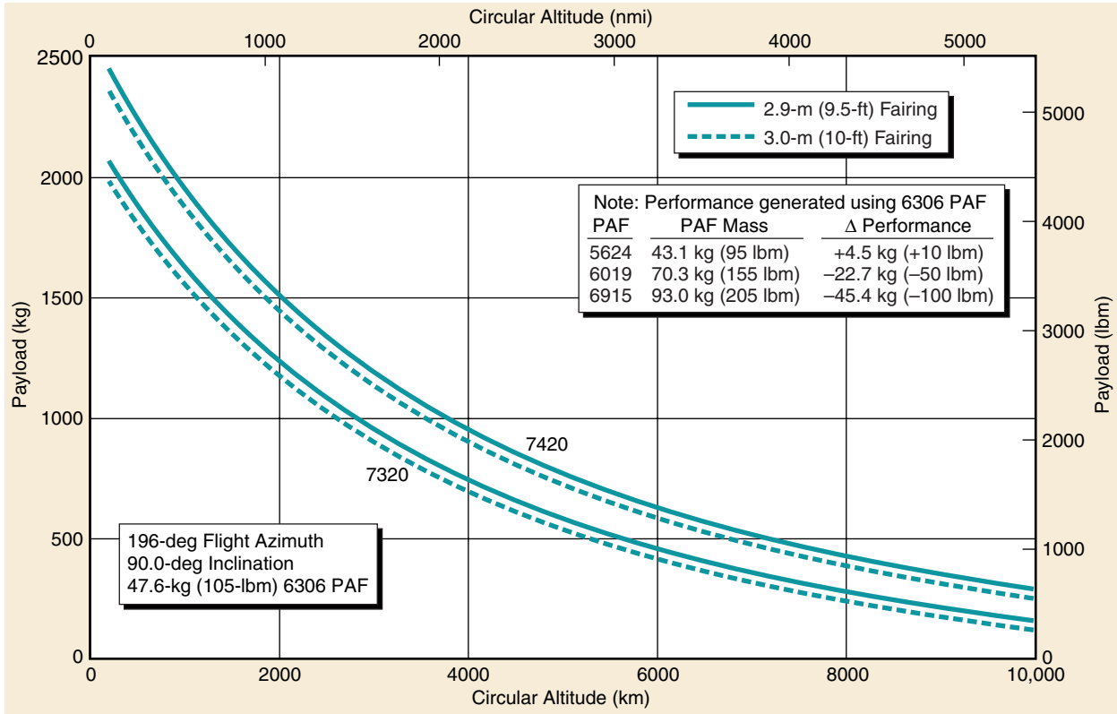
Figure 2-16. Delta II 7320/7420 Vehicle, LEO Two-Stage Circular Orbit Altitude Capability—Western Launch Site
