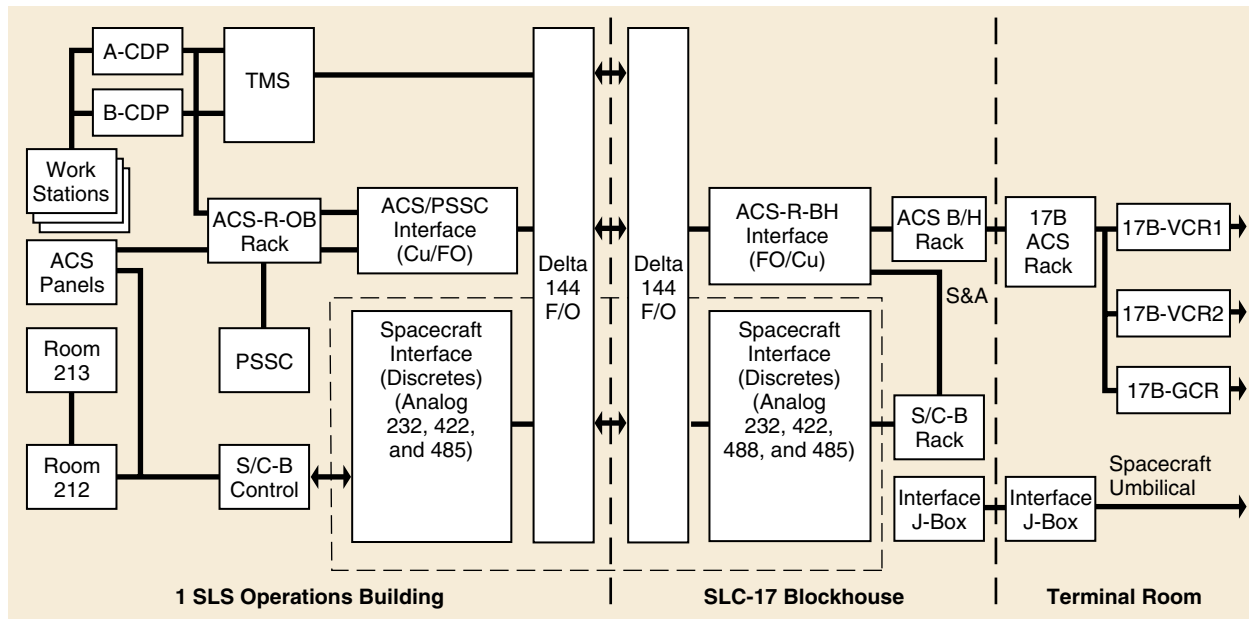
Figure 6-23. Interface Overview—Spacecraft Control Rack in 1 SLS Operations Building
