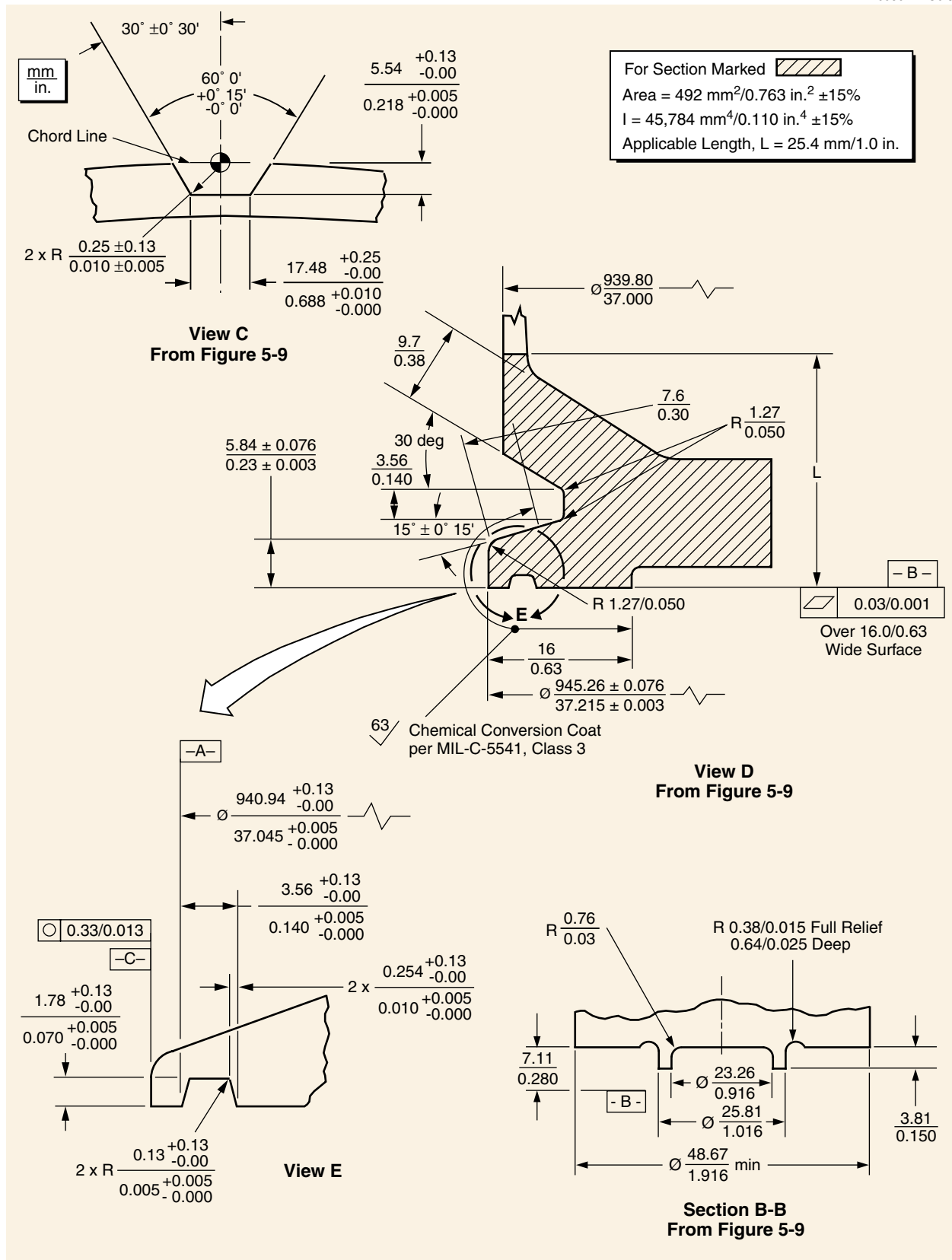
Figure 5-10. Dimensional Constraints on Spacecraft Interface to 3712A PAF (Views C, D, E, and Section B-B)
