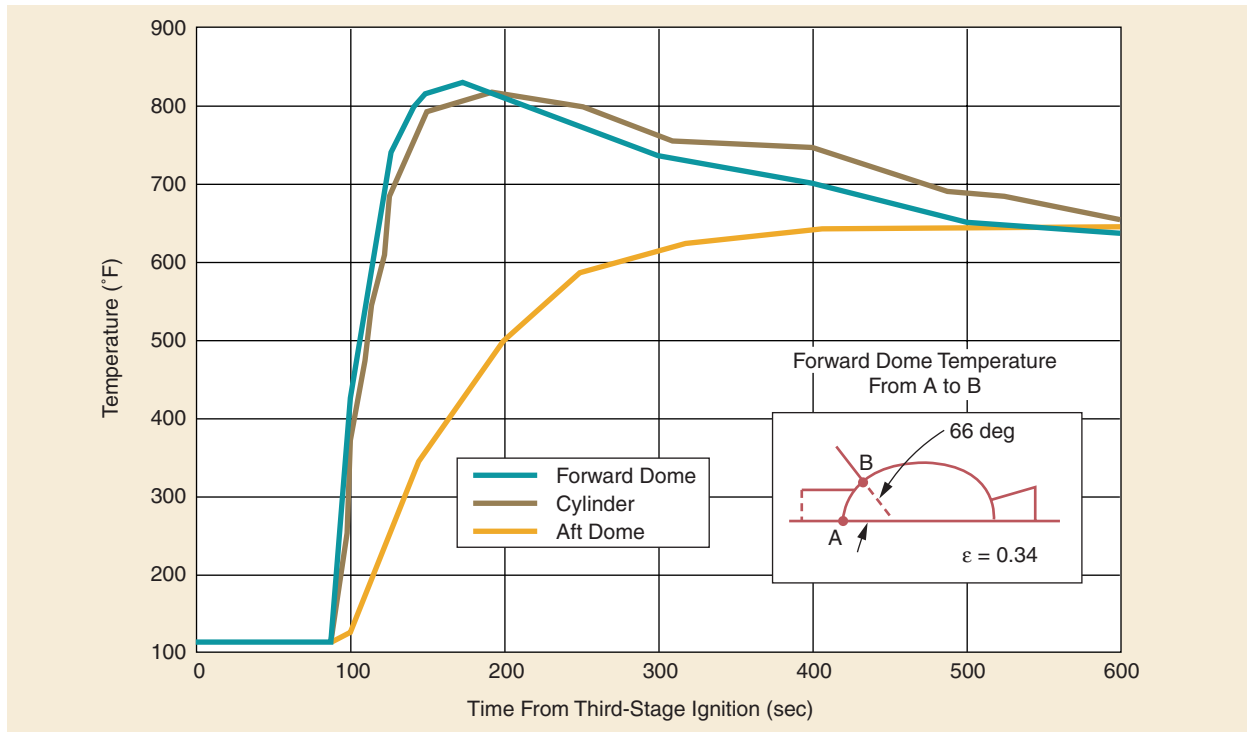
Figure 4-16. Star-48B Motor Case Soakback Temperature for Payload Mass Between 300 kg (661 lb) and 460 kg (1014 lb)
