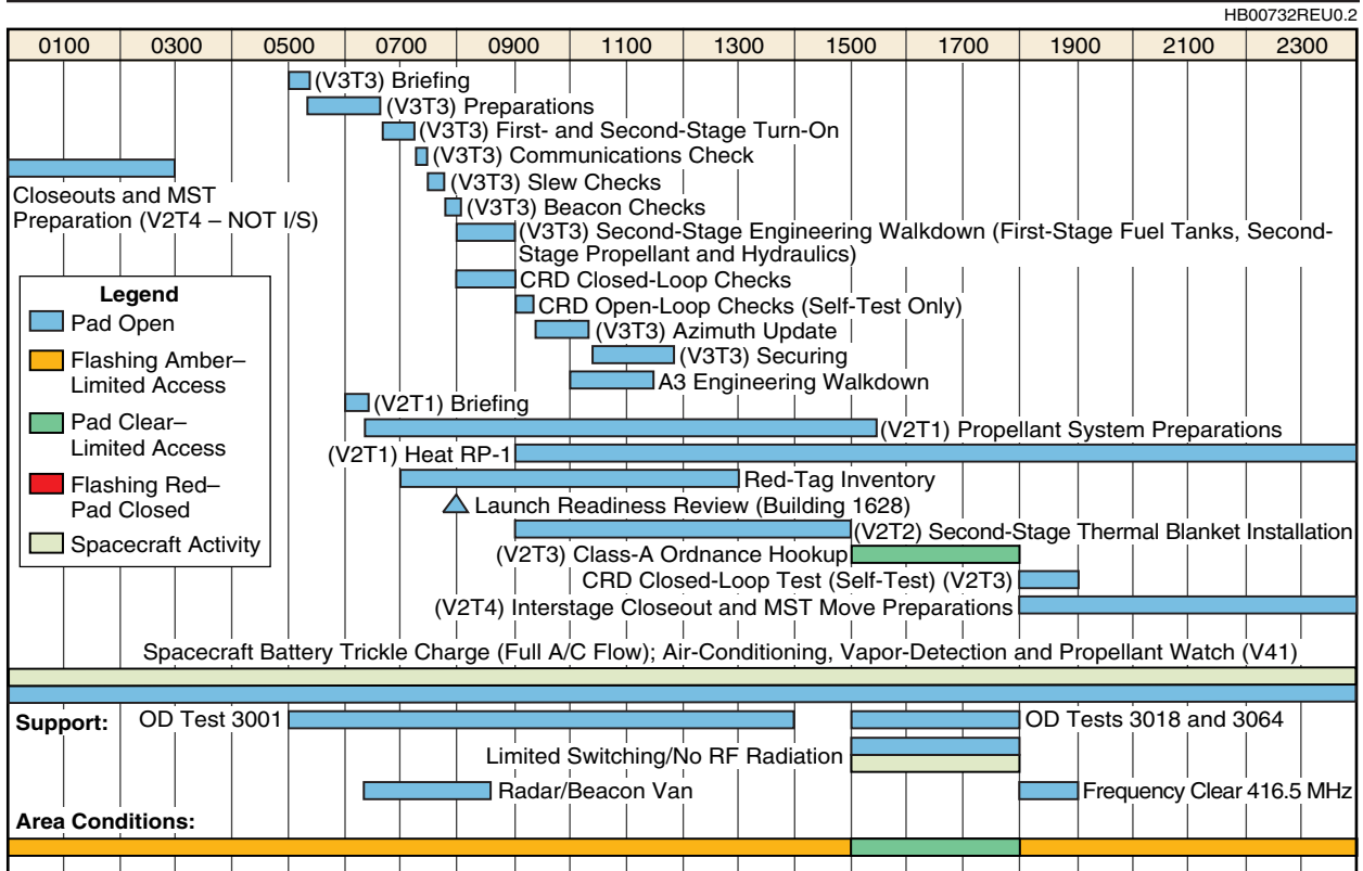
Figure 7-46. Typical Beacon and Range Safety Checks/Class-A Ordnance Connect (T-2 Day)
