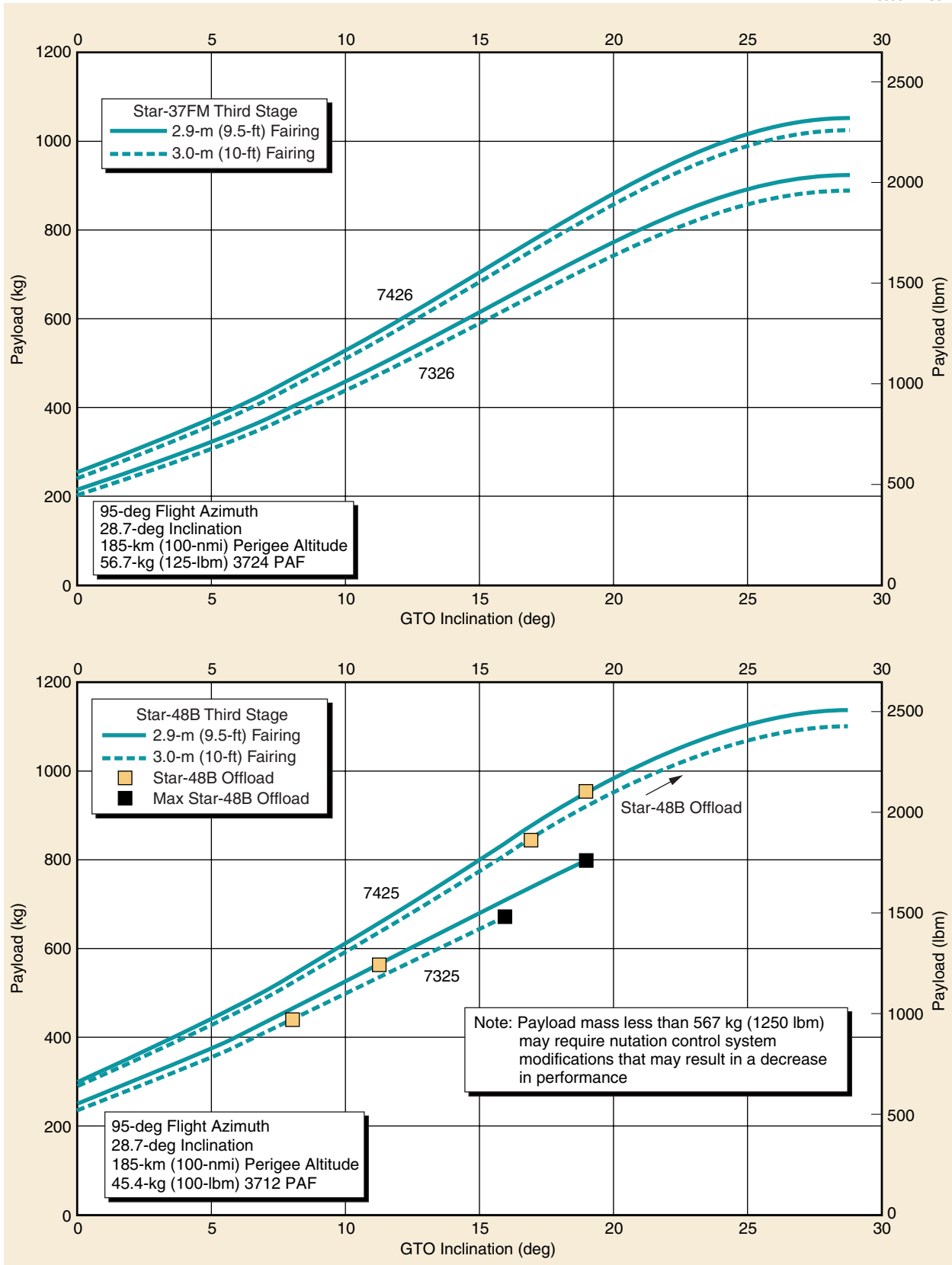
Figure 2-12. Delta II 732X/742X Vehicle, Three-Stage GTO Inclination Capability—Eastern Launch Site
