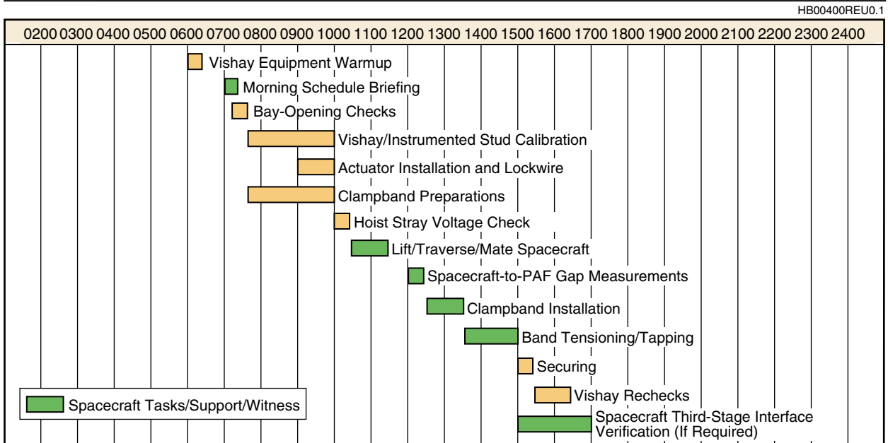
Figure 6-28. Typical Mating of Spacecraft and Third Stage (T-10 Day)
