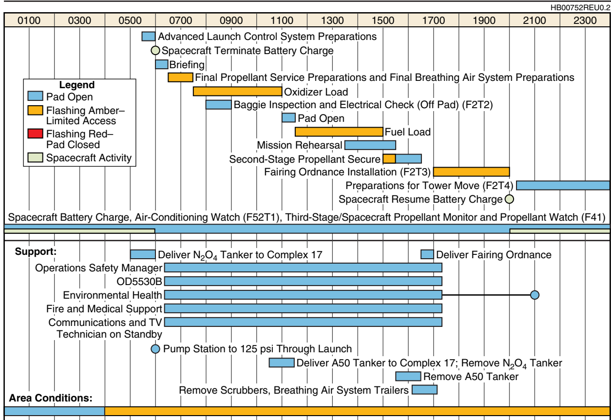
Figure 6-36. Typical Second-Stage Propellant Loading (T-2 Day)
