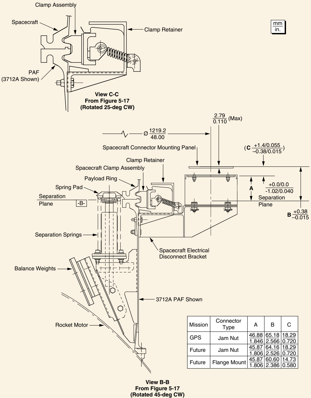
Figure 5-18. 3712A Clamp Assembly and Spring Actuator
