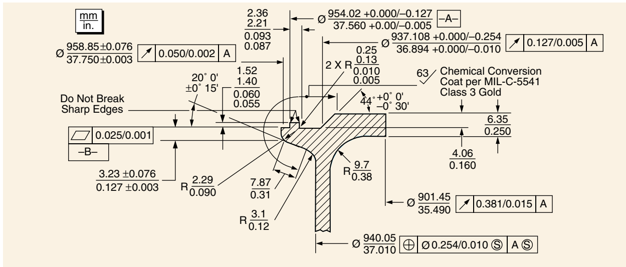
Figure 5-14. 3712C and 3724C PAF Detailed Dimensions
