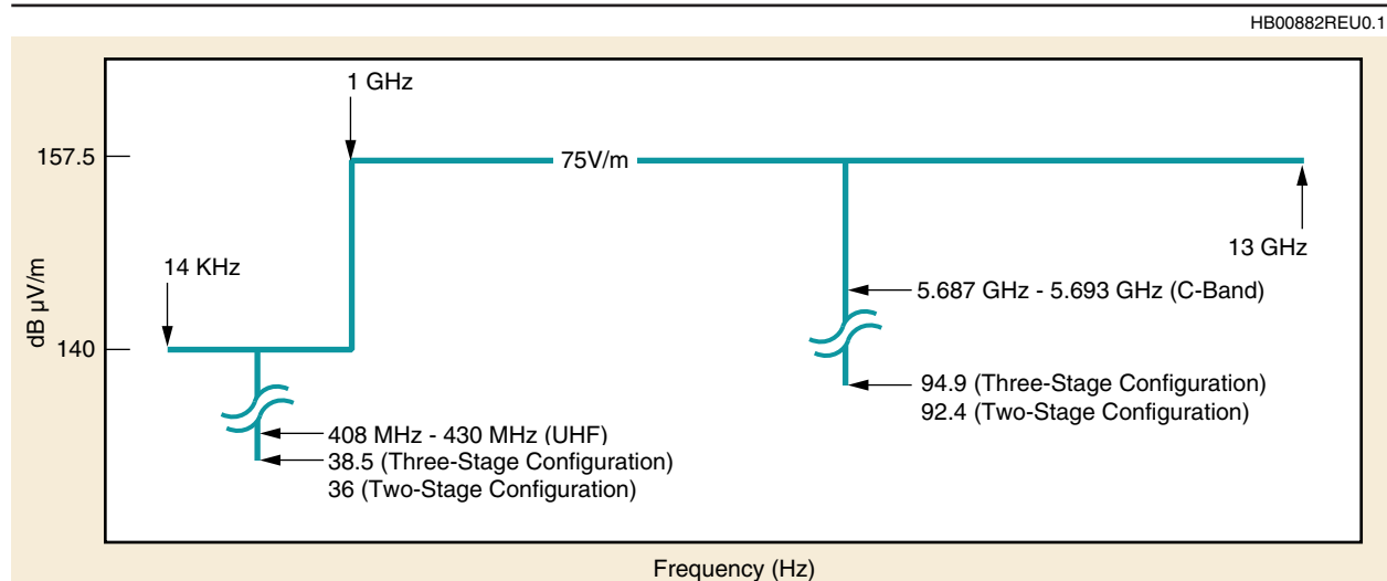
Figure 4-5. Maximum Allowable Payload Radiated Emissions at the Payload/ Launch Vehicle Separation Plane
