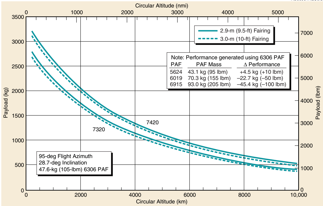
Figure 2-9. Delta II 7320/7420 Vehicle, Two-Stage Circular Orbit Altitude Capability—ER Launch Site
