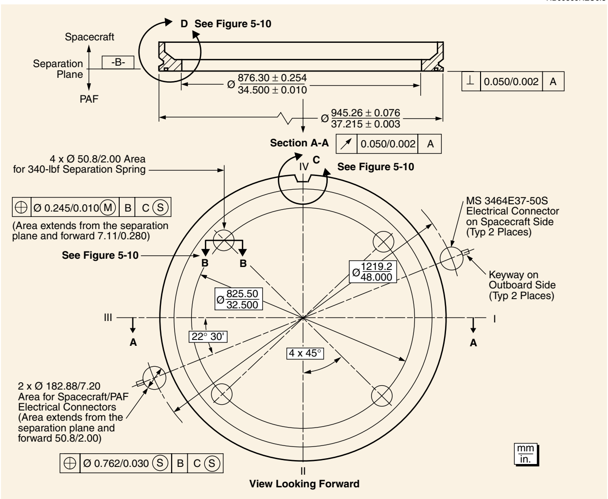
Figure 5-9. Dimensional Constraints on Spacecraft Interface to 3712A PAF
