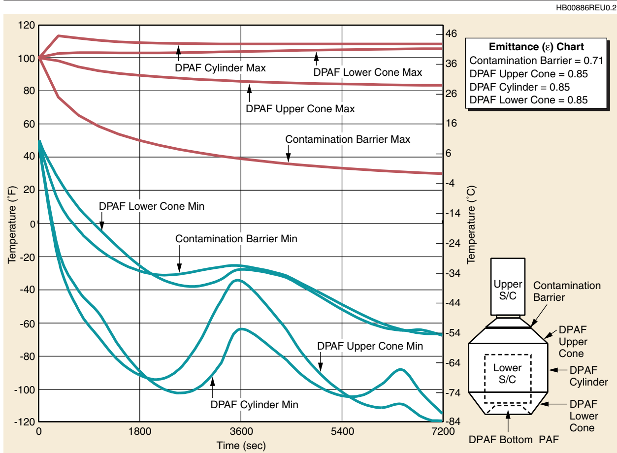
Figure 4-9. Predicted Maximum and Minimum Internal DPAF Temperature (Internal Emittance \cong 0.71, 0.86 )
