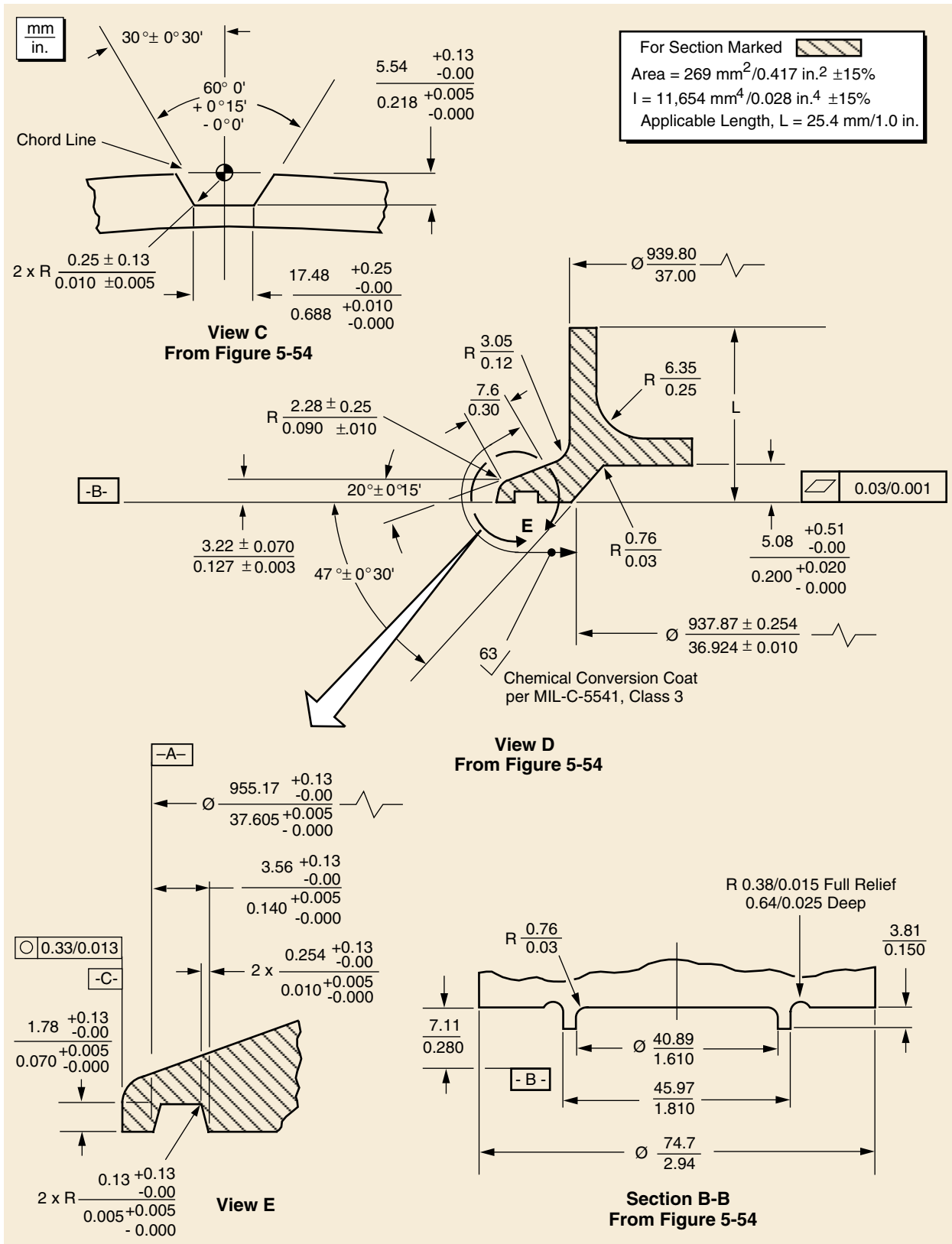
Figure 5-55. Dimensional Constraints on Spacecraft Interface to 37C PAF (Views C, D, E, and Section B-B)
