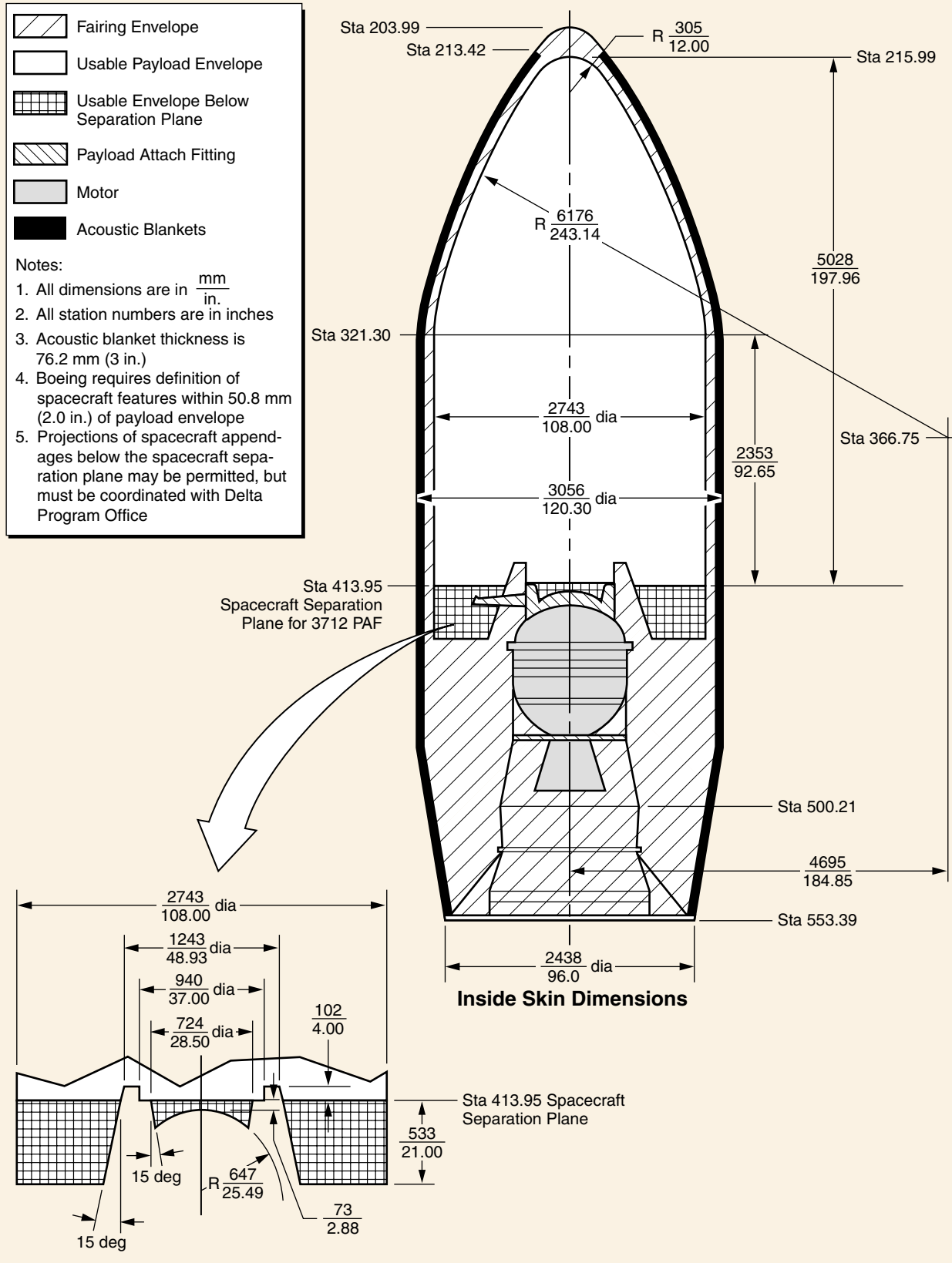
Figure 3-7. Payload Static Envelope, 3-m (10-ft)-dia Fairing, Three-Stage Configuration (3712 PAF)
