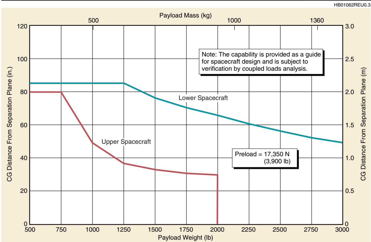
Figure 5-49. Capability of Dual-Payload Attach Fitting (DPAF)
