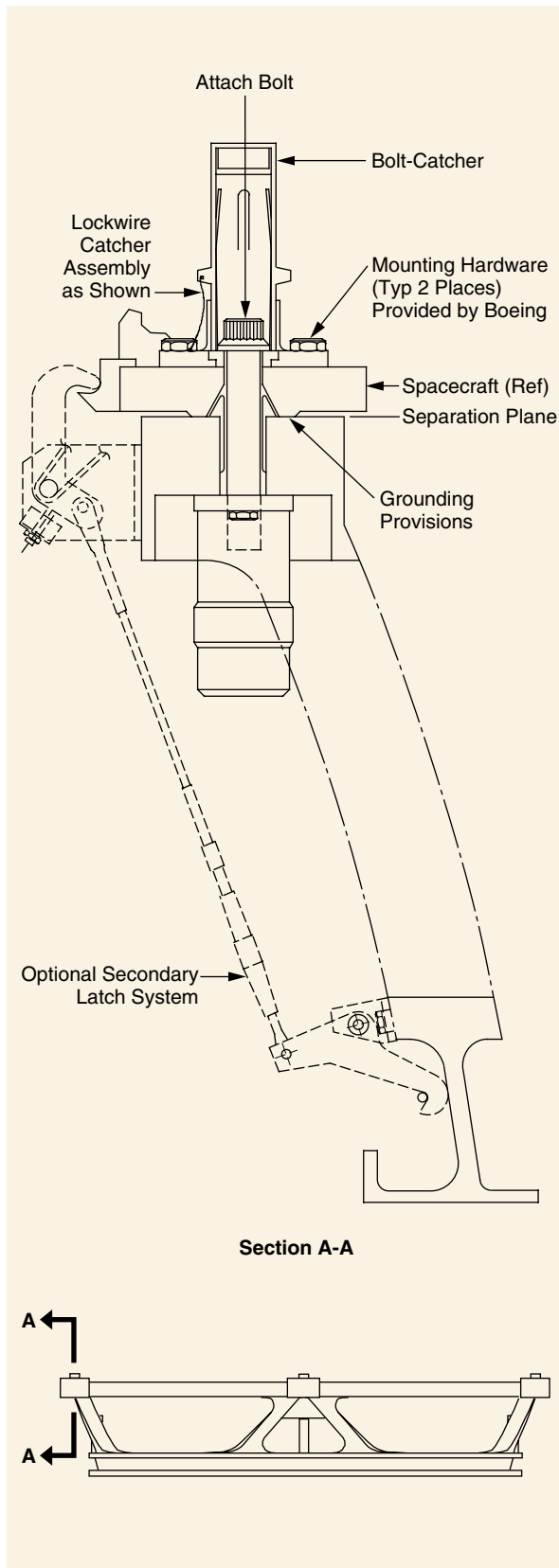
Figure 5-30. 6915 PAF Spacecraft Assembly
