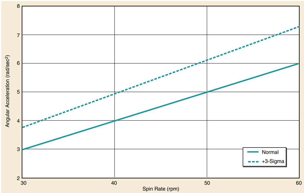
Figure 4-29. Maximum Expected Angular Acceleration vs. Spin Rate—Star-37FM
