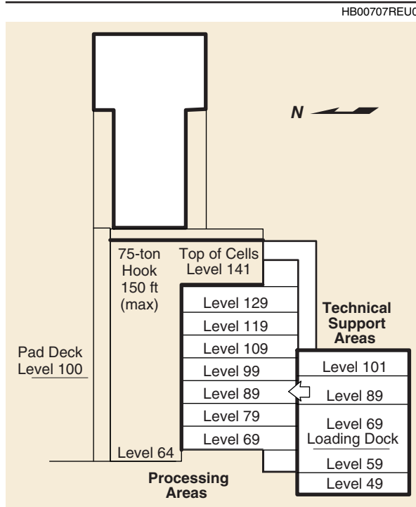
Figure 7-19. California Spaceport—IPF Cross-Sectional View
