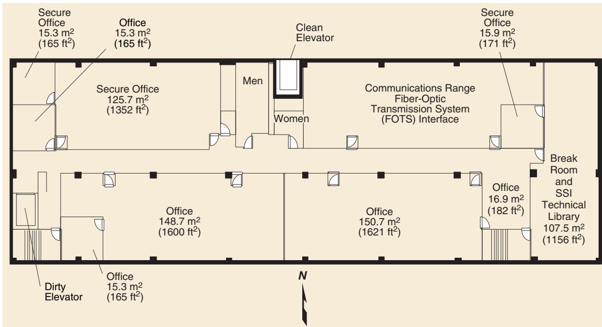
Figure 7-23. California Spaceport—Level 101 Technical Support Area
