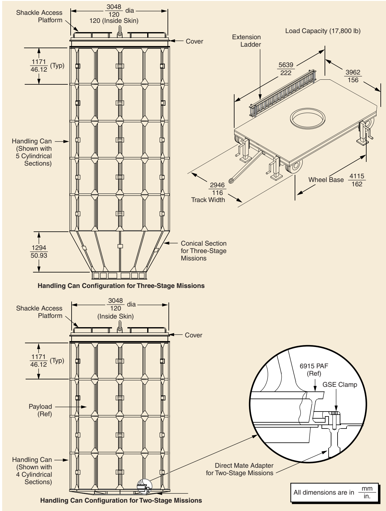
Figure 7-24. Second-Stage Assembly Ground Handling Can and Transporter
