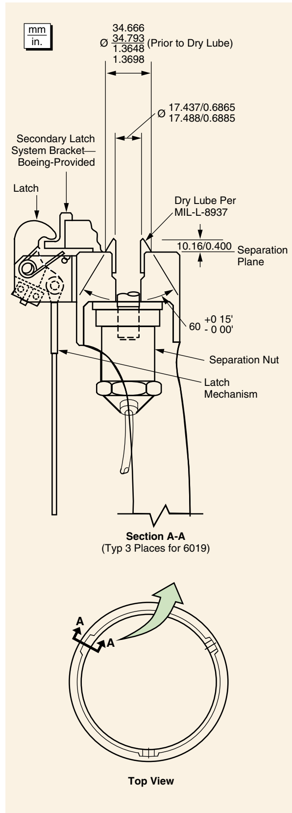
Figure 5-25. 6019 PAF Detailed Dimensions
