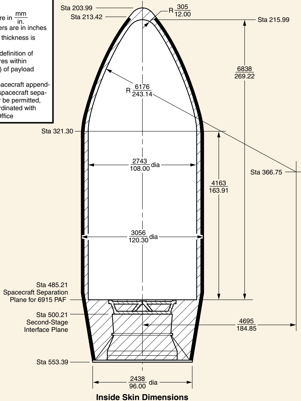
Figure 3-8. Payload Static Envelope, 3-m (10-ft)-dia Fairing, Two-Stage Configuration (6915 PAF)
