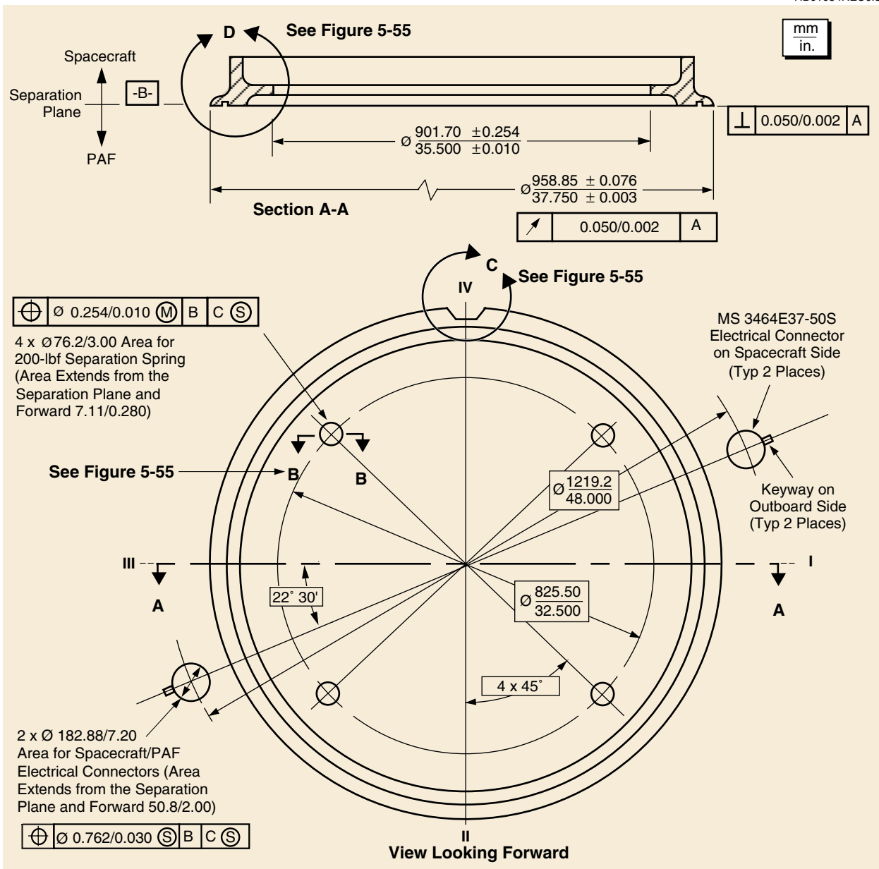
Figure 5-54. Dimensional Constraints on Spacecraft Interface to 37C PAF
