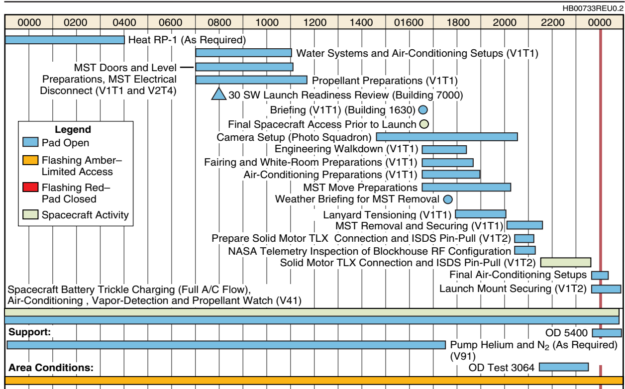
Figure 7-47. Typical Countdown Preparations (T-1 Day)
