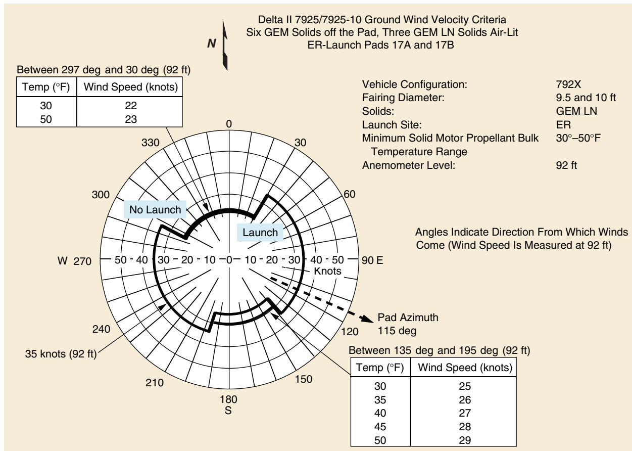
Figure 6-25. Delta II 792X Ground Wind Velocity Criteria, SLC-17
