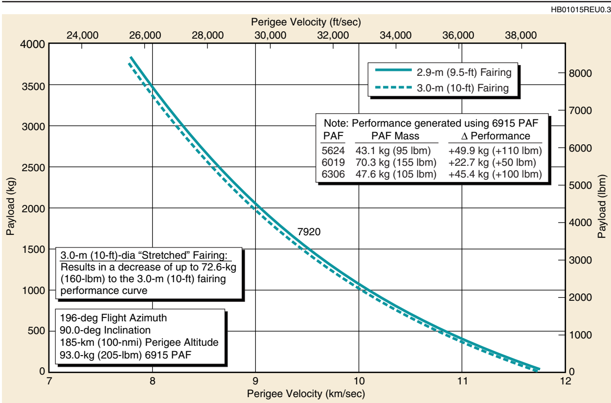
Figure 2-27. Delta II 7920 Vehicle, Two-Stage Perigee Velocity Capability—Western Launch Site
