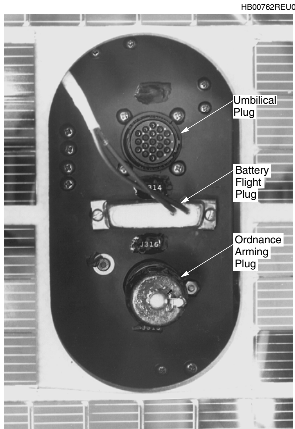
Figure 5-63. Typical Spacecraft Umbilical Connector
