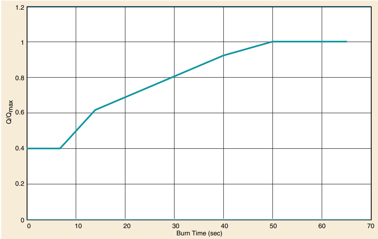
Figure 4-13. Predicted Star-37FM Plume Radiation at the Spacecraft Separation Plane vs. Burn Time
