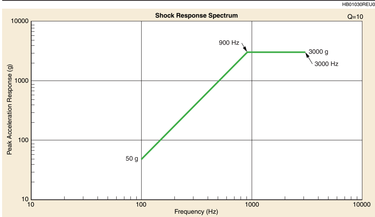
Figure 4-25. Maximum Flight Spacecraft Interface Shock Environment 5624 Payload Attach Fitting
