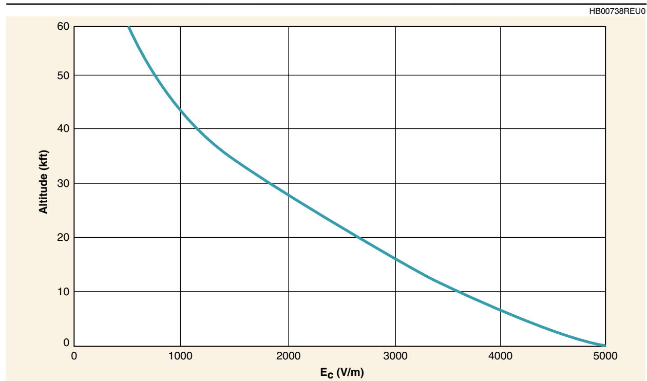
Figure A-1. Instantaneous Critical Electric Field, E_C , vs Altitude
