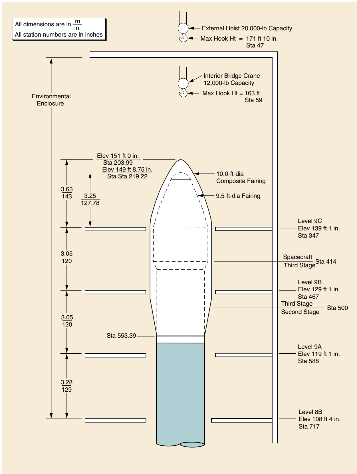
Figure 6-18. Environmental Enclosure Work Levels
