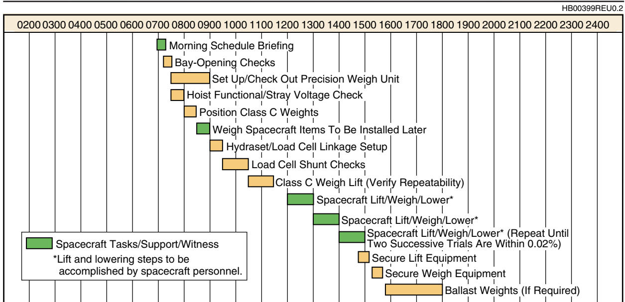
Figure 6-27. Typical Spacecraft Weighing (T-11 Day)
