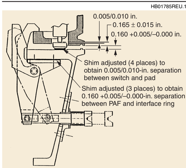
Figure 5-39. 6306 PAF Separation Switch Pad Interface
