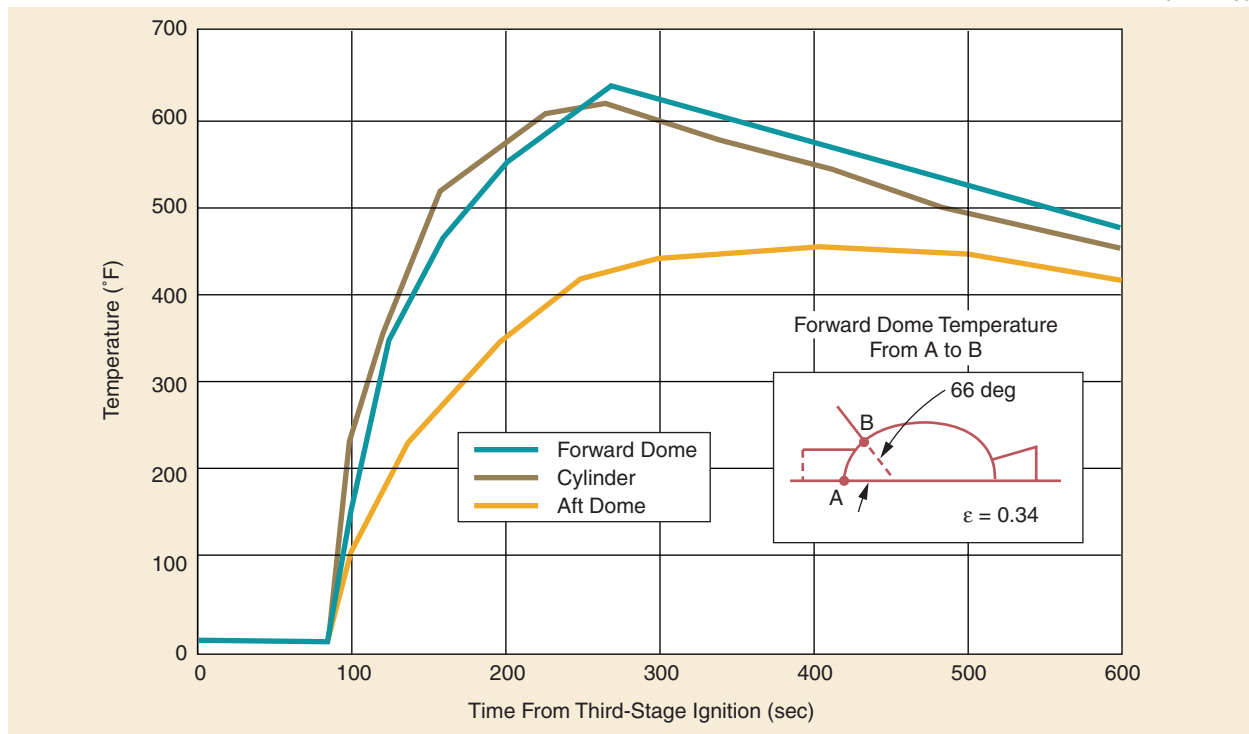
Figure 4-14. Star-48B Motor Case Soakback Temperature for Payload Mass Greater Than 910 kg (2006 lb)
