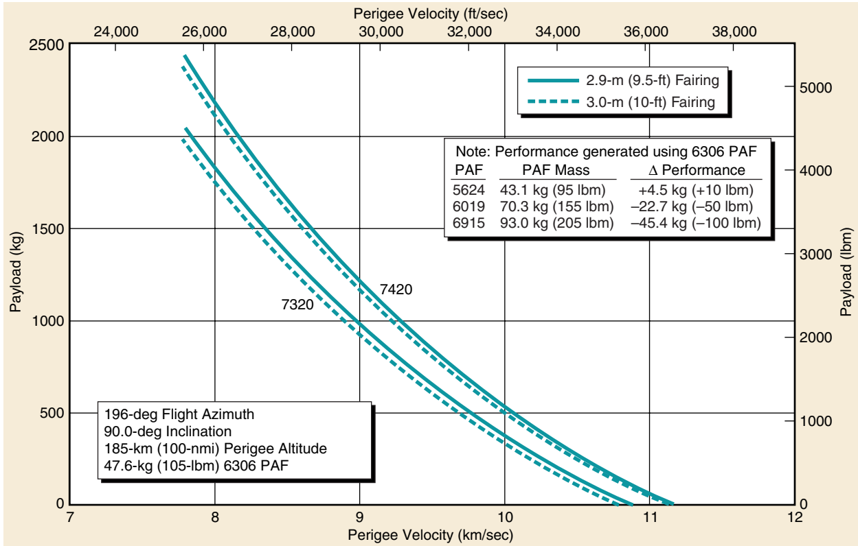
Figure 2-14. Delta II 7320/7420 Vehicle, Two-Stage Perigee Velocity Capability—Western Launch Site
