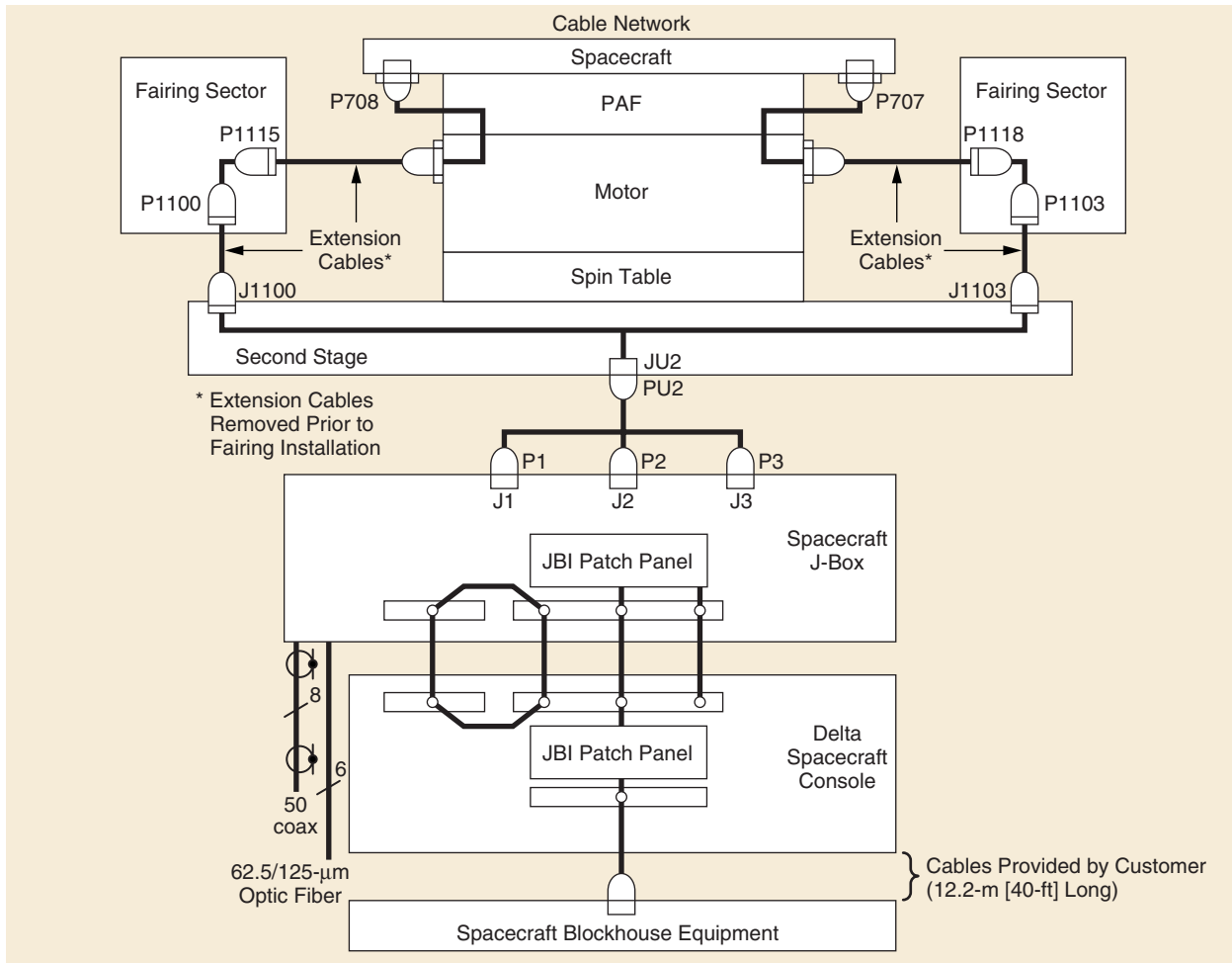
Figure 5-62. Typical Payload-to-Blockhouse Wiring Diagram for Three-Stage Missions at SLC-2
