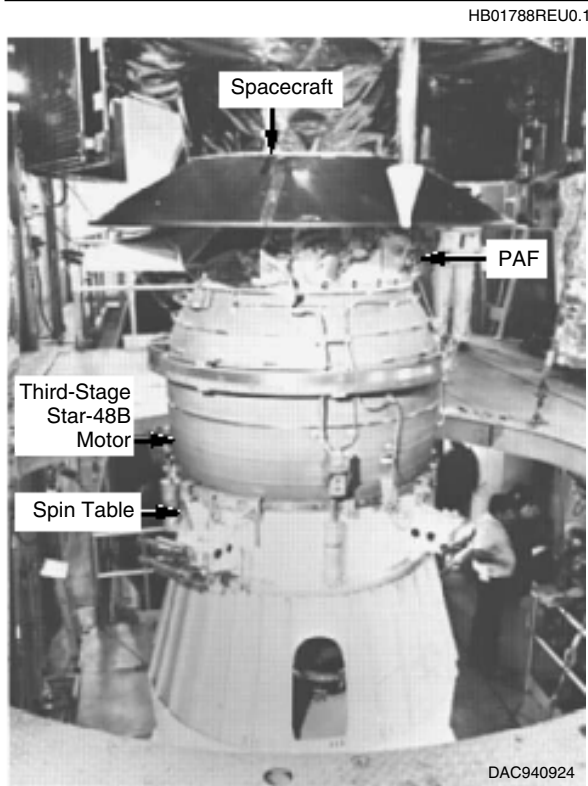
Figure 5-3. Delta II Third Stage
