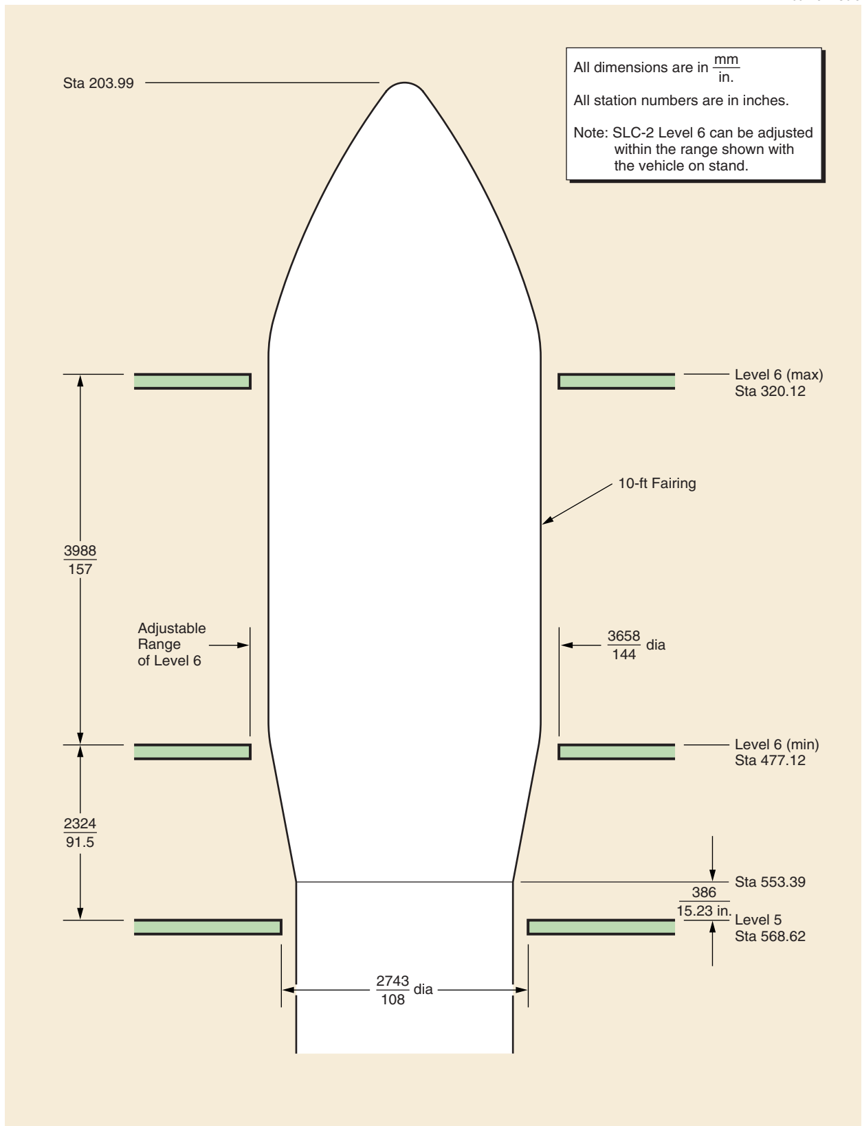
Figure 7-29. Spacecraft Work Levels in SLC-2 Mobile Service Tower—VAFB
