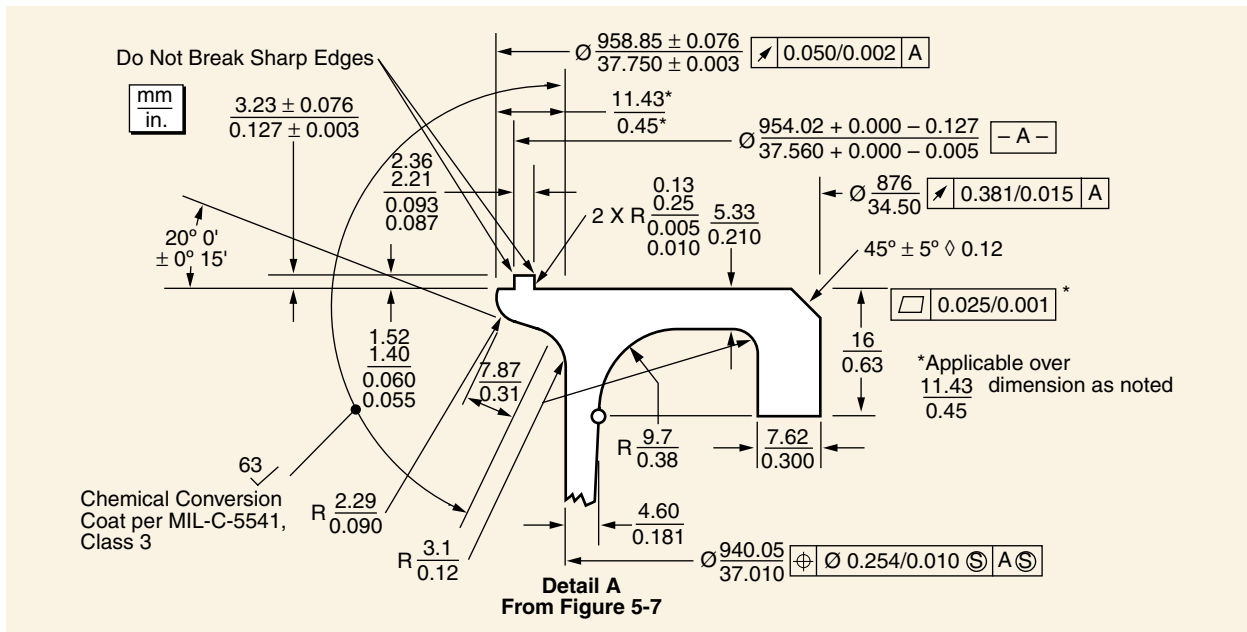
Figure 5-11. 3712B PAF Detailed Dimensions
