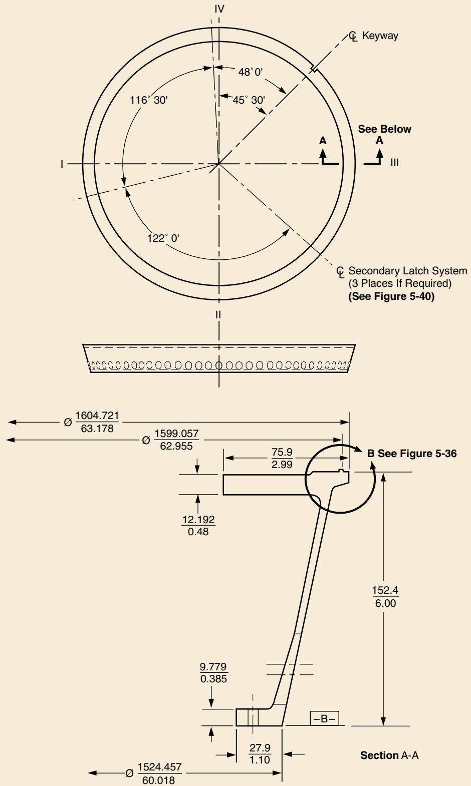
Figure 5-35. 6306 PAF Detailed Dimensions
