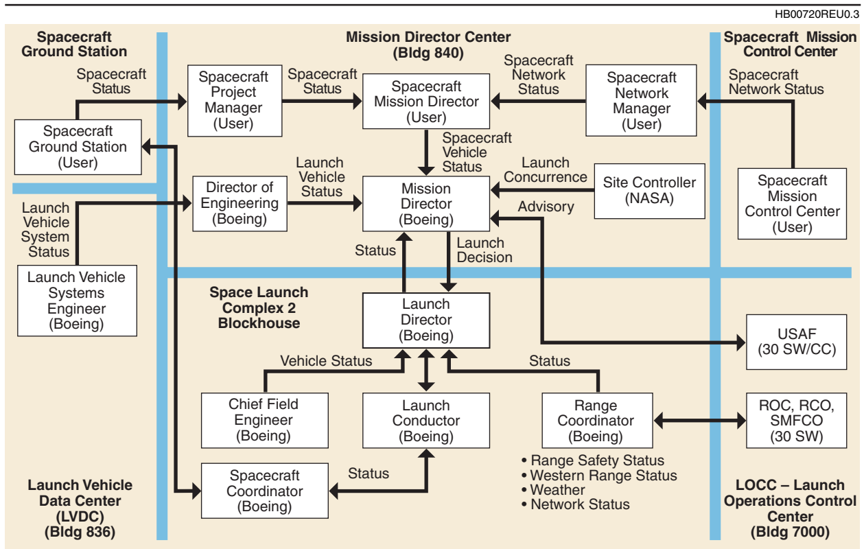
Figure 7-35. Launch Decision Flow for Commercial Missions—Western Range
