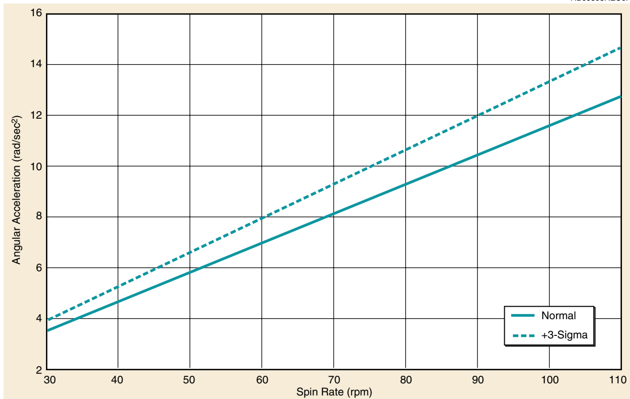
Figure 4-28. Maximum Expected Angular Acceleration vs. Spin Rate—Star-48B
