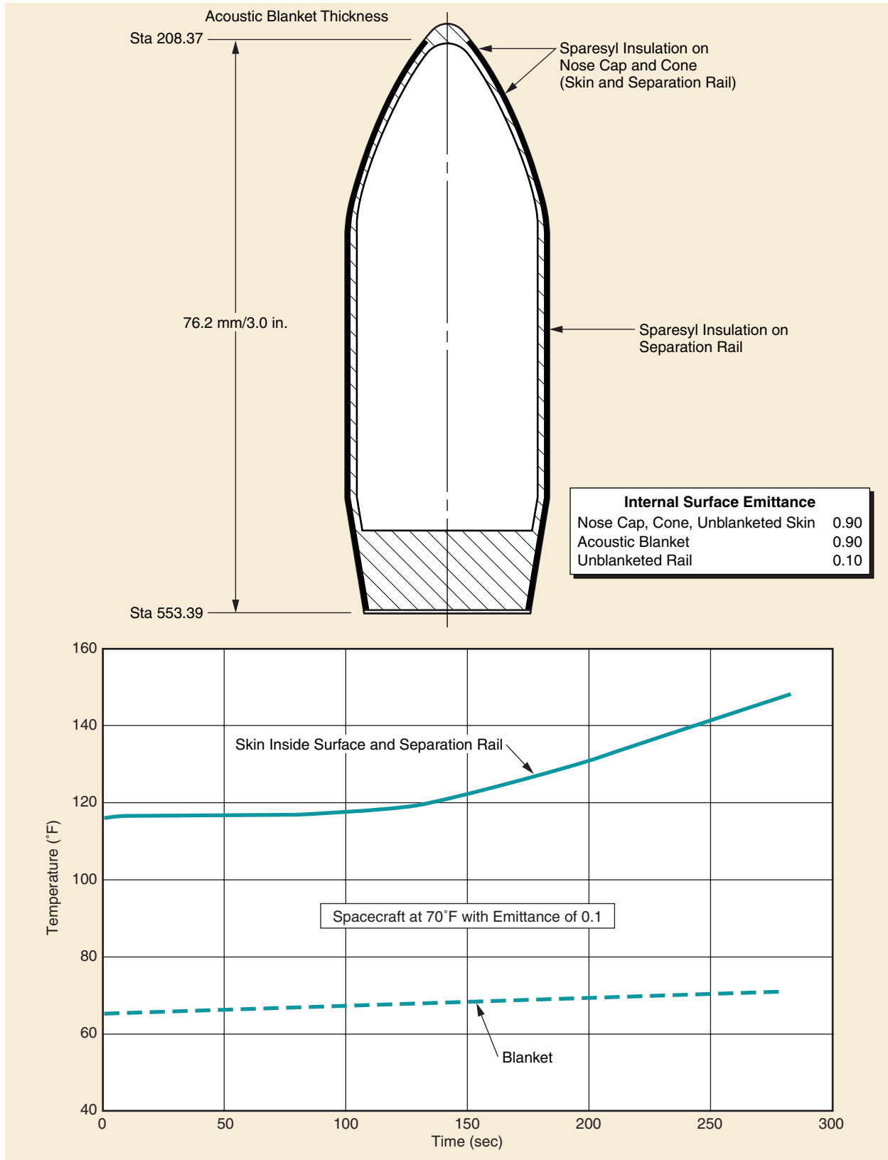
Figure 4-8. Predicted Maximum Internal Wall Temperature and Internal Surface Emittance (10-ft Fairing, Standard or Stretched)
