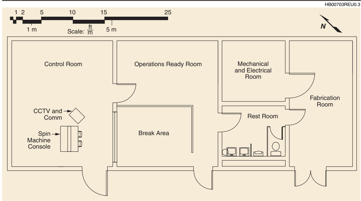
Figure 7-13. Control Room (Building 1605)
