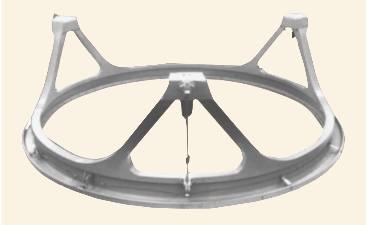
Figure 5-20. 6019 PAF Assembly
