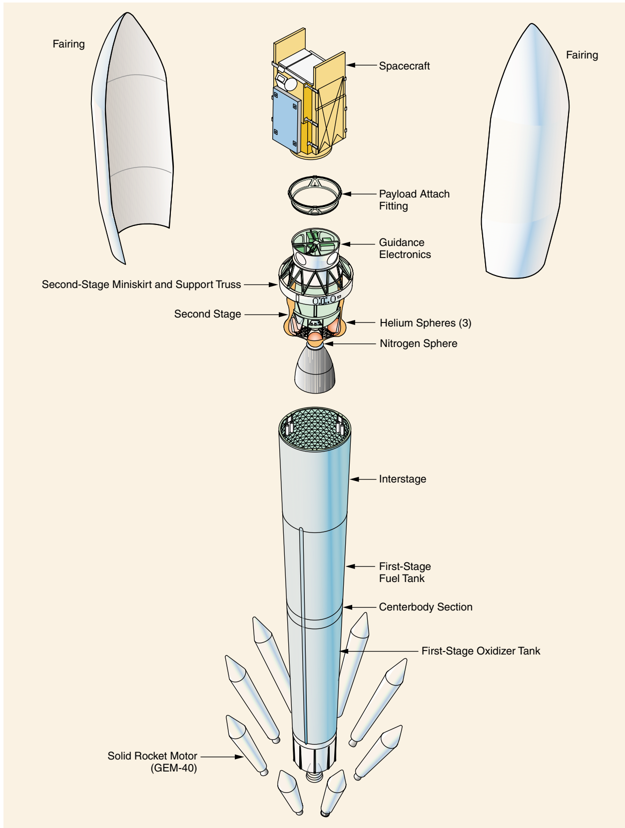
Figure 1-5. Delta 7920-10 Launch Vehicle
