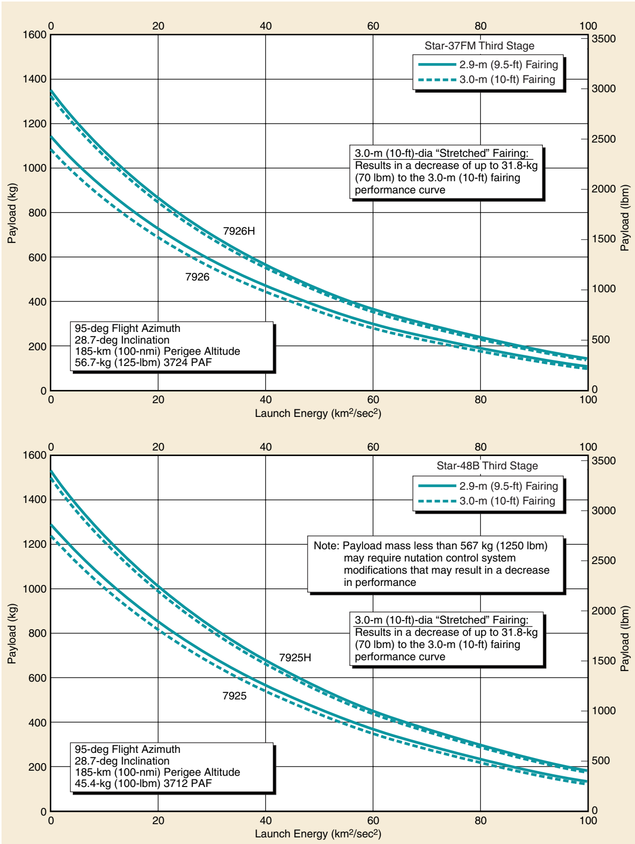
Figure 2-26. Delta II 792X/792XH Vehicle, Three-Stage Launch Energy Capability—Eastern Launch Site
