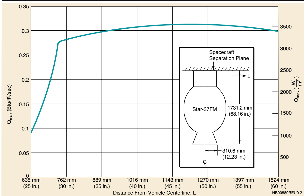
Figure 4-12. Predicted Star-37FM Plume Radiation at the Spacecraft Separation Plane vs. Radial Distance
