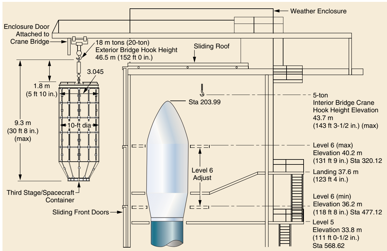
Figure 7-30. Whiteroom Elevations and Hook Heights—SLC-2 Mobile Service Tower
