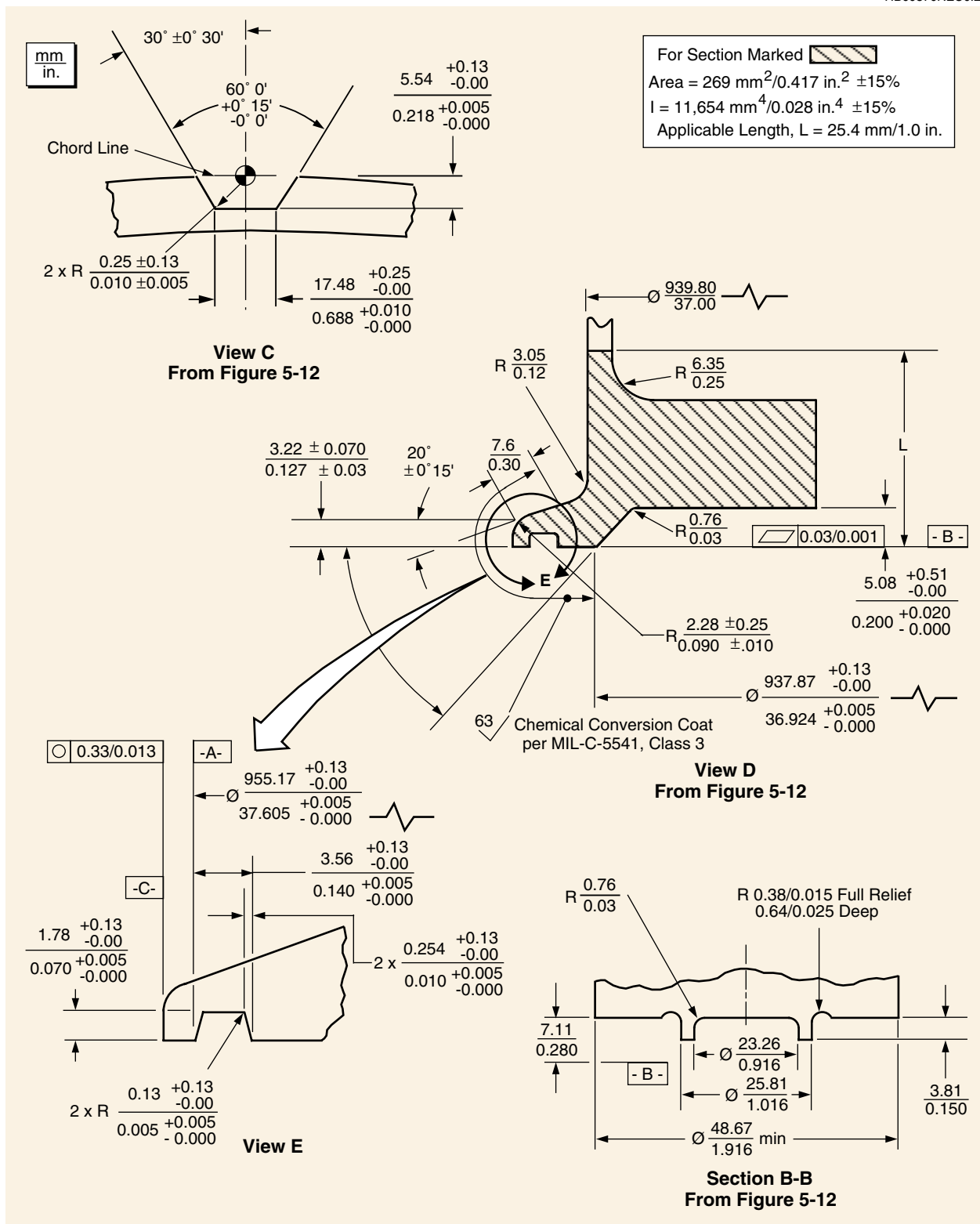
Figure 5-13. Dimensional Constraints on Spacecraft Interface to 3712B PAF (Views C, D, and E and Section B-B)
