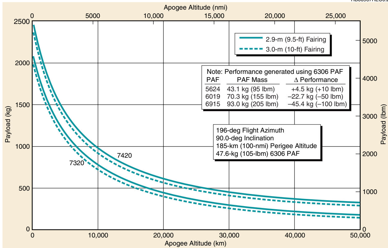
Figure 2-15. Delta II 7320/7420 Vehicle, Two-Stage Apogee Altitude Capability—Western Launch Site
