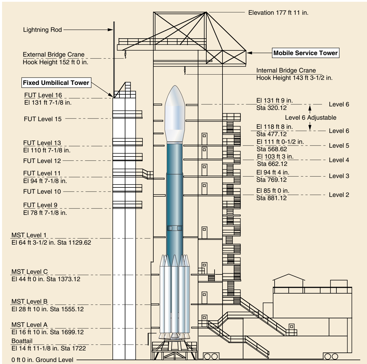
Figure 7-26. SLC-2 Mobile Service Tower/Fixed Umbilical Tower Elevations
