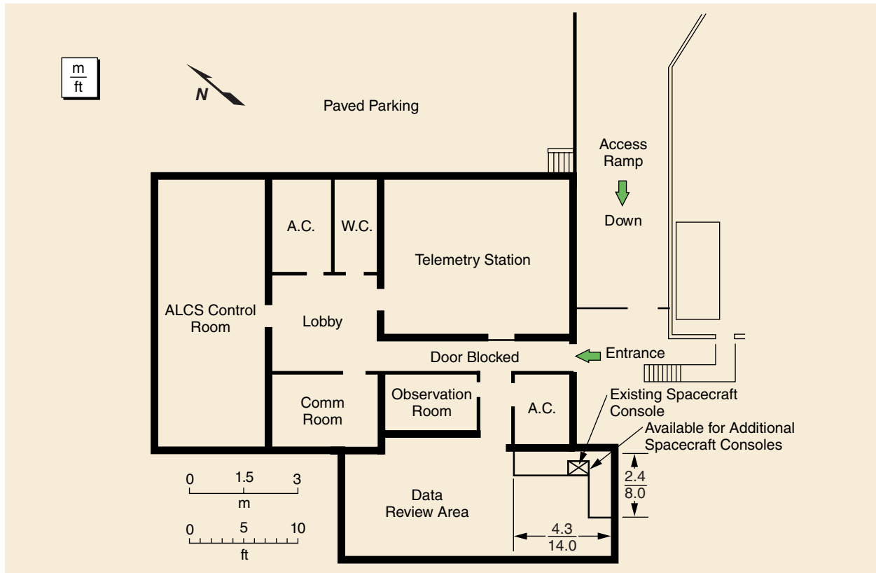
Figure 7-31. SLC-2 Blockhouse
