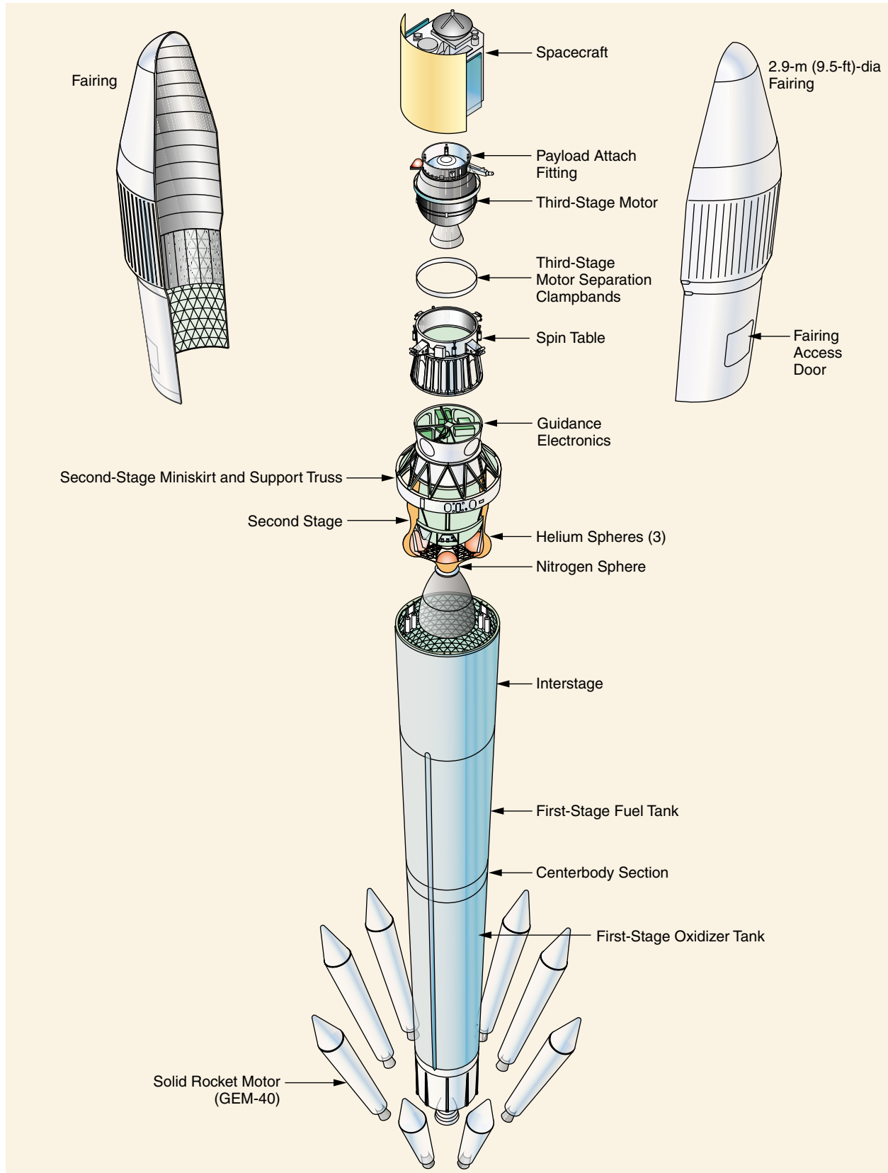
Figure 1-4. Delta 7925 Launch Vehicle
