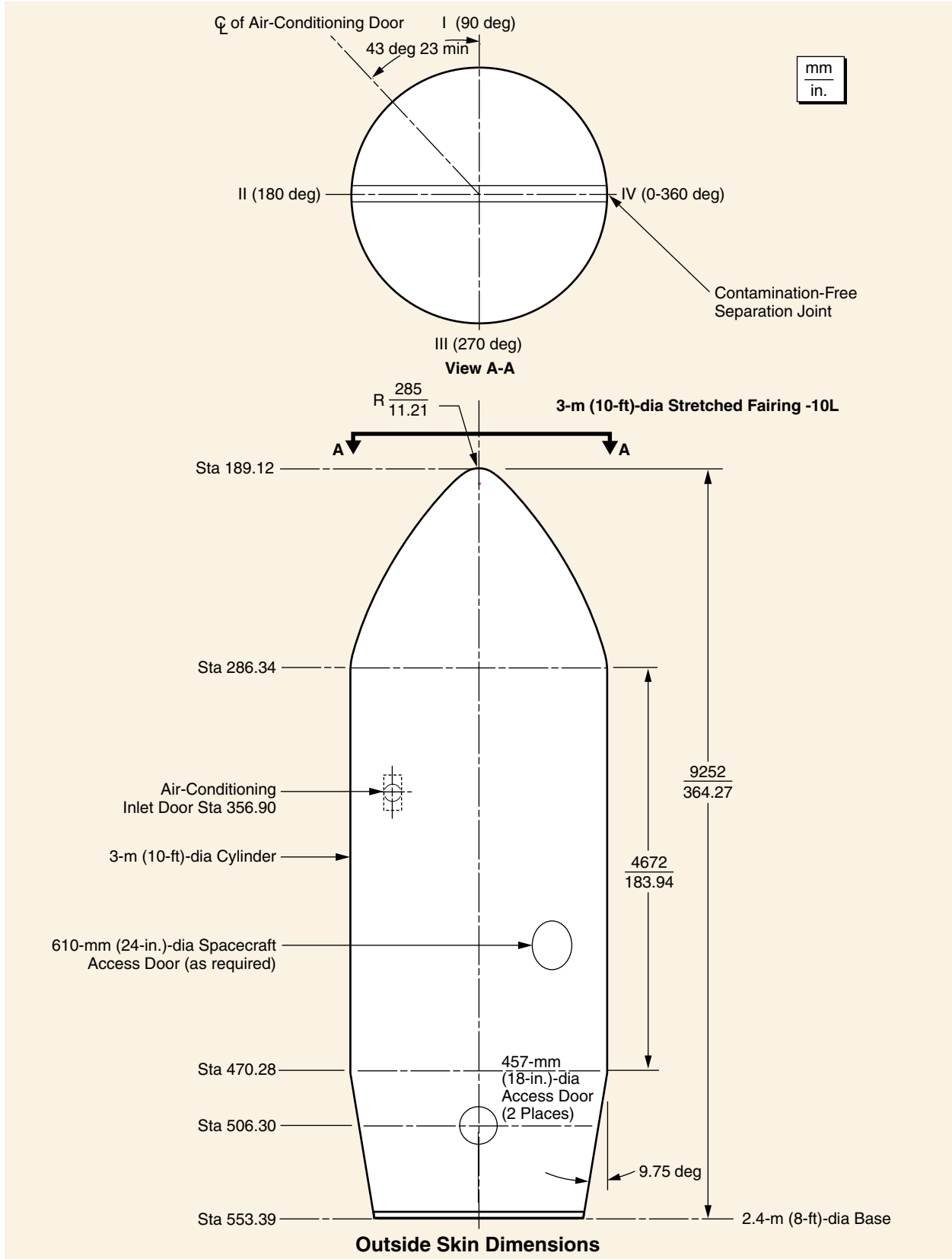
Figure 3-10. Profile, 3-m (10-ft)-dia Stretched Composite Fairing (-10L)
