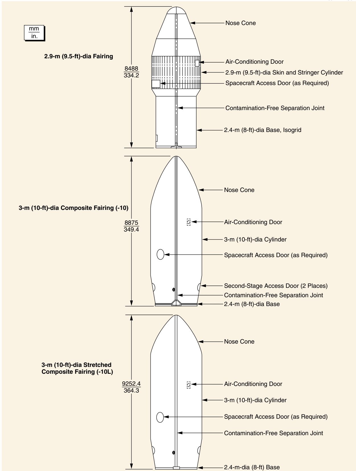
Figure 1-6. Delta II Payload Fairings
