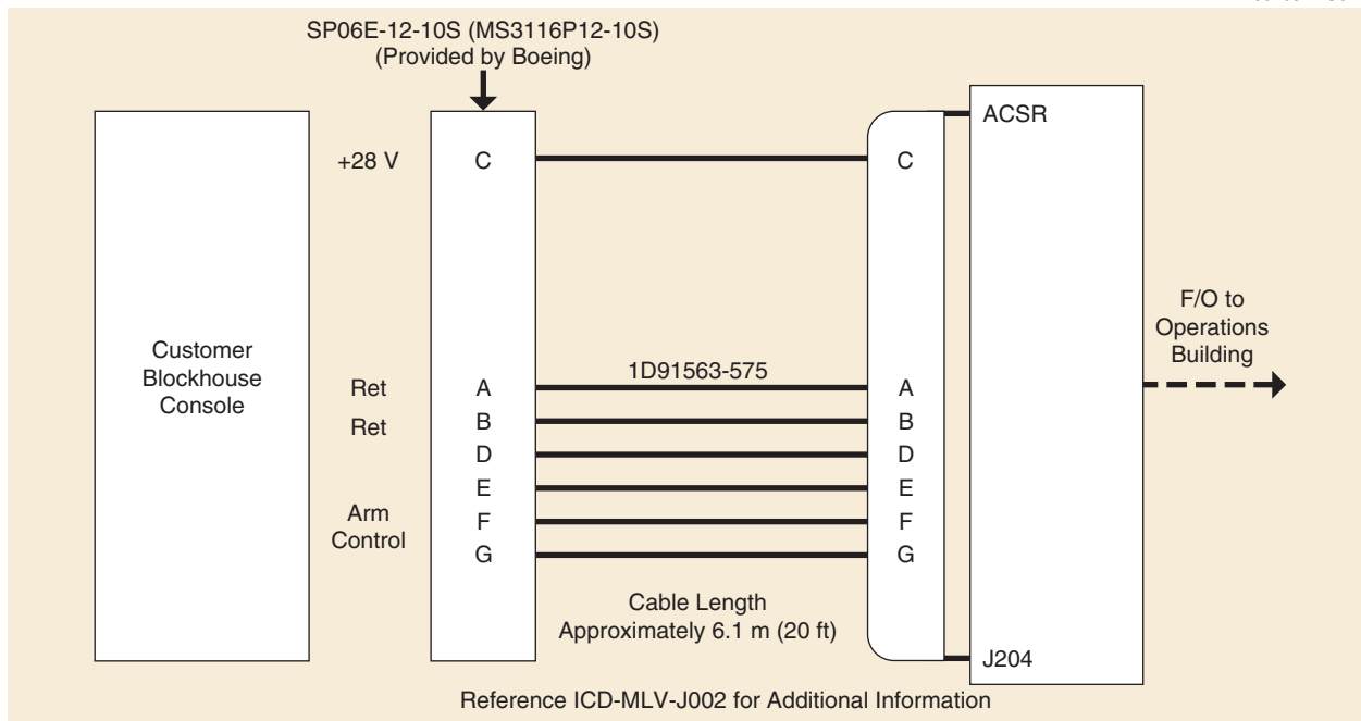
Figure 5-66. Blockhouse Spacecraft/Operation Safety Manager's Console Interface for SLC-17
