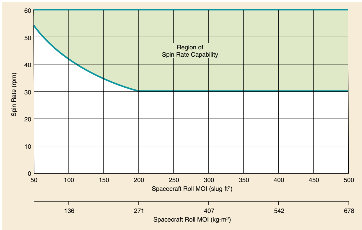
Figure 4-27. Delta II Star-37FM Spin Rate Capability
