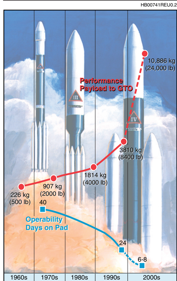
Figure 1-2. Performance and Operability of the Delta Family
