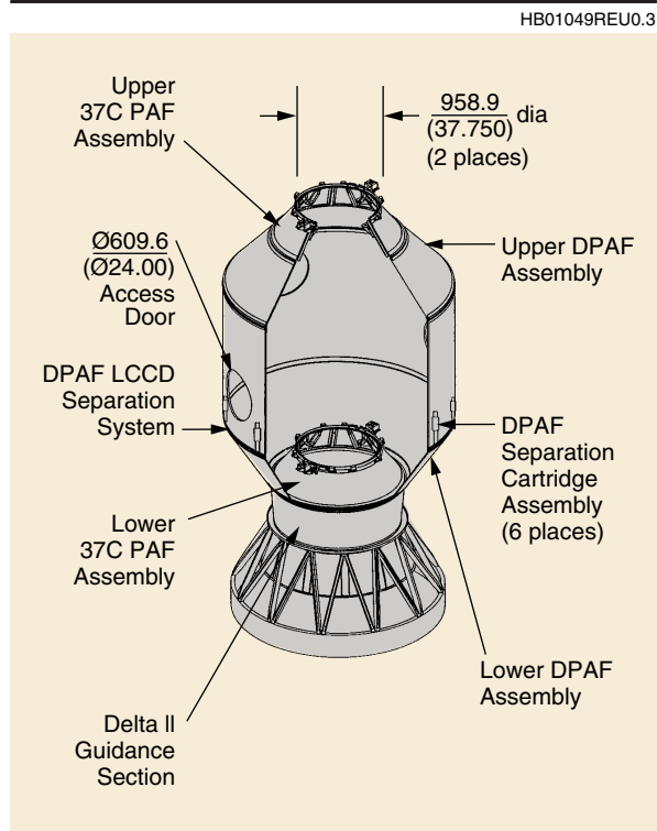
Figure 5-48. PAFs for Lower and Upper Payloads in Dual-Manifest
