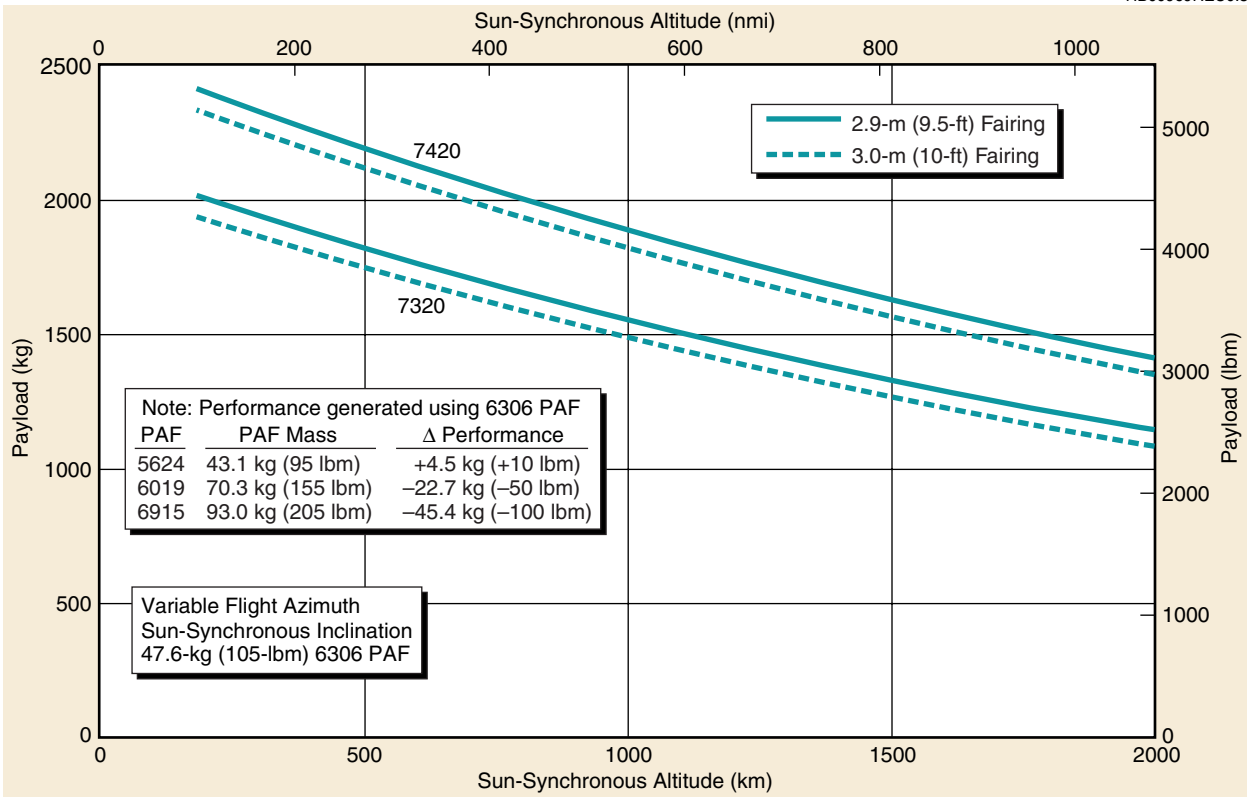
Figure 2-17. Delta II 7320/7420 Vehicle, Two-Stage Sun-Synchronous Capability—Western Launch Site
