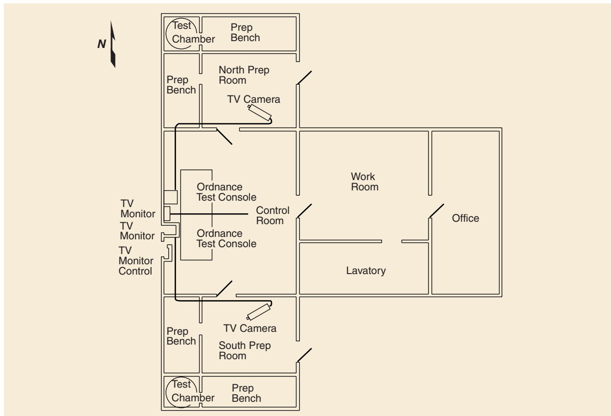
Figure 6-13. Electrical-Mechanical Testing Building Floor Plan
