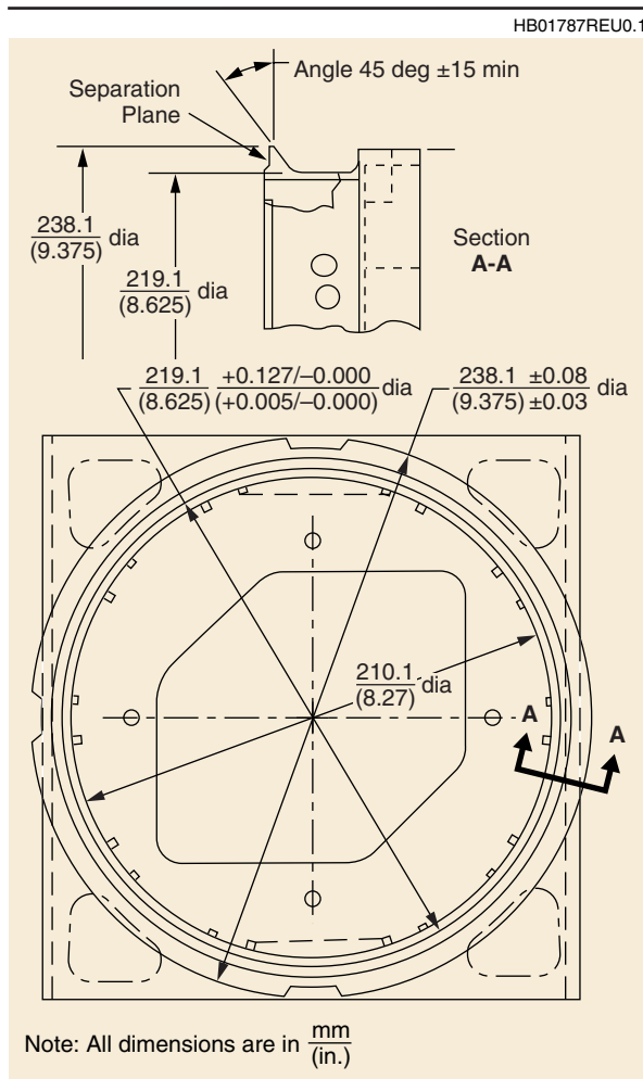
Figure 5-57. Separating Secondary Payload Standard Interface
