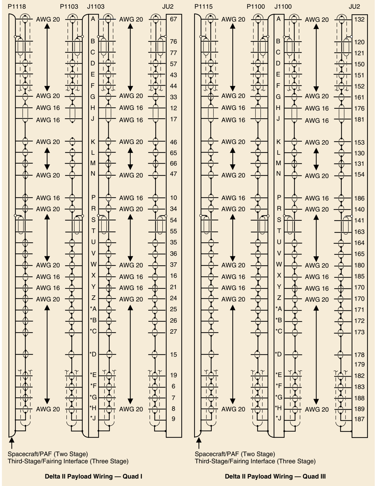
Figure 5-60. Typical Delta II Wiring Configuration
