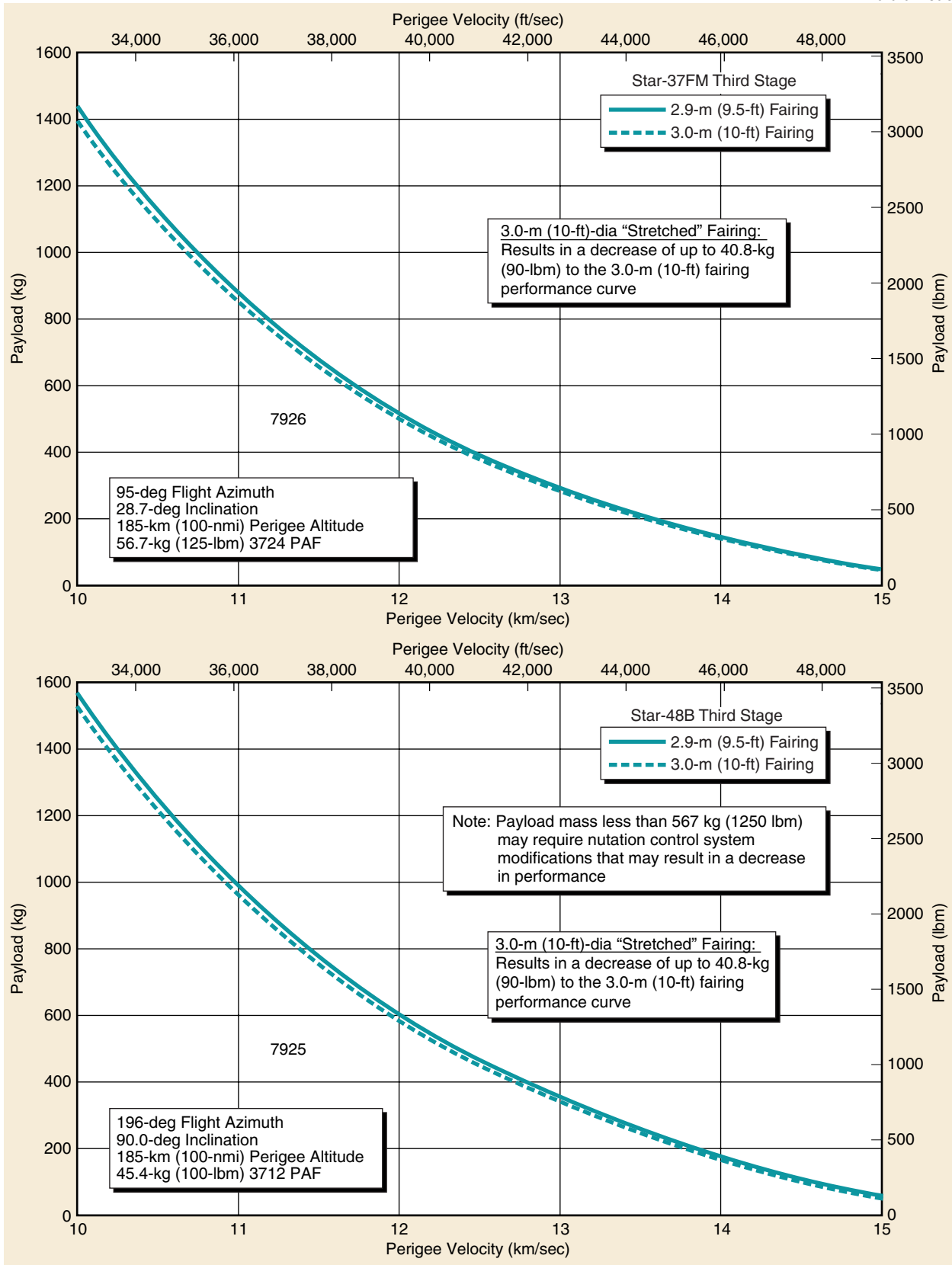
Figure 2-31. Delta II 792X Vehicle, Three-Stage Perigee Velocity Capability—Western Launch Site
