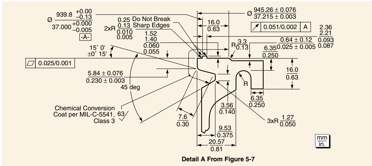
Figure 5-8. 3712A PAF Detailed Dimensions
