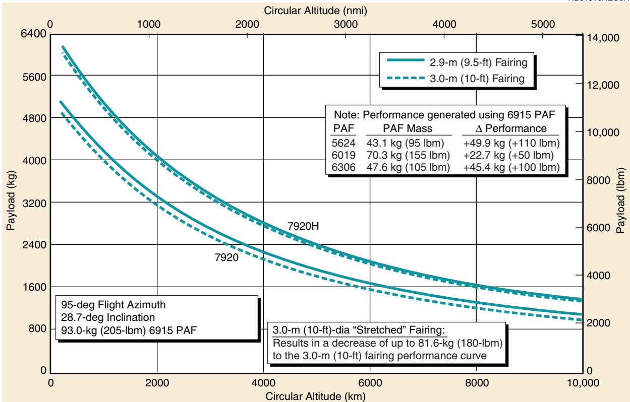
Figure 2-22. Delta II 7920/7920H Vehicle, Two-Stage Circular Orbit Altitude Capability—Eastern Launch Site
