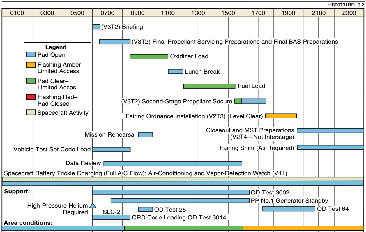
Figure 7-45. Typical Second-Stage Propellant Loading (T-3 Day)
