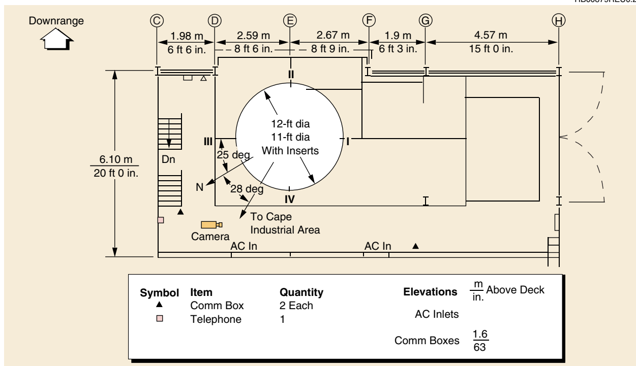
Figure 6-21B. Level 9C Floor Plan, Pad 17B
