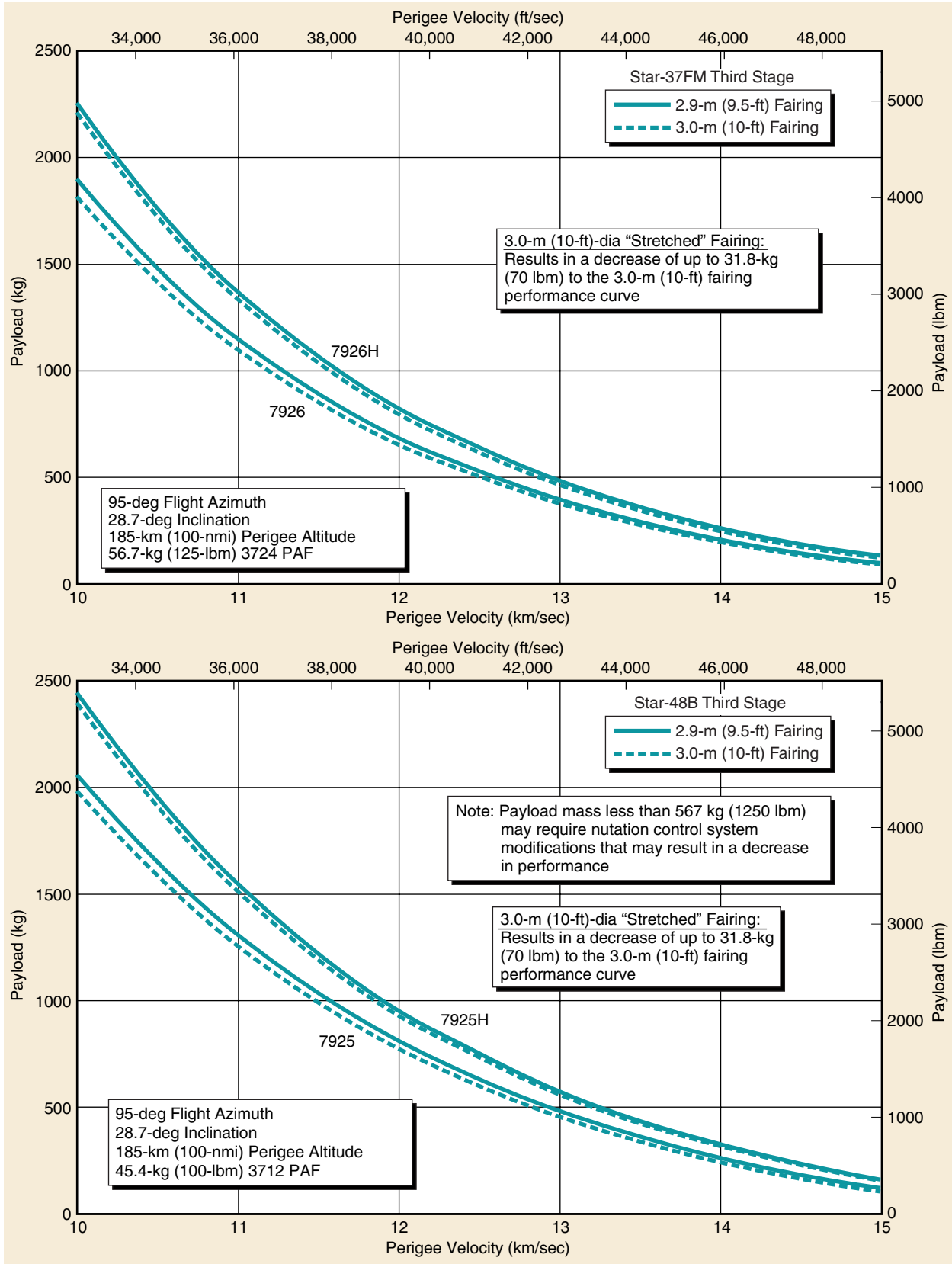
Figure 2-23. Delta II 792X/792XH Vehicle, Three-Stage Perigee Velocity Capability—Eastern Launch Site
