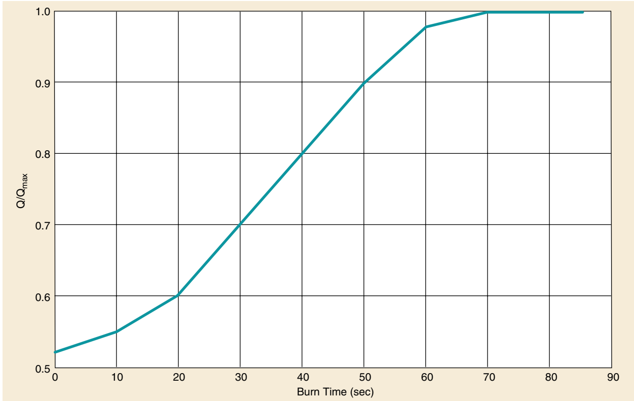
Figure 4-11. Predicted Star-48B Plume Radiation at the Spacecraft Separation Plane vs. Burn Time
