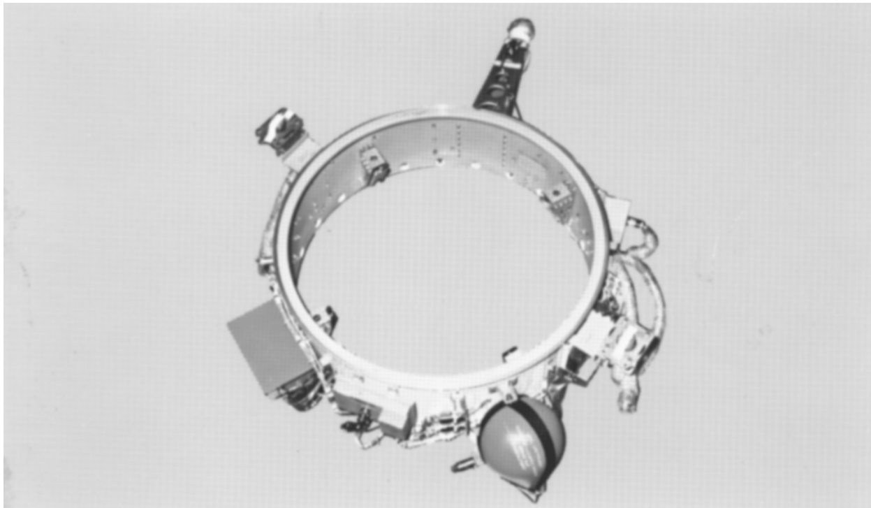
Figure 5-2. 3712 Payload Attach Fitting (PAF)
