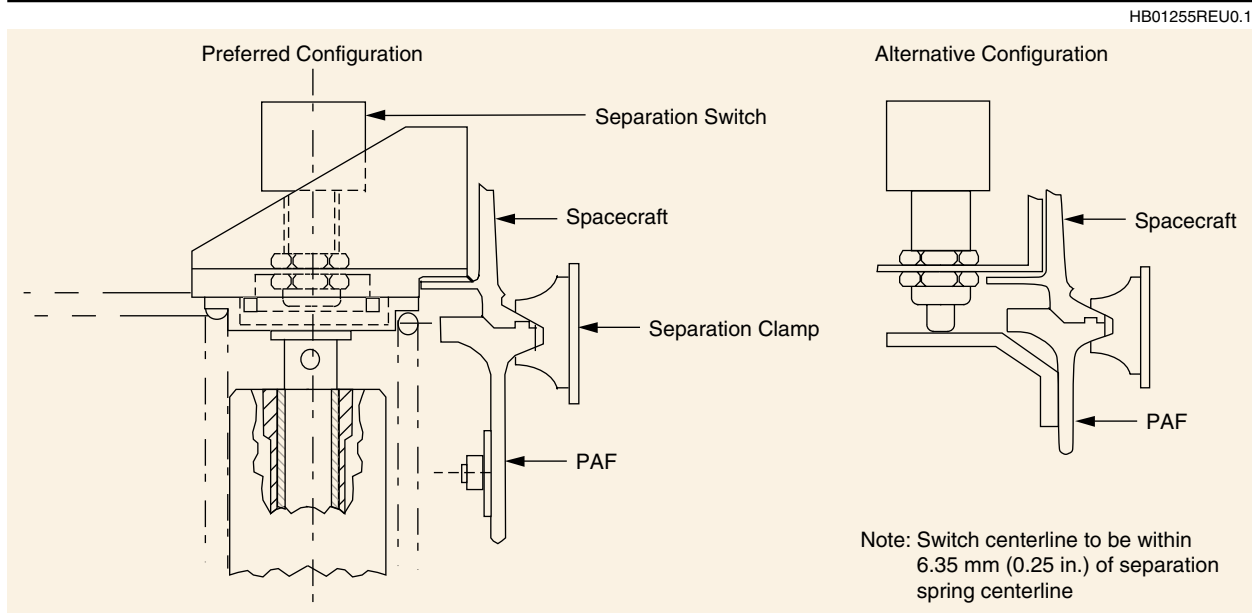
Figure 5-4. Typical Spacecraft Separation Switch and PAF Switch Pad
