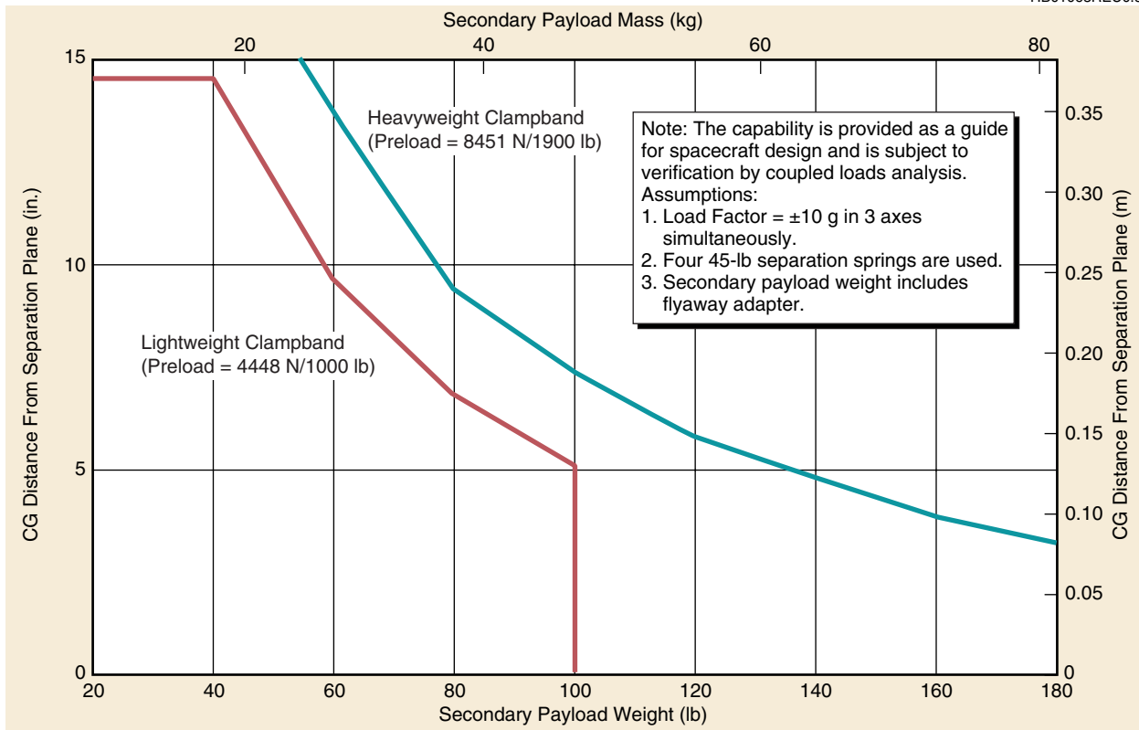
Figure 5-59. Capability of Separating Secondary Payloads
