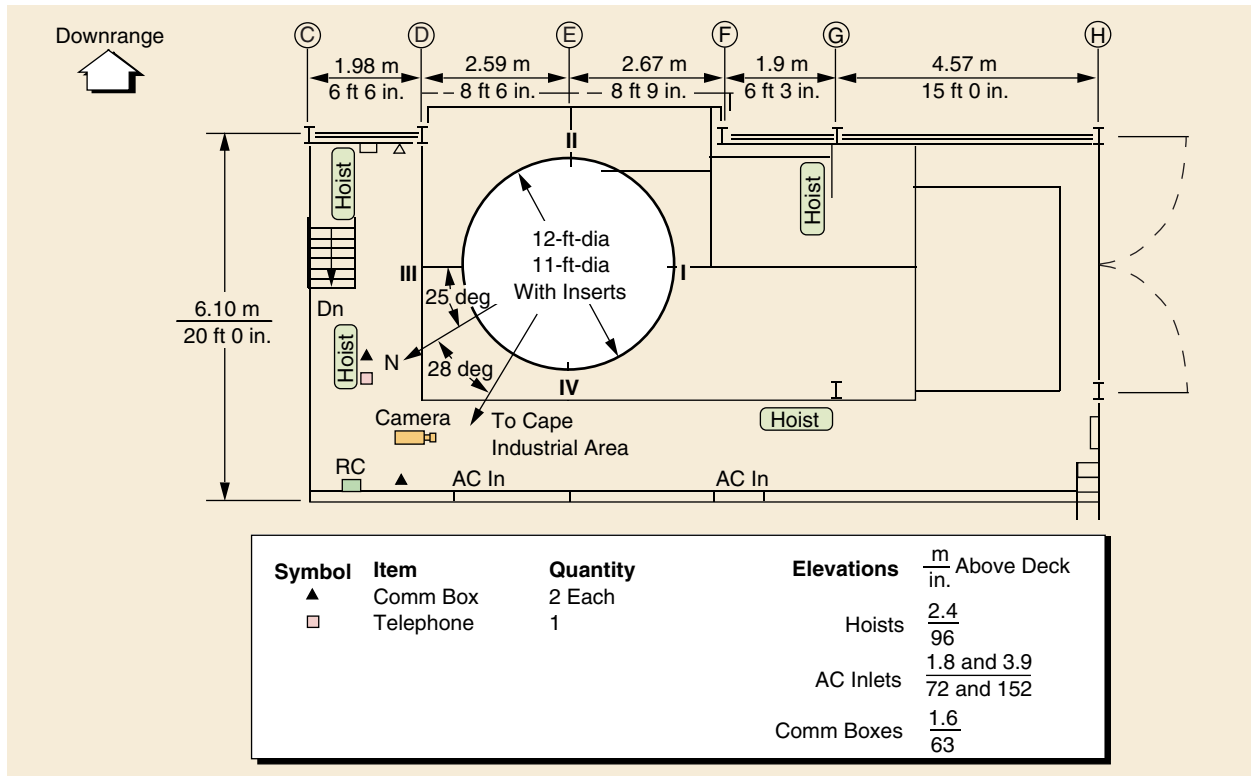
Figure 6-21A. Level 9C Floor Plan, Pad 17A
