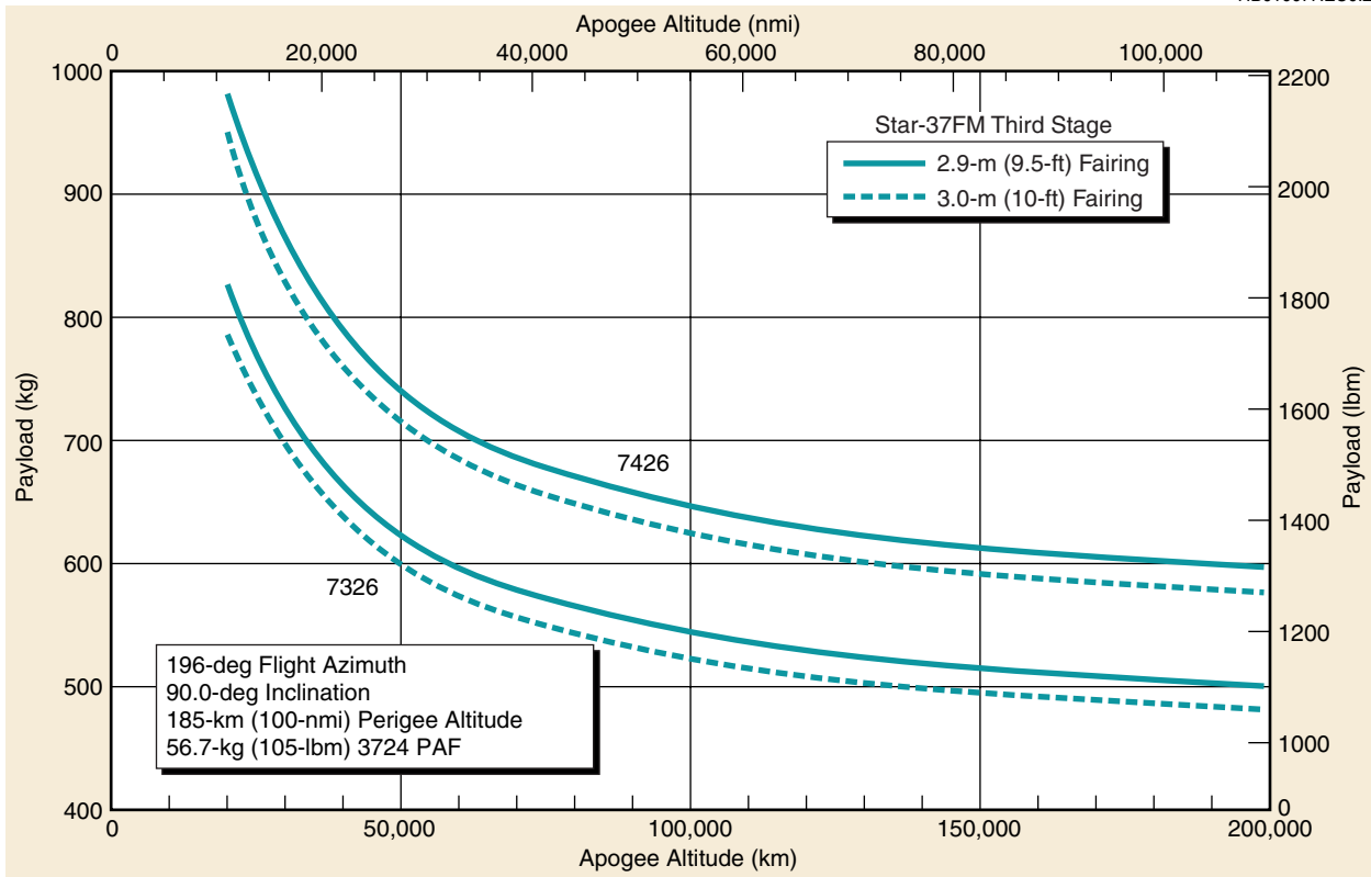
Figure 2-19. Delta II 7326/7426 Vehicle, Three-Stage Apogee Altitude Capability—Western Launch Site
