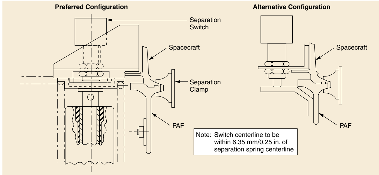
Figure 5-65. Typical Spacecraft Separation Switch and PAF Switch Pad
