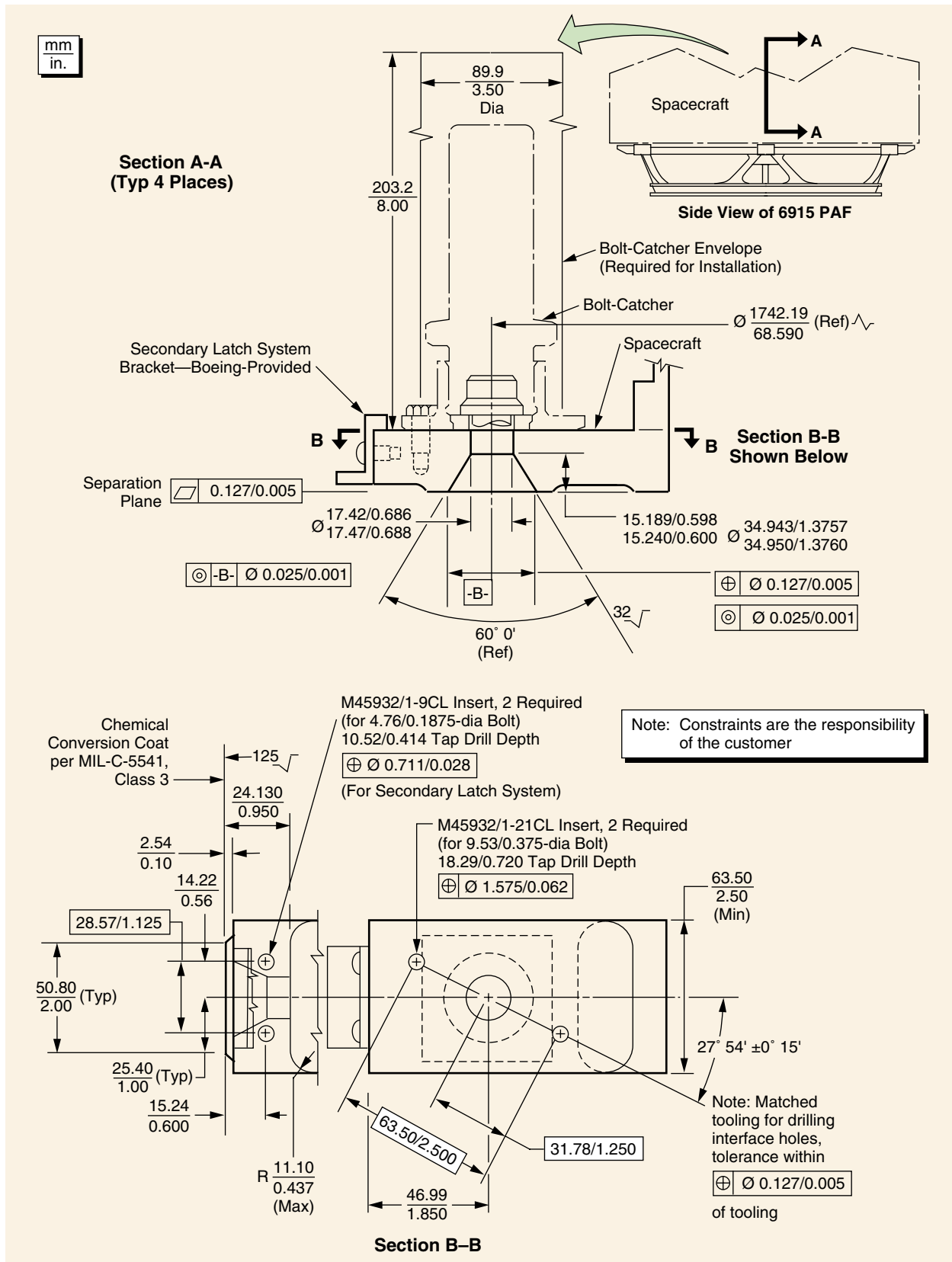
Figure 5-29. Dimensional Constraints on Spacecraft Interface to 6915 PAF
