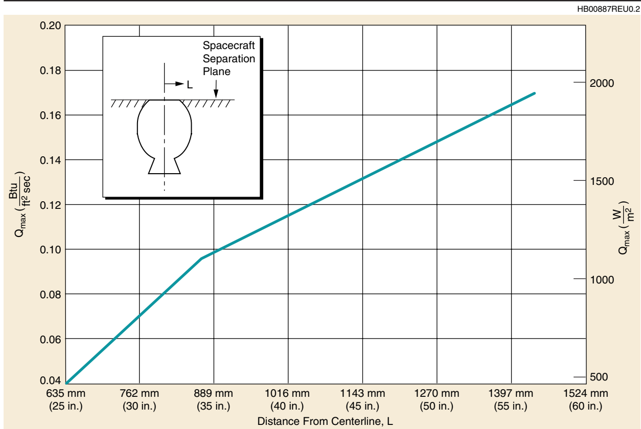
Figure 4-10. Predicted Star-48B Plume Radiation at the Spacecraft Separation Plane vs. Radial Distance
