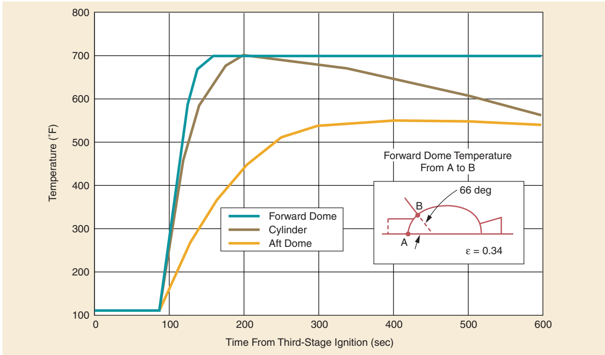
Figure 4-15. Star-48B Motor Case Soakback Temperature for Payload Mass Between 460 kg (1014 lb) and 910 kg (2006 lb)
