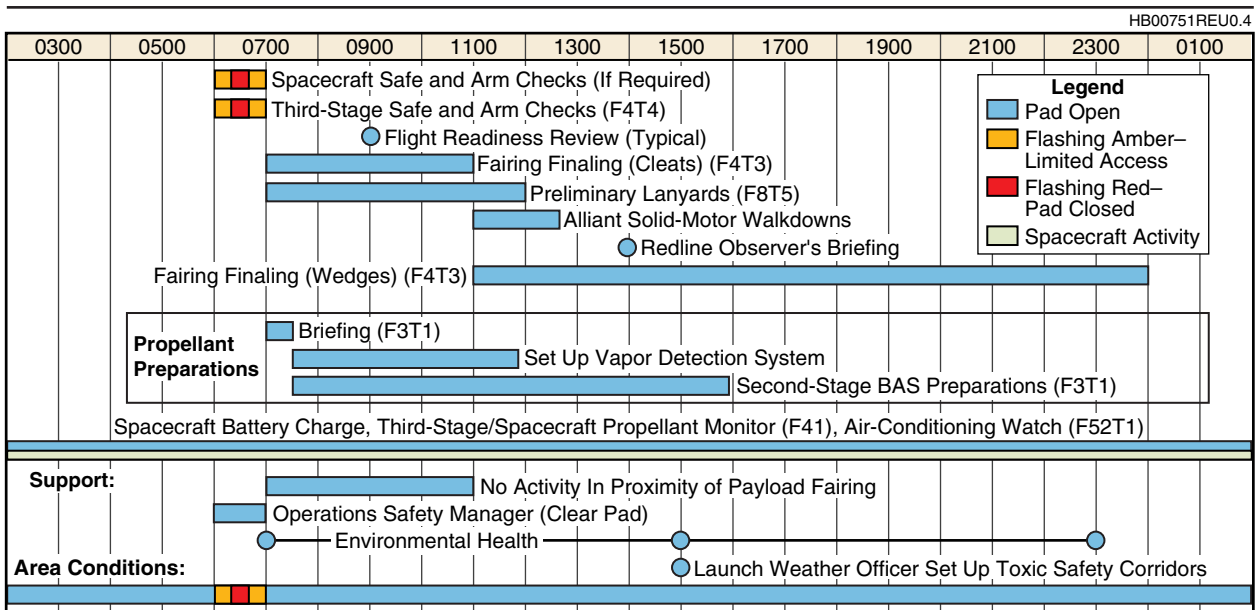
Figure 6-35. Typical Propellant Loading Preparations (T-3 Day)
