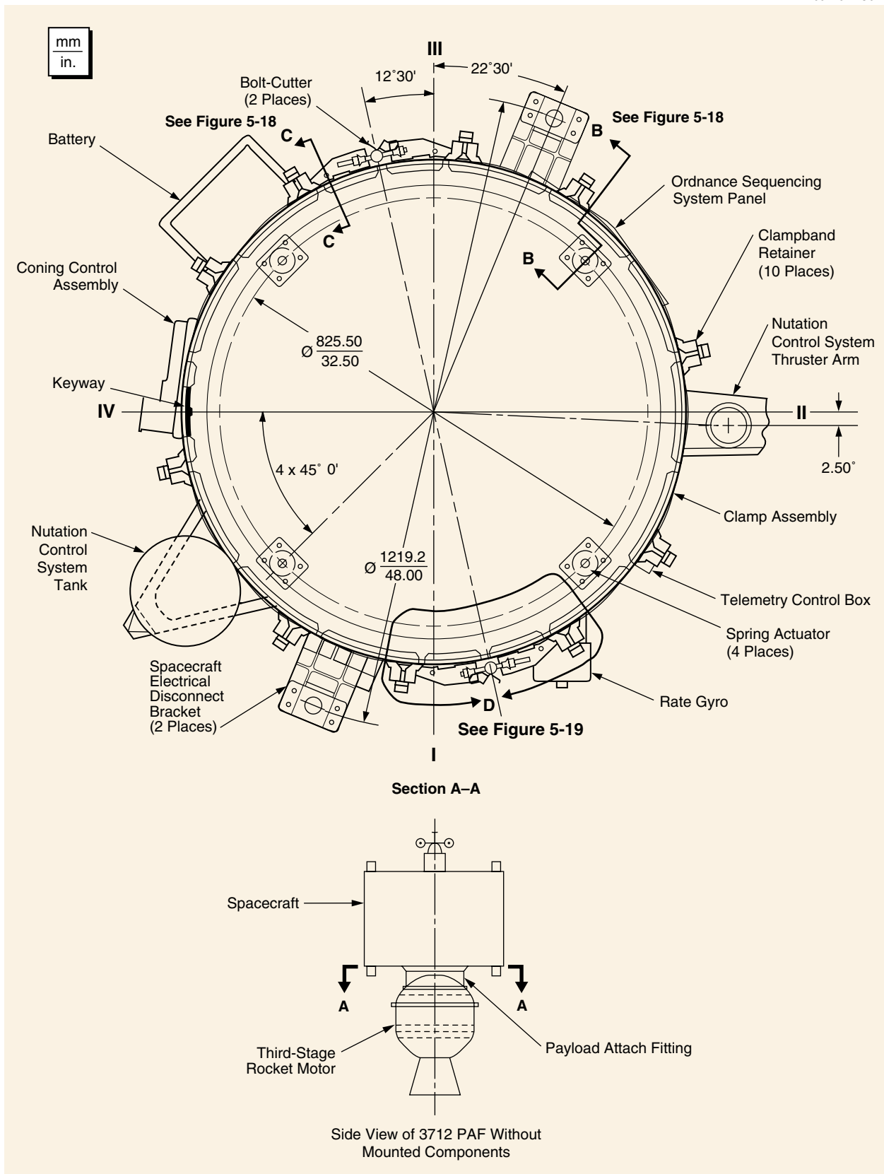
Figure 5-17. 3712 PAF Interface
