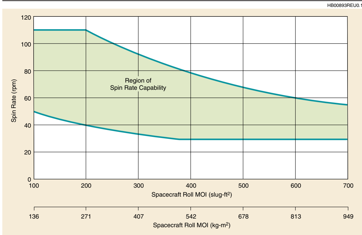
Figure 4-26. Delta II Star-48B Spin Rate Capability
