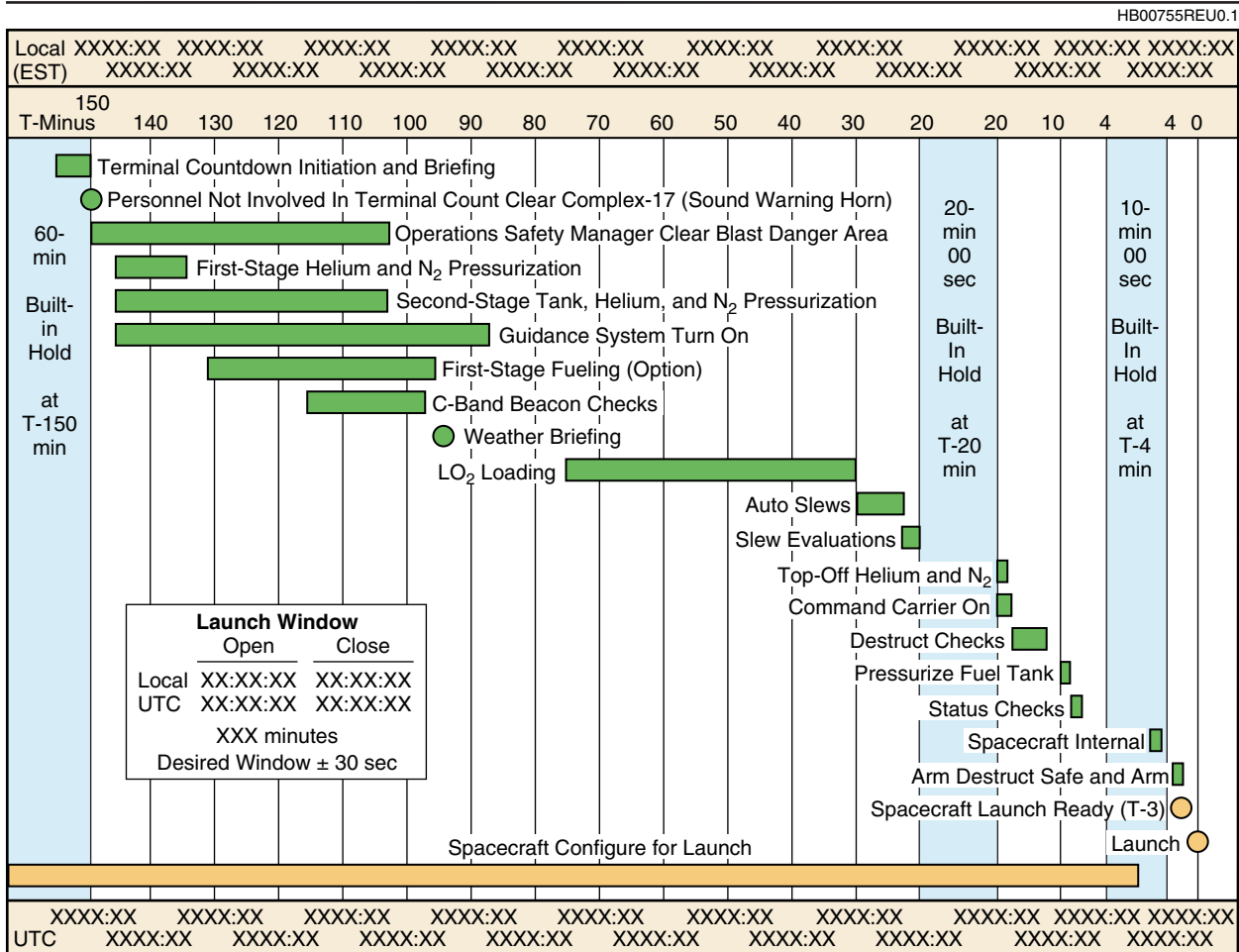
Figure 6-39. Typical Terminal Countdown (T-0 Day)
