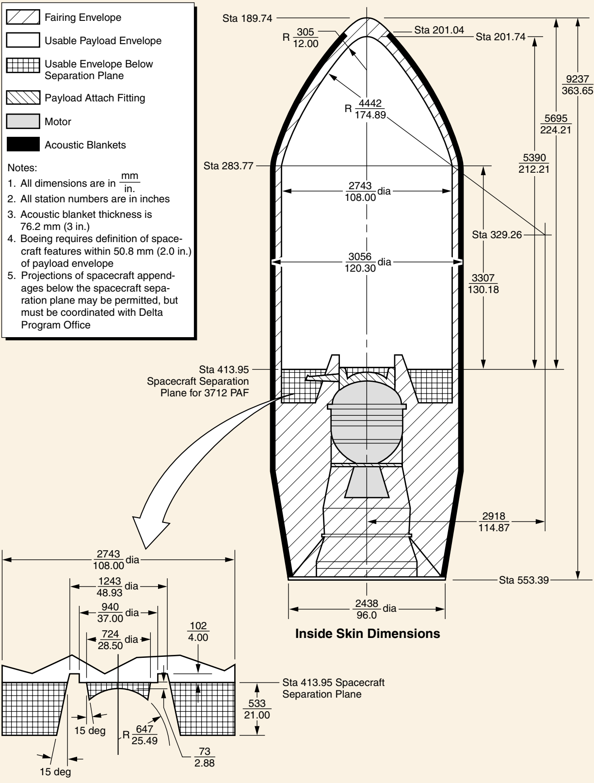
Figure 3-11. Payload Static Envelope, 3-m (10-ft)-dia Stretched Composite Fairing (-10L), Three-Stage Configuration (3712 PAF)
