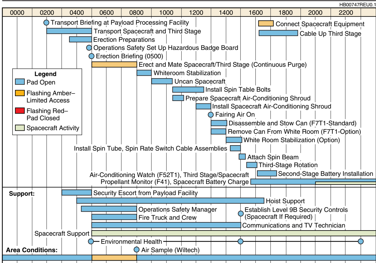
Figure 6-31. Typical Spacecraft Erection (T-7 Day)
