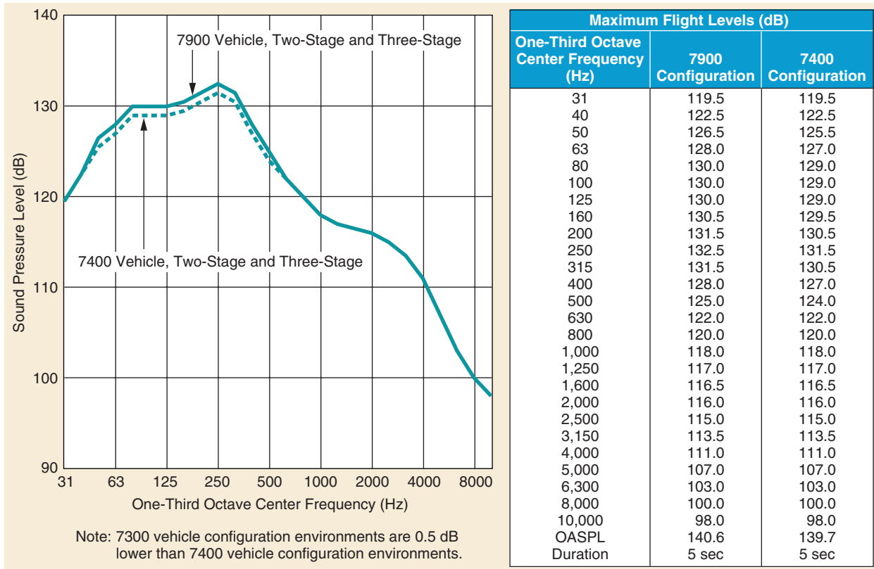
Figure 4-21. Predicted Delta II Acoustic Environments for 10-ft and -10L Fairing Missions
