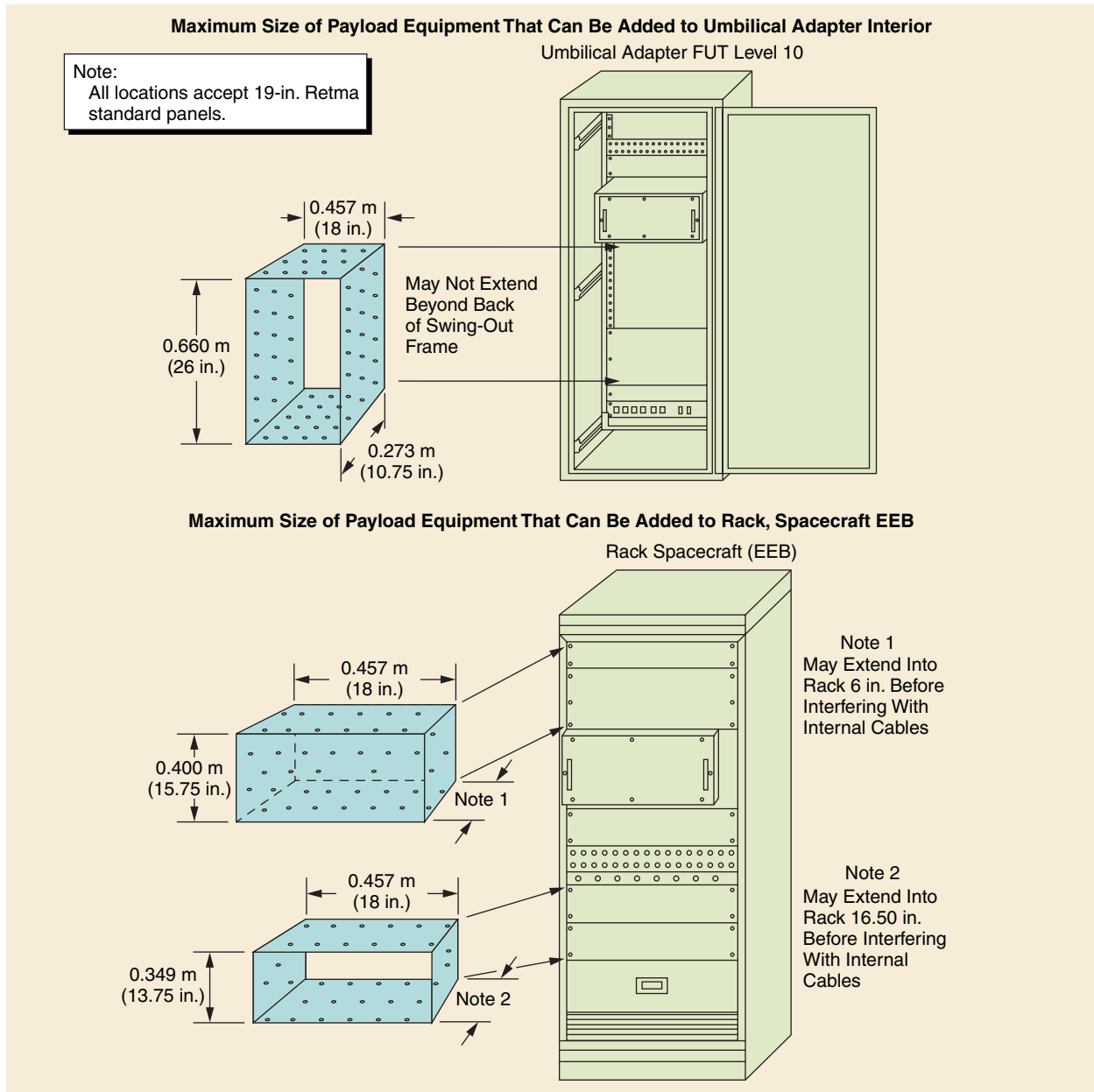
Figure 7-34. SLC-2
