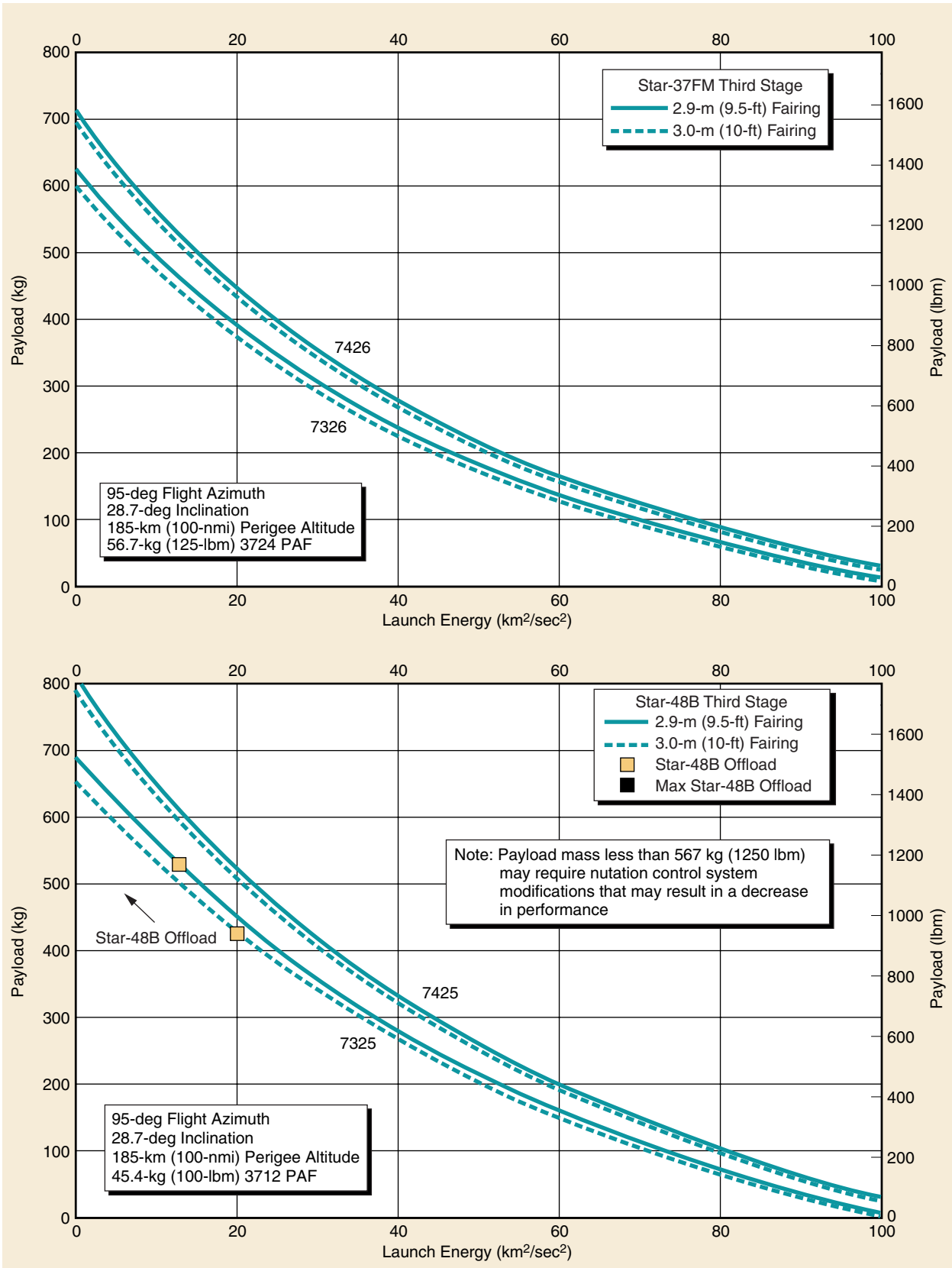
Figure 2-13. Delta II 732X/742X Vehicle, Three-Stage Launch Energy Capability—Eastern Launch Site
