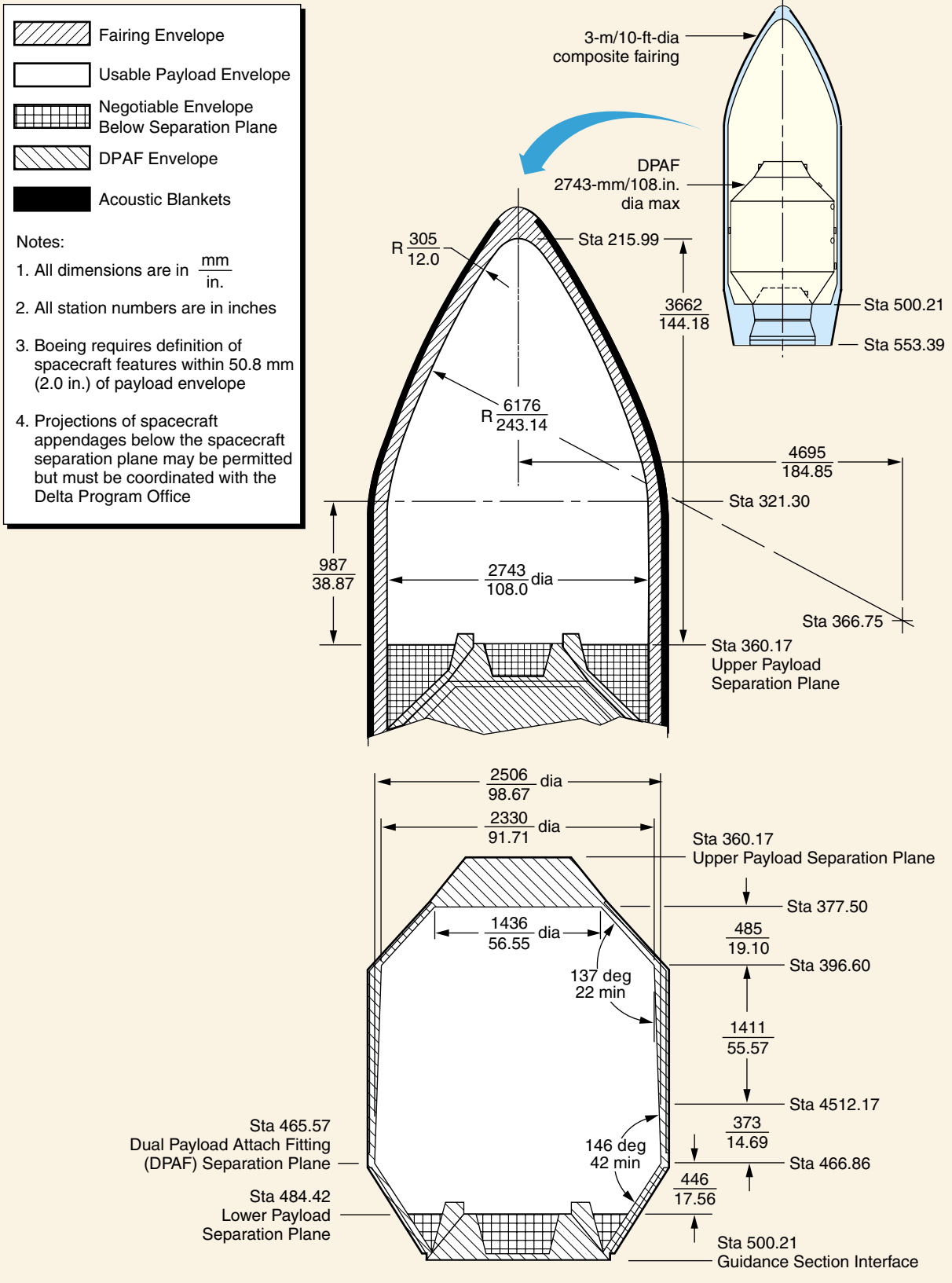
Figure 3-9. Maximum Payload Envelope for 3.0-m (10-ft)-dia Fairing, Dual-Payload Attach Fitting
