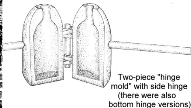
Figure 4. Two-Piece Mold 6
