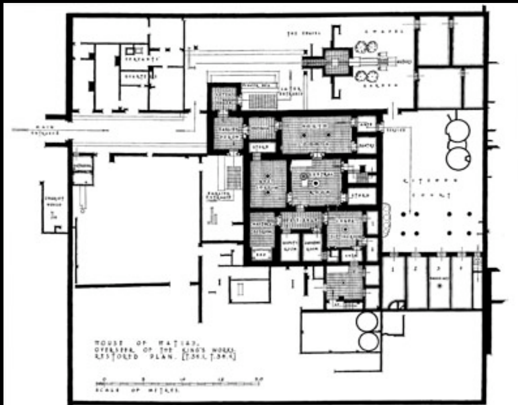
House of the Chief Builder, Hatia, North Suburb
