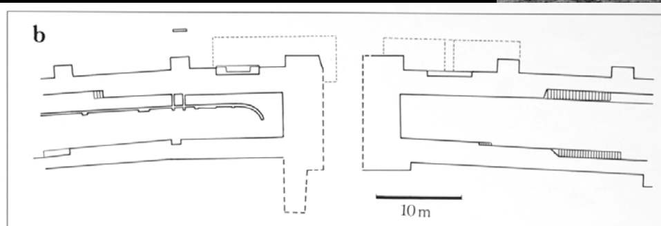
Fig. 118b. Detail of Gateway of North Riverside Palace. Dotted lines indicate reconstructed areas on plan (after unpublished drawing by B. Kemp).
