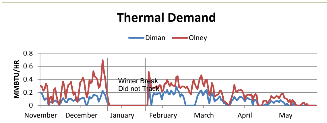
Figure 6: Diman and Olney average thermal consumption rate
