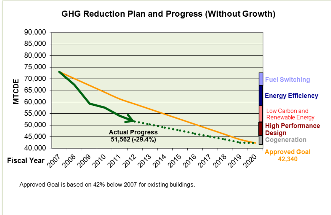
Figure 2: GHG Reduction Plan and Progress Without Growth
