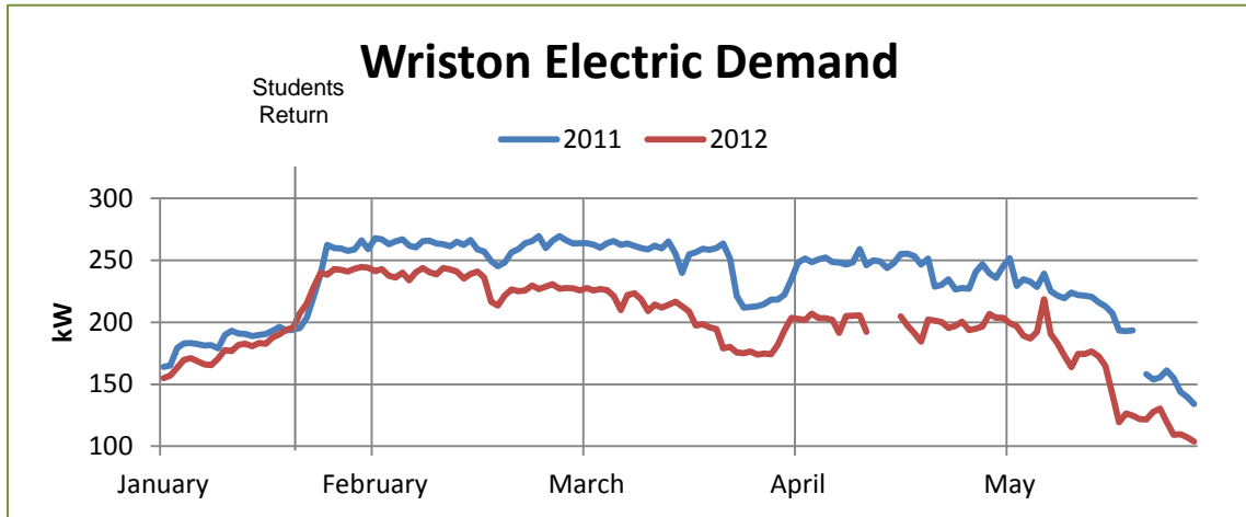
Figure 7: This graphic represents daily average electric load from January through May, 2011 and 2012.
