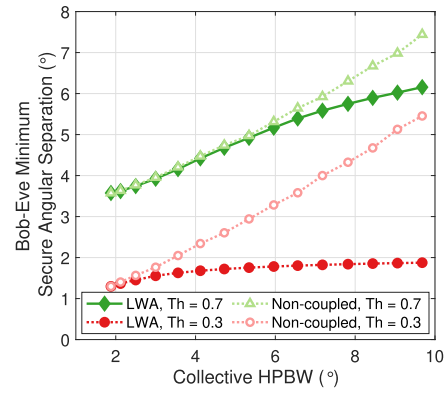
Fig. 9. Minimum angular separation between Bob and a positive-angle Eve required to achieve a certain normalized secrecy capacity as the transmission beamwidth increases due to increasing bandwidth, for two thresholds [0.3, 0.7]. The non-coupled baseline is a hypothetical link with the same collective radiation pattern that widens with bandwidth as the LWA link but has no frequency-angle coupling.
