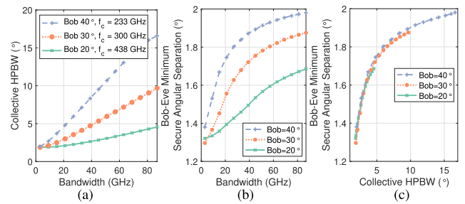
Fig. 11. (a) Collective HPBW and (b)(c) minimum angular separation between Bob and positive-angle Eve to achieve a normalized secrecy capacity of 0.3, for Bob at different angular locations.
