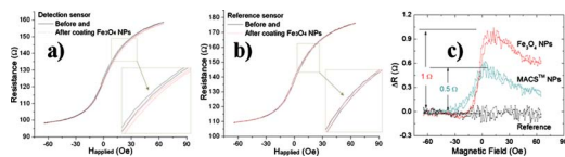
FIG. 3. (Color online) The MR transfer curves measured before and after the bonding of \text{Fe}_3\text{O}_4 NPs, (a) from an MTJ array treated with DNA and (b) from a nearby array without DNA treatment, meant as a reference. (c) Measured resistance differences for the detection sensors bonded with \text{Fe}_3\text{O}_4 and \text{MACS}^{\text{TM}} NPs, respectively, and for the reference sensor.
