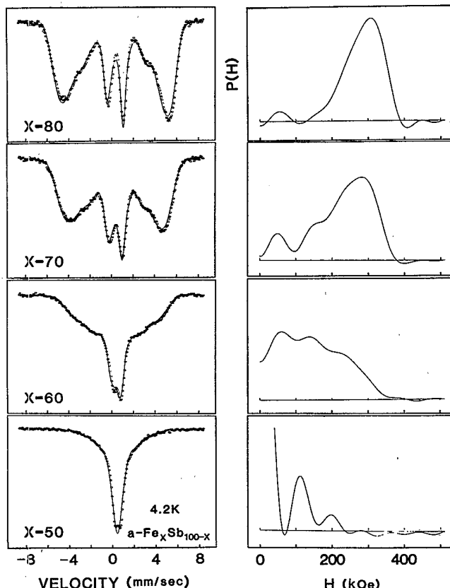
FIG. 2. Mössbauer spectra and deduced magnetic hyperfine field distribution of amorphous Fe-Sb alloys at 4.2 K.
