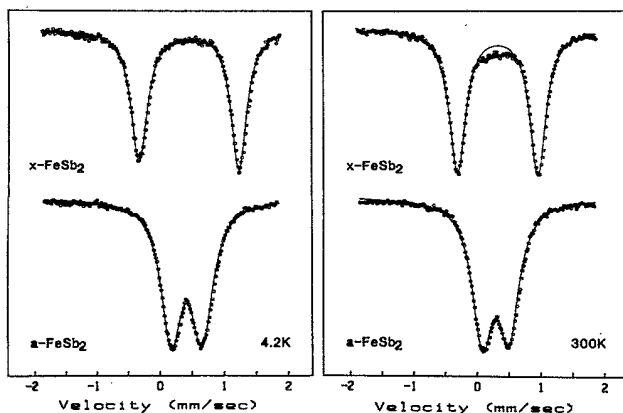
FIG. 6. Mössbauer spectra of amorphous FeSb 2 and crystalline FeSb 2 at 4.2 and 300 K.
