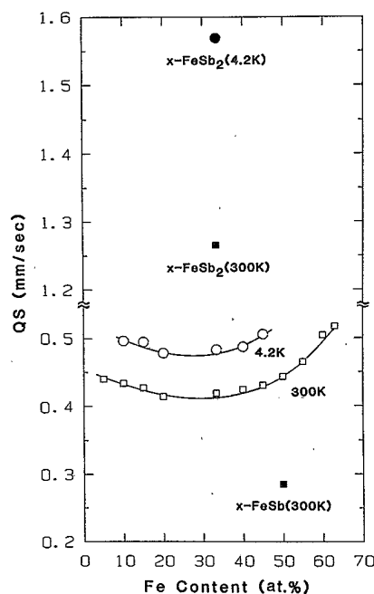
FIG. 5. Mean quadrupole splitting of amorphous Fe-Sb alloys as a function of Fe concentration at 4.2 and 300 K. Open squares and circles are data of amorphous samples and solid squares and circles are data of crystalline samples.
