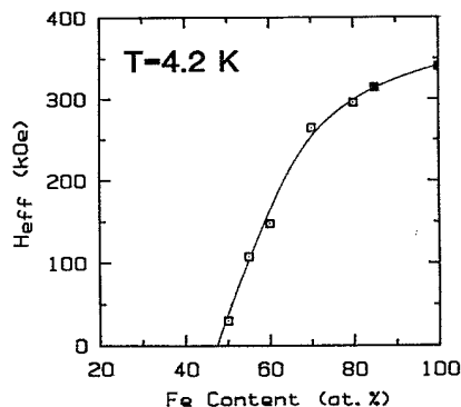
FIG. 11. Effective magnetic hyperfine fields of amorphous Fe-Sb and crystalline Fe-Sb alloys as a function of Fe concentration at 4.2 K.
