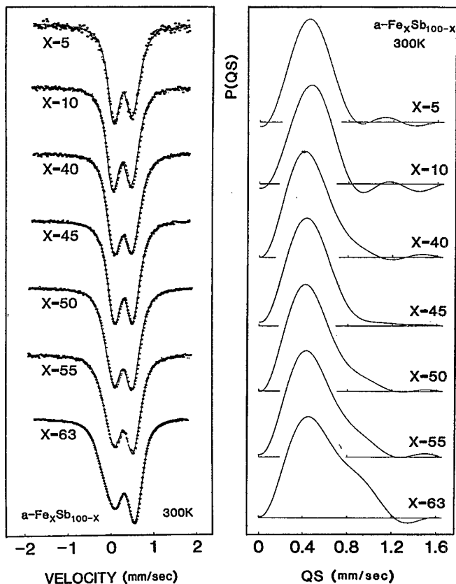
FIG. 1. Mössbauer spectra and deduced quadrupole splitting distribution P(QS) of amorphous Fe-Sb alloys at 300 K.
