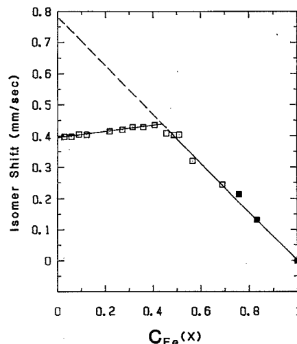
FIG. 4. Isomer shift of amorphous Fe-Sb alloys as a function of Fe surface-area concentration C_{\text{Fe}} defined in the text.
