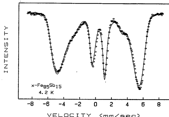
FIG. 9. Mössbauer spectrum of crystalline bcc \text{Fe}_{85}\text{Sb}_{15} at 4.2 K.
