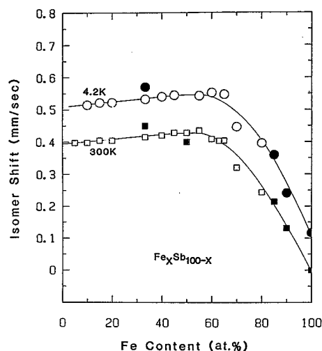
FIG. 3. Isomer shifts (relative to \alpha -Fe) of amorphous Fe x Sb 100-x alloys and some crystalline Fe-Sb samples at 4.2 and 300 K. Open squares and circles are data of amorphous samples and solid squares and circles are data of crystalline samples.
