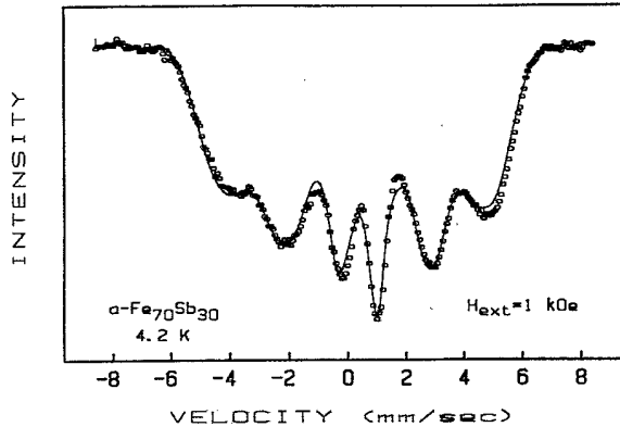
FIG. 10. Mössbauer spectrum of amorphous \text{Fe}_{70}\text{Sb}_{30} at 4.2 K with an external magnetic field of about 1 kOe applied in the sample plane.
