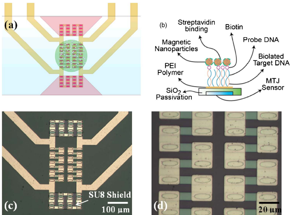
FIG. 1. (Color online) (a) Schematic image of the 64-element MTJ array. The 120\ \mu\text{m} diameter green spot is the biologically active area which contains all of the active MTJ sensors. The pink area indicates the regions of photoreist which shield the reference arms of the Wheatstone bridge. (b) Schematic of the surface treatment used for the MTJ biosensor array. (c) Optical image of the 64-element MTJ biosensor device. (d) A close-up view of the active arms of the array, each of which contains 16 MTJ sensors.
