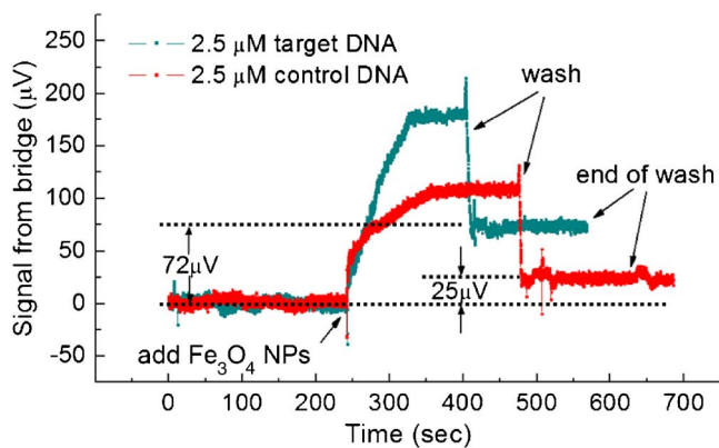
FIG. 3. (Color online) Real-time detection data of 2.5 \mu\text{M} target DNA (dark cyan curve) and 2.5 \mu\text{M} control DNA (red curve) by the MTJ biosensor.
