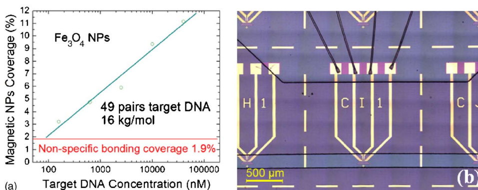
FIG. 2. (Color online) (a) Semilogarithmic graph plotting the coverage of \text{Fe}_3\text{O}_4 NPs vs the concentration of target DNA. (b) A 300\ \mu\text{m} wide microfluidic channel sealed on the MTJ bridge array chip.
